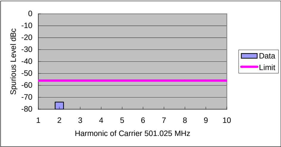
Figure 6F-5: 4.5 Watt Harmonic of Carrier 501.025 MHz, 12.5 kHz Channel Spacing
