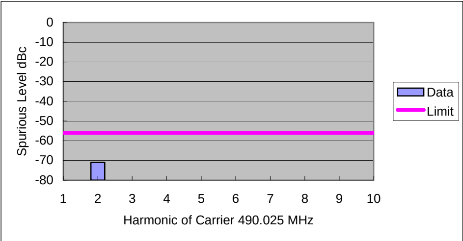
Figure 6F-4: 4.5 Watt Harmonic of Carrier 490.025 MHz, 12.5 kHz Channel Spacing
