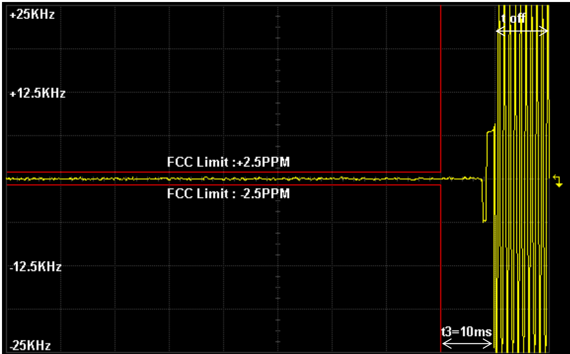
Figure 6I-4: 4 Watts, 25 kHz, 501.025 MHz, De-Key Decay Time
