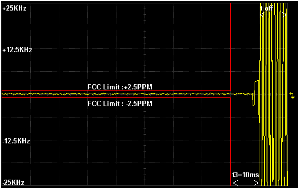
Figure 6I-6: 1 Watt, 12.5 kHz, 501.025 MHz, De-Key Decay Time
