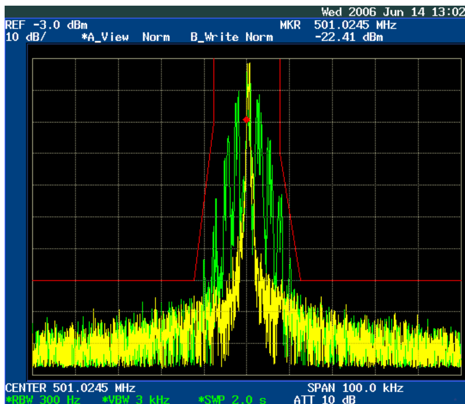
Figure 6E-3: 12.5 kHz Channel Spacing, 501.025 MHz, 2500 Hz Audio and DPL Tone Modulation, Mask D 11K0F3E
