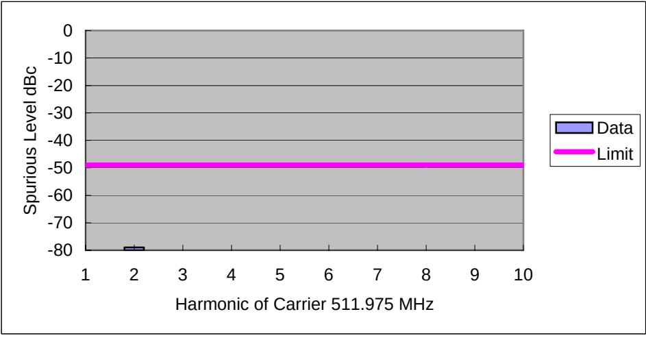
Figure 6F-12: 4.5 Watt Harmonic of Carrier 511.975 MHz, 25 kHz Channel Spacing
