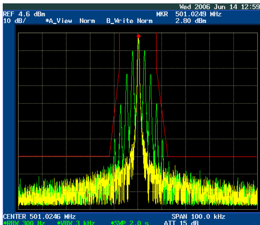
Figure 6E-1: 12.5 kHz Channel Spacing, 501.025 MHz, 2500 Hz Audio Modulation Only, Mask D 11K0F3E
