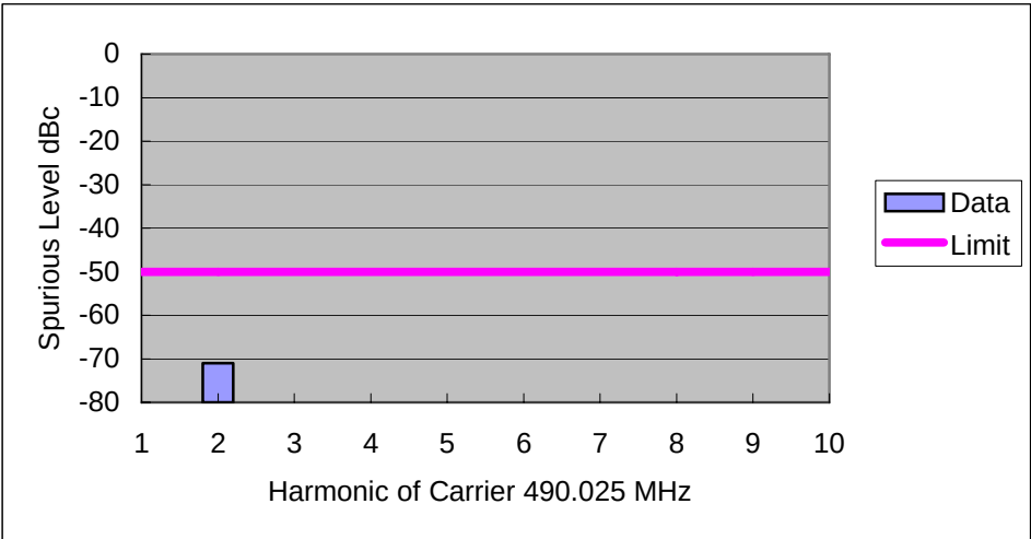
Figure 6F-1: 1 Watt Harmonic of Carrier 490.025 MHz, 12.5 kHz Channel Spacing
