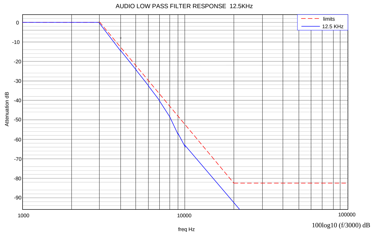
Figure 6C-1: 12.5 kHz Channel Spacing, 501.025 MHz, Transmit Audio Lowpass Filter Response
