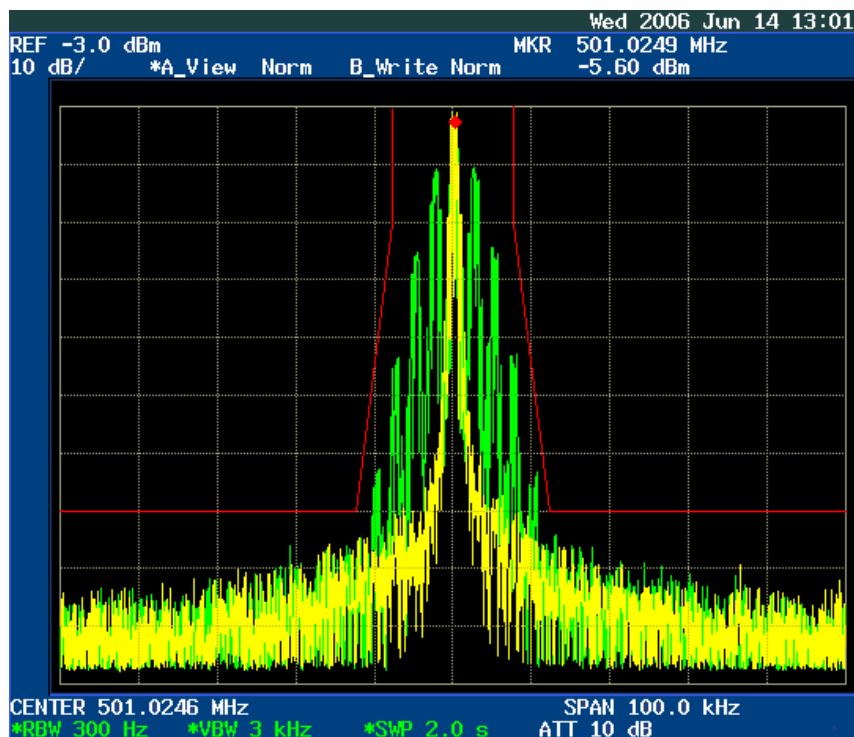
Figure 6E-2: 12.5 kHz Channel Spacing, 501.025 MHz, 2500 Hz Audio and PL Tone Modulation, Mask D 11K0F3E
