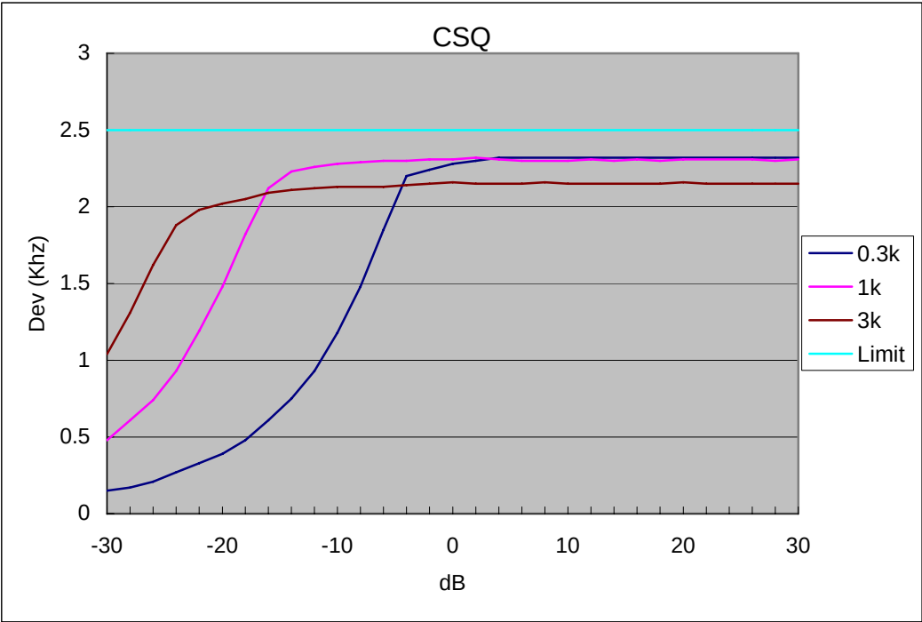
Figure 6D-1: 12.5 kHz Channel Spacing, 501.025 MHz, Carrier Squelch (CSQ) Mode
