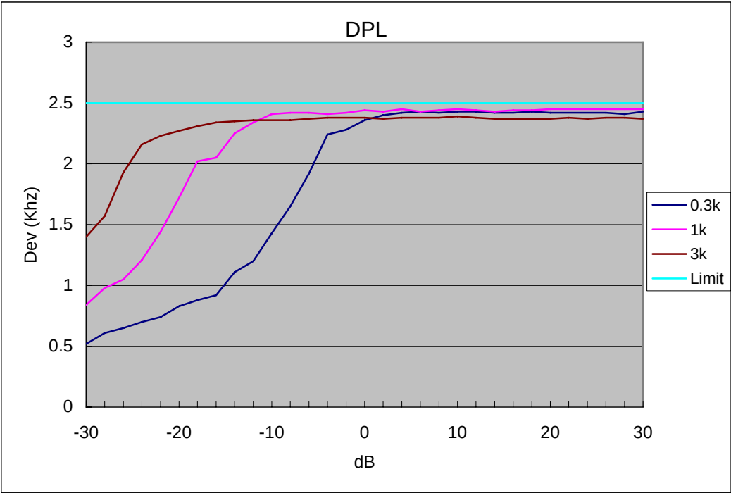
Figure 6D-3: 12.5 kHz Channel Spacing, 501.025 MHz, Digital Private Line (DPL) Mode
