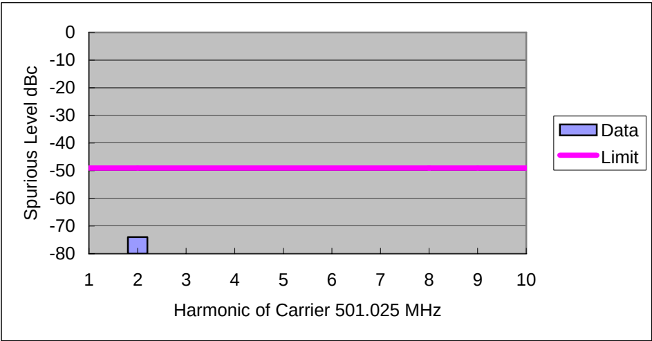
Figure 6F-11: 4.5 Watt Harmonic of Carrier 501.025 MHz, 25 kHz Channel Spacing
