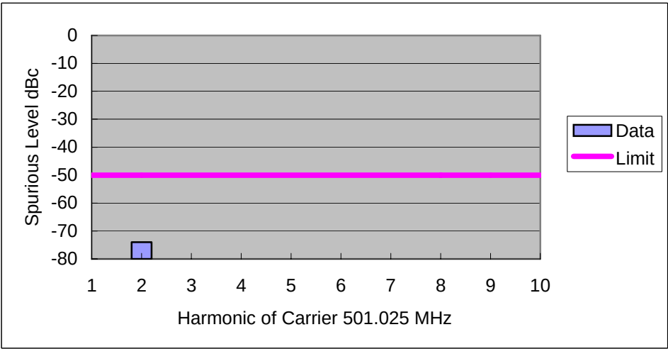
Figure 6F-2: 1 Watt Harmonic of Carrier 501.025 MHz, 12.5 kHz Channel Spacing
