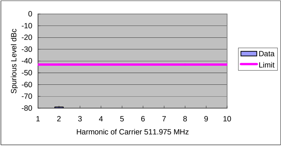
Figure 6F-9: 1 Watt Harmonic of Carrier 511.975 MHz, 25 kHz Channel Spacing
