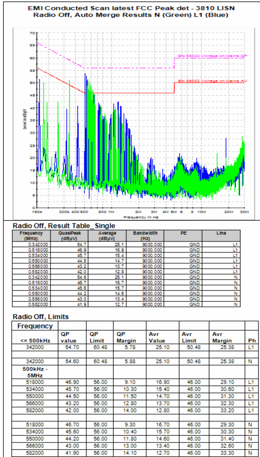
Figure 6J-1: Radio off Line/Neutral
