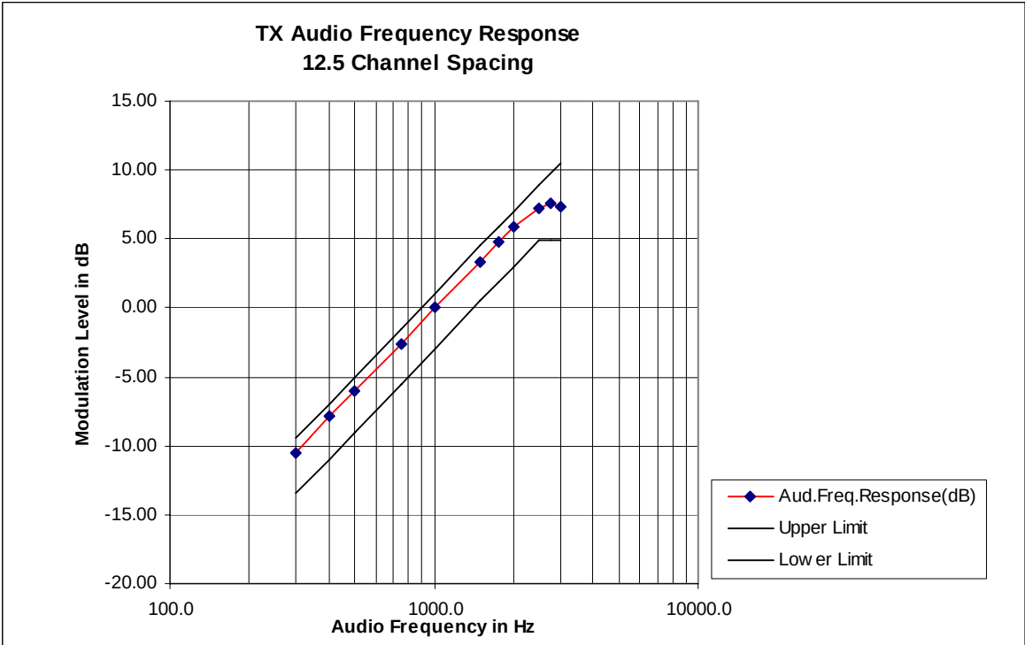
Figure 6B-1: 12.5 kHz Channel Spacing, 501.025 MHz, Transmit Audio Frequency Response
