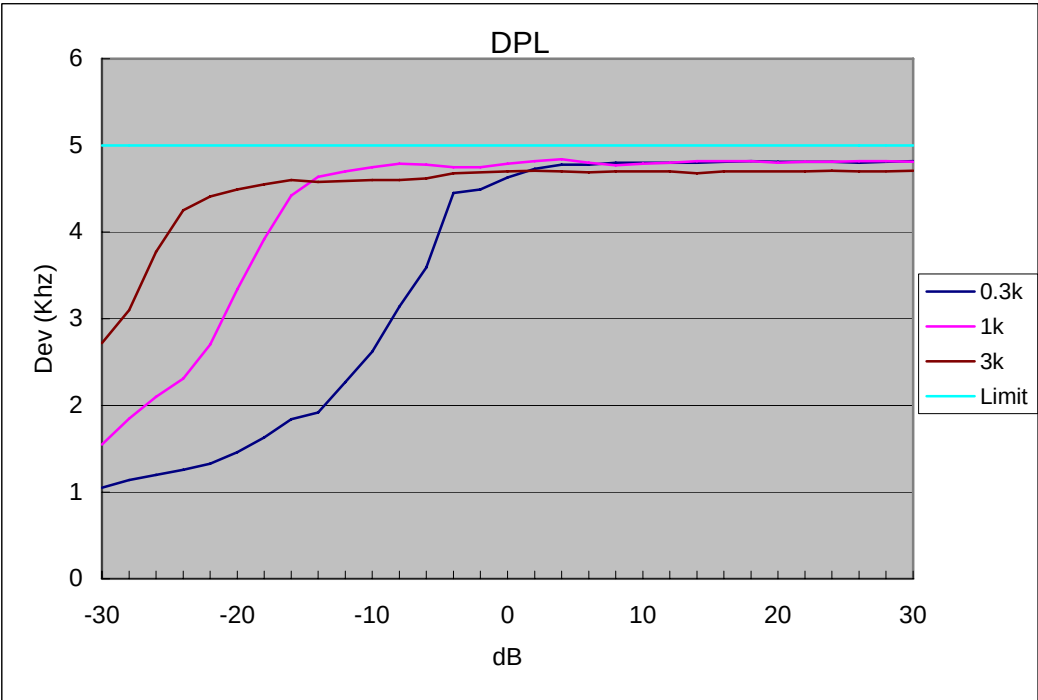
Figure 6D-6: 25 kHz Channel Spacing, 501.025 MHz, Digital Private Line (DPL) Mode
