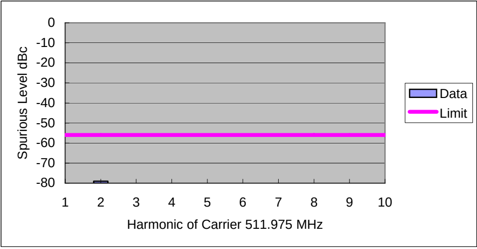
Figure 6F-6: 4.5 Watt Harmonic of Carrier 511.975 MHz, 12.5 kHz Channel Spacing
