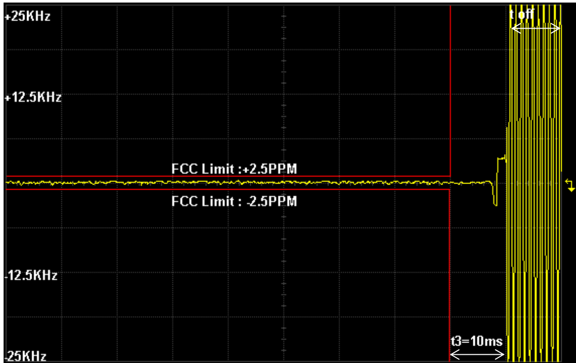
Figure 6I-2: 4 Watts, 12.5 kHz, 501.025 MHz, De-Key Decay Time
