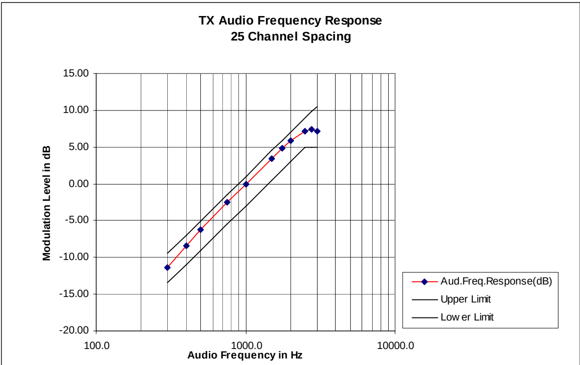
Figure 6B-2: 25 kHz Channel Spacing, 501.025 MHz, Transmit Audio Frequency Response
