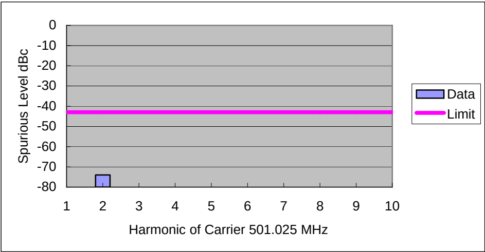
Figure 6F-8: 1 Watt Harmonic of Carrier 501.025 MHz, 25 kHz Channel Spacing
