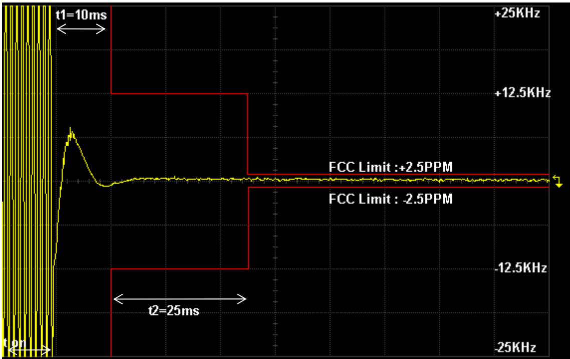
Figure 6I-3: 4 Watts, 25 kHz, 501.025 MHz, Key-Up Attack Time
