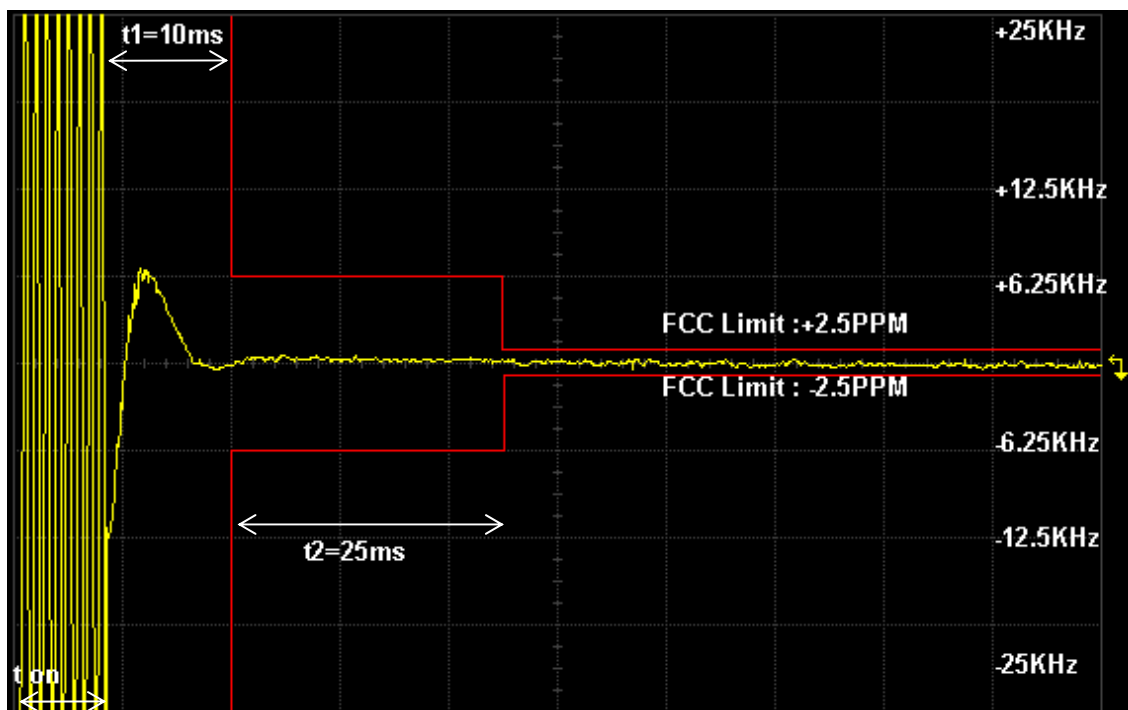
Figure 6I-1: 4 Watts, 12.5 kHz, 501.025 MHz, Key-Up Attack Time
