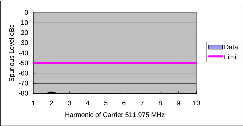
Figure 6F-3: 1 Watt Harmonic of Carrier 511.975 MHz, 12.5 kHz Channel Spacing
