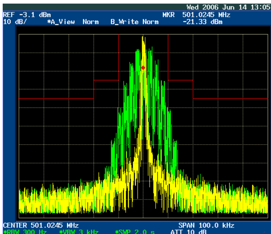
Figure 6E-5: 25 kHz Channel Spacing, 501.025 MHz, 2500 Hz Audio and PL Tone Modulation, Mask B 16K0F3E
