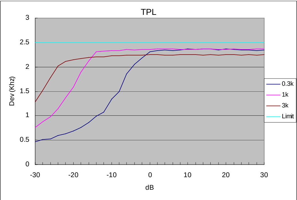
Figure 6D-2: 12.5 kHz Channel Spacing, 501.025 MHz, Tone Private Line (TPL) Mode
