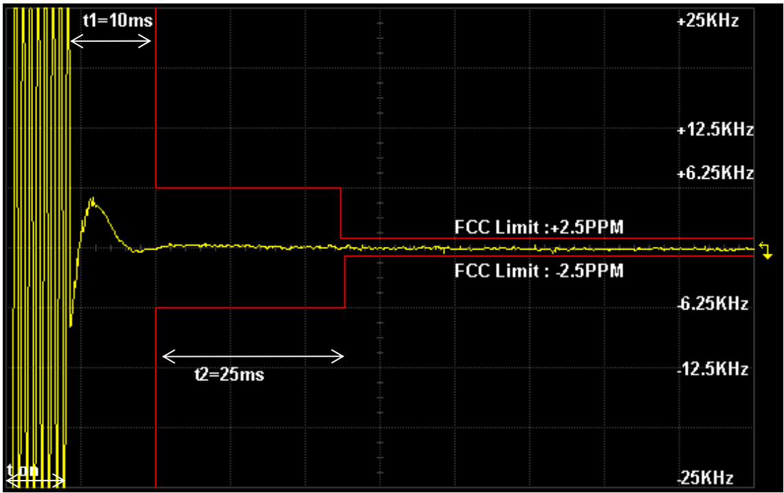
Figure 6I-5: 1 Watt, 12.5 kHz, 501.025 MHz, Key-Up Attack Time
