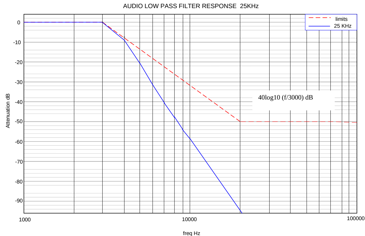
Figure 6C-2: 25 kHz Channel Spacing, 501.025 MHz, Transmit Audio Low pass Filter Response
