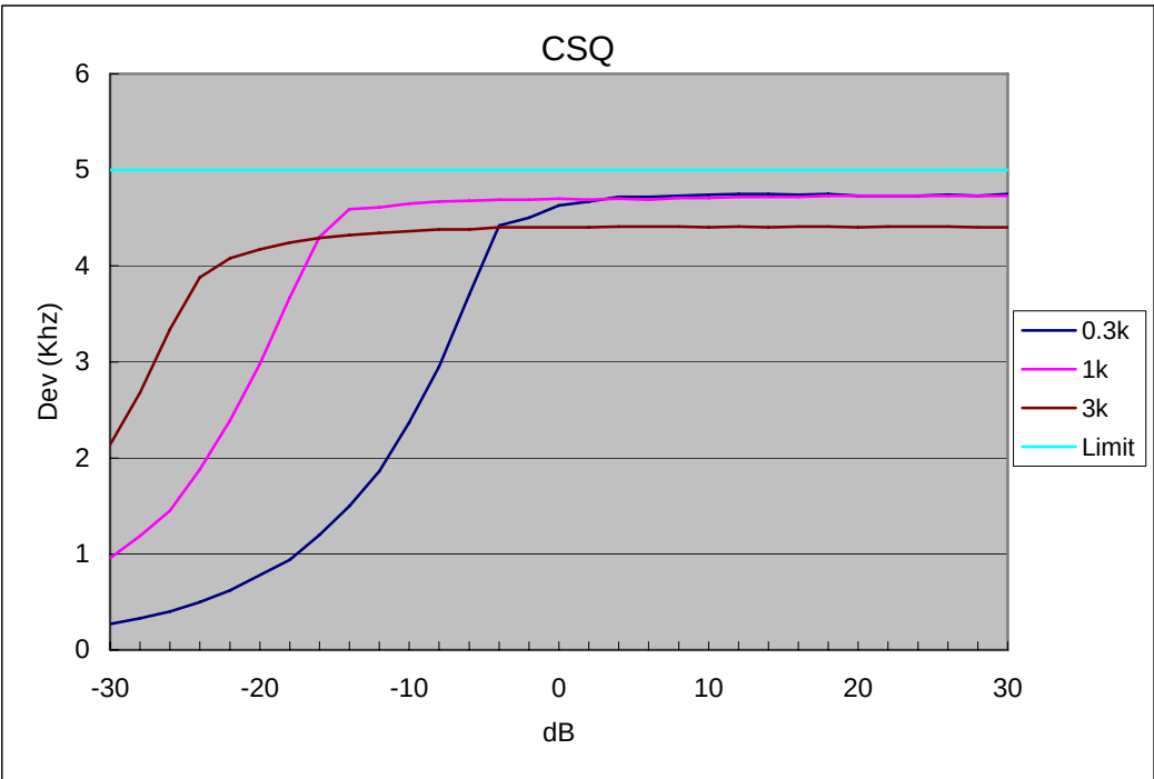
Figure 6D-4: 25 kHz Channel Spacing, 501.025 MHz, Carrier Squelch (CSQ) Mode
