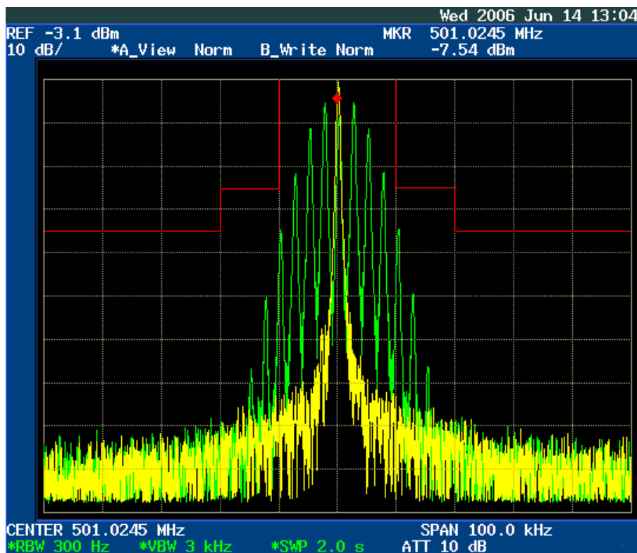
Figure 6E-4: 25 kHz Channel Spacing, 501.025 MHz, 2500 Hz Audio Modulation Only, Mask B 16K0F3E
