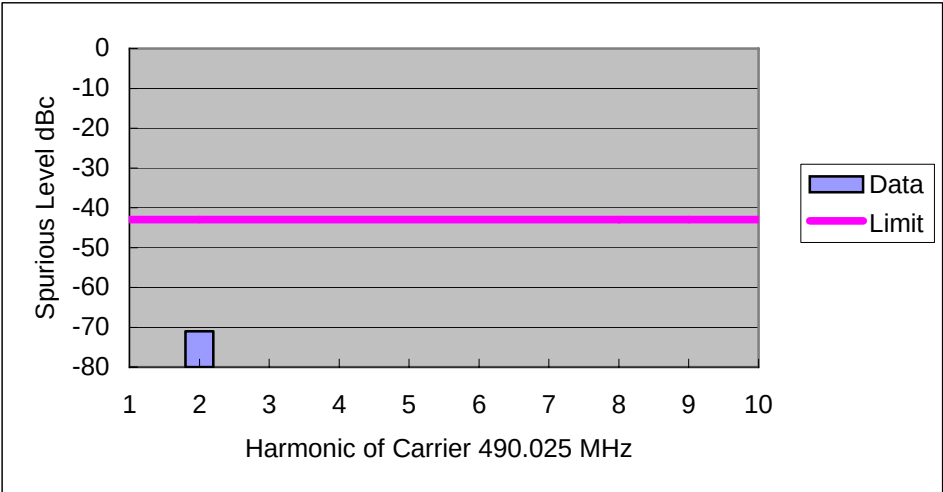
Figure 6F-7: 1 Watt Harmonic of Carrier 490.025 MHz, 25 kHz Channel Spacing
