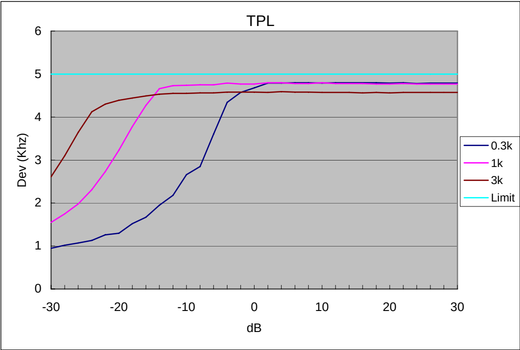
Figure 6D-5: 25 kHz Channel Spacing, 501.025 MHz, Tone Private Line (TPL) Mode
