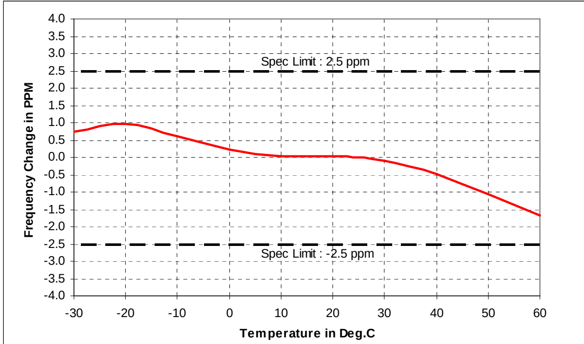
Figure 6H-1: Frequency Stability vs. Temperature
