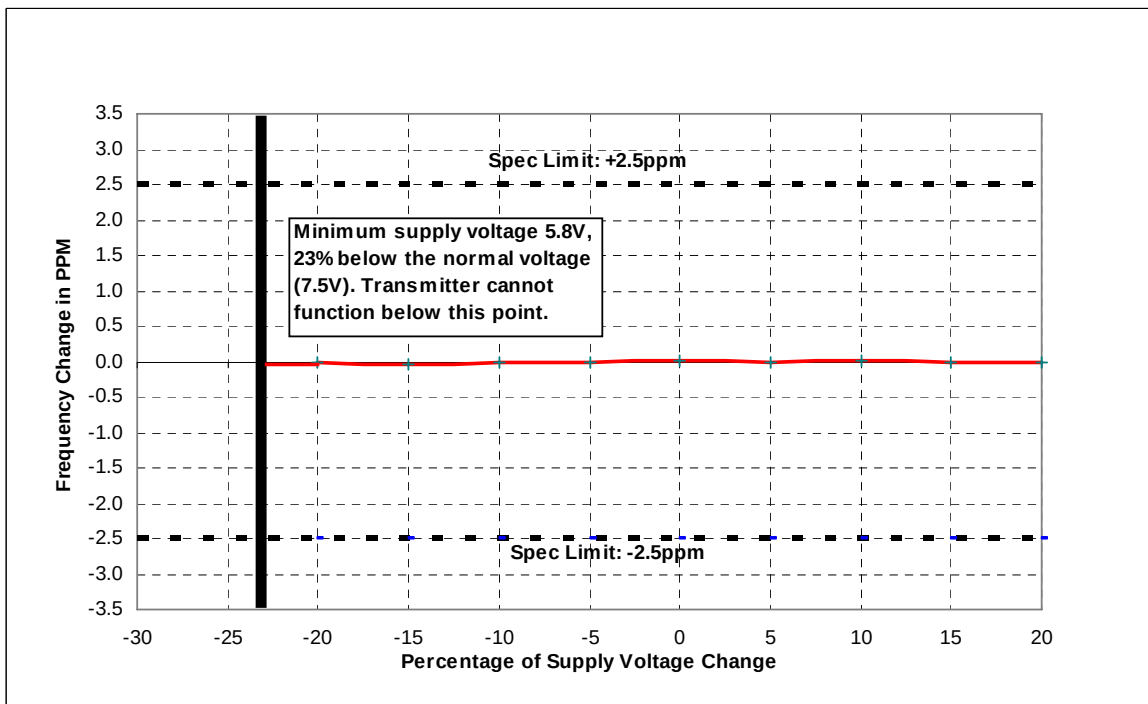
Figure 6H-2: Frequency Stability vs. Supply Voltage
