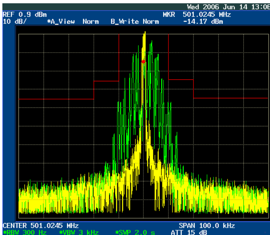
Figure 6E-6: 25 kHz Channel Spacing, 501.025 MHz, 2500 Hz Audio and DPL Tone Modulation, Mask B 16K0F3E
