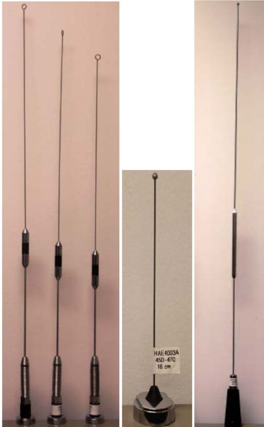
UHF Antenna kit numbers, from left to right: HAE4011A, HAE4012A, HAE4013A, HAE4003A, HAE4004A
