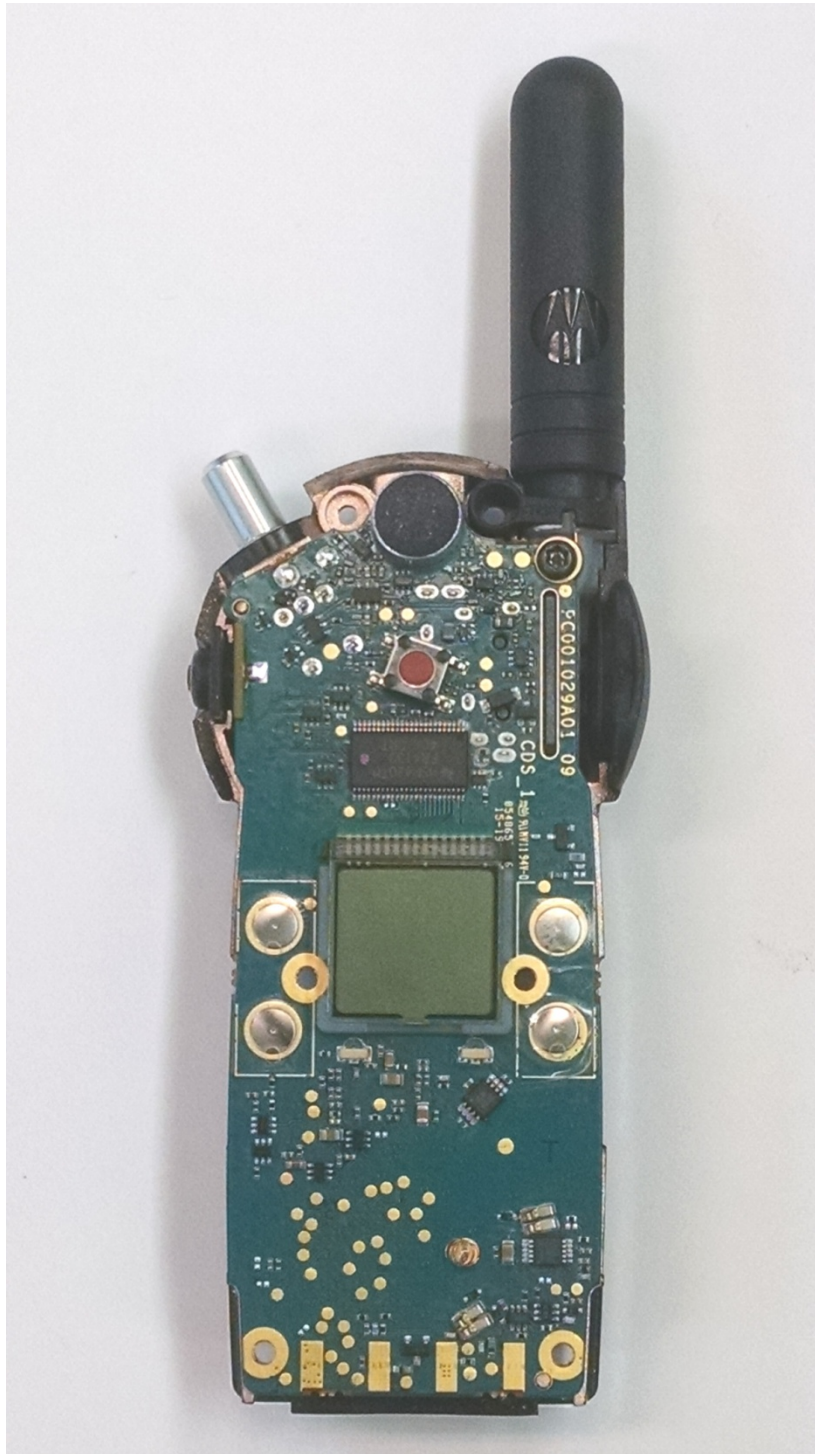
Figure 9-8 Board Assembly
