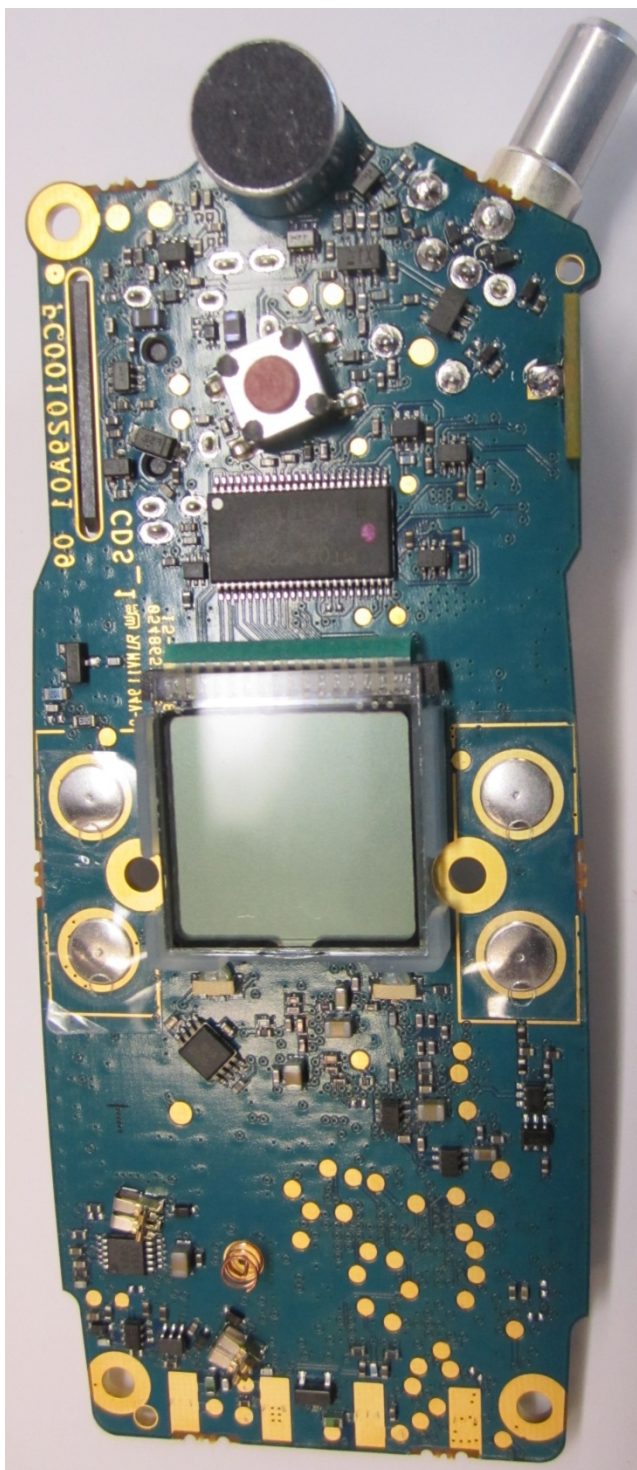
Figure 9-1 Internal Top Side Photo.
