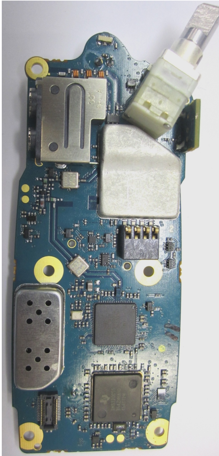
Figure 9-2 Internal Bottom Side Photo with Shields.
