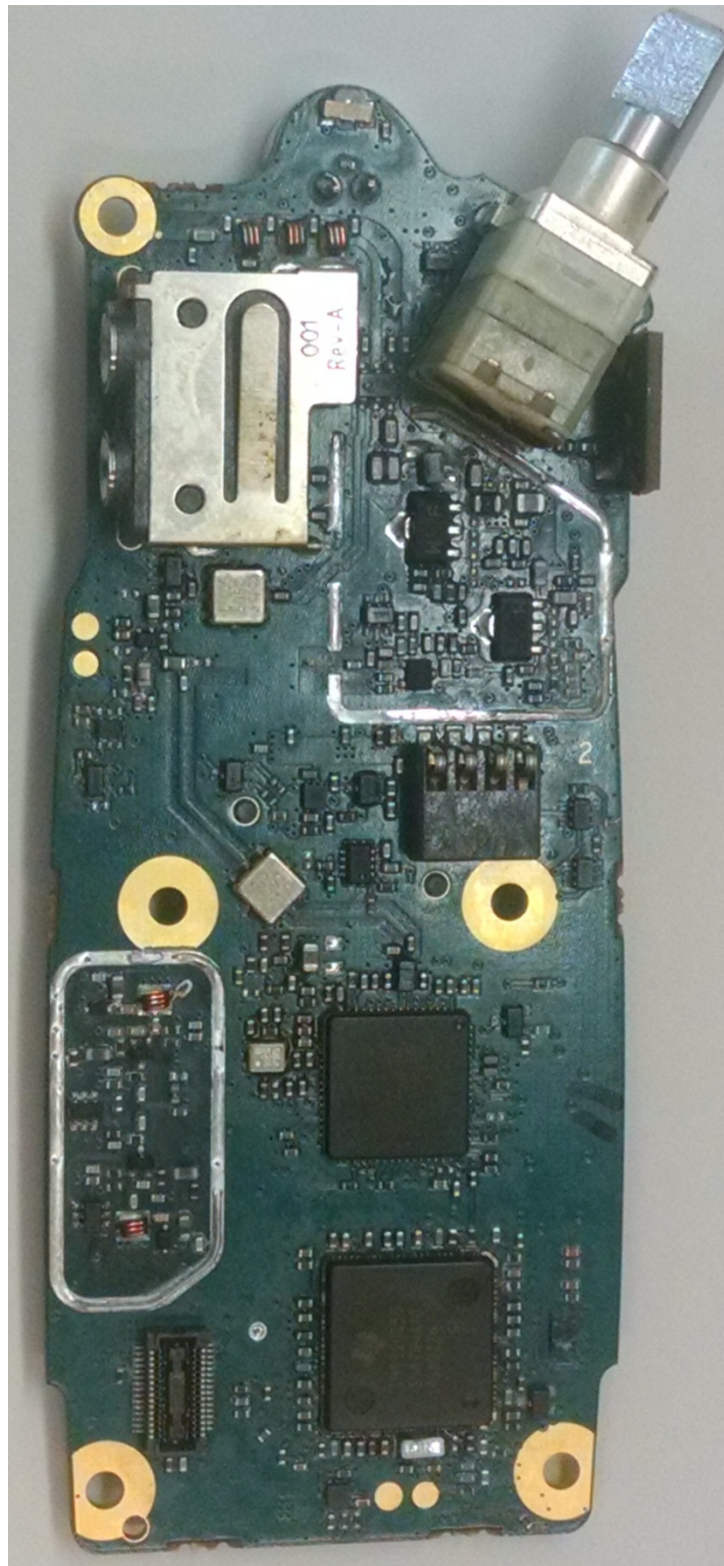
Figure 9-3 Internal Bottom Side Photo without Shields.
