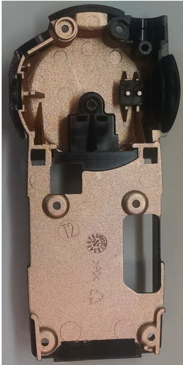
Figure 9-6 Back Housing
