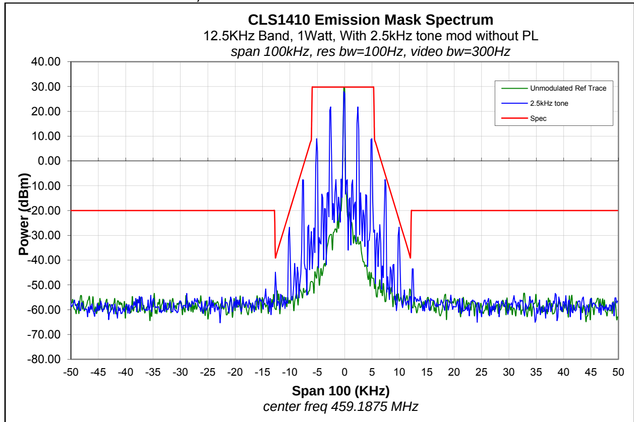
Figure 6C-6: 459.1875 MHz Emission Mask Spectrum without PL
