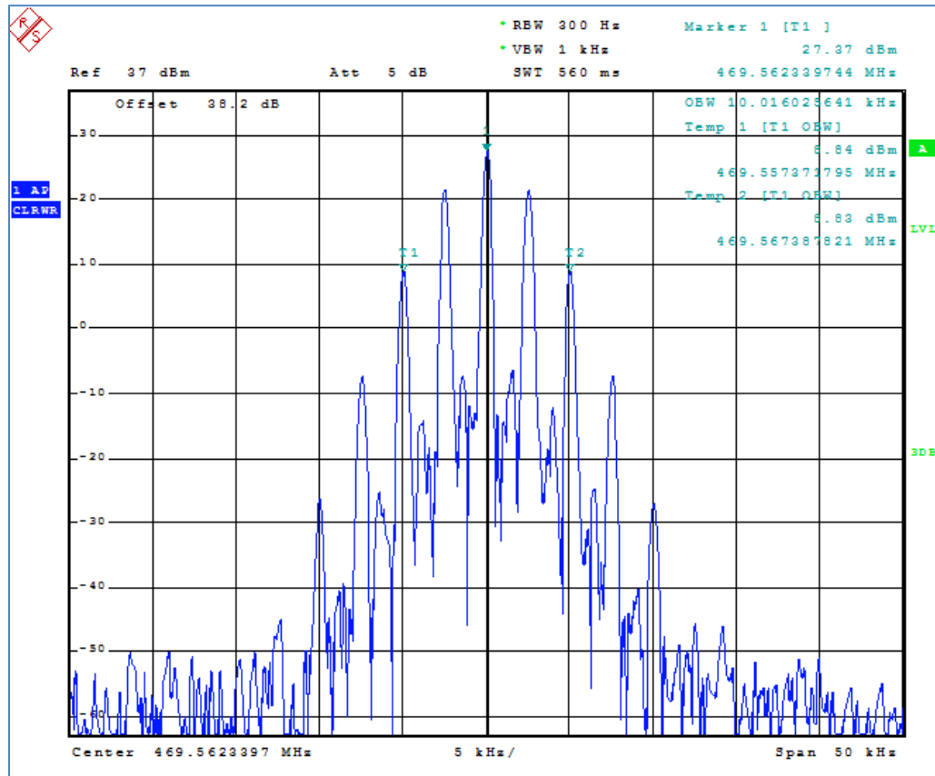
Figure 6C-3: 469.5625 MHz occupied bandwidth
