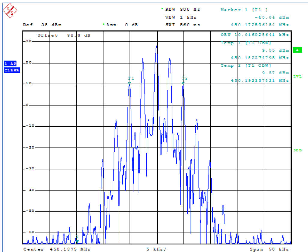
Figure 6C-1: 450.1875 MHz channel occupied bandwidth
