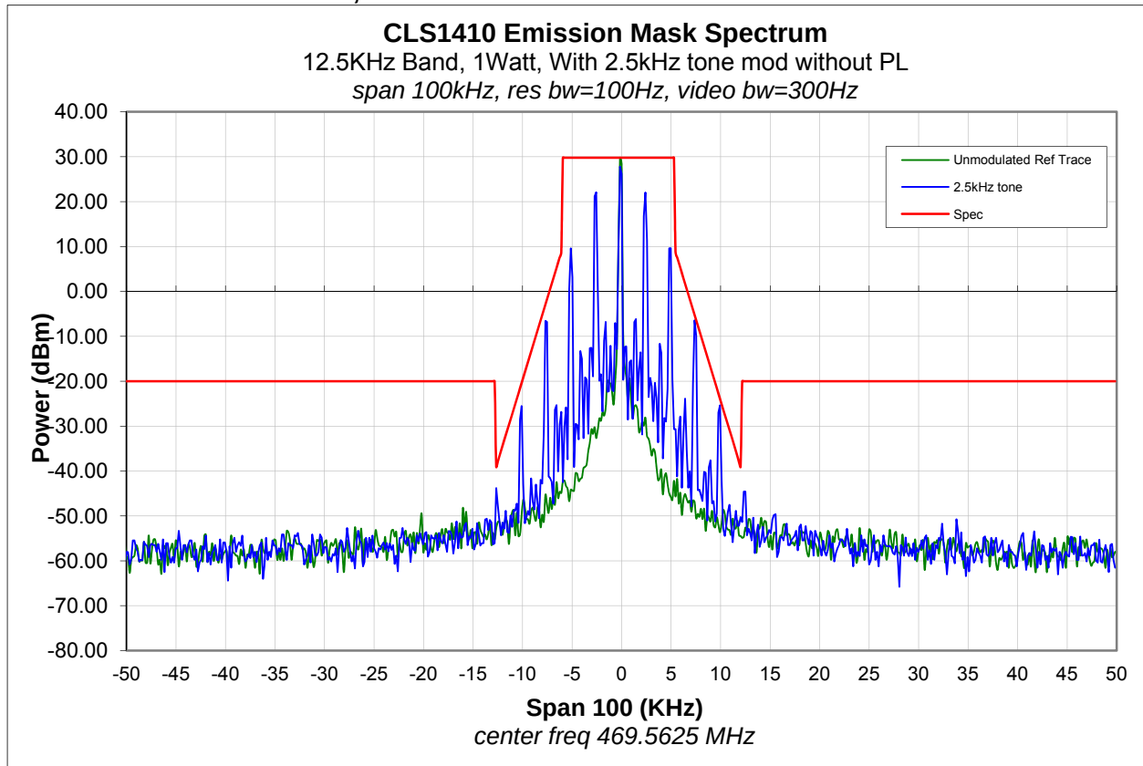
Figure 6C-8: 469.5625 MHz Emission Mask Spectrum without PL
