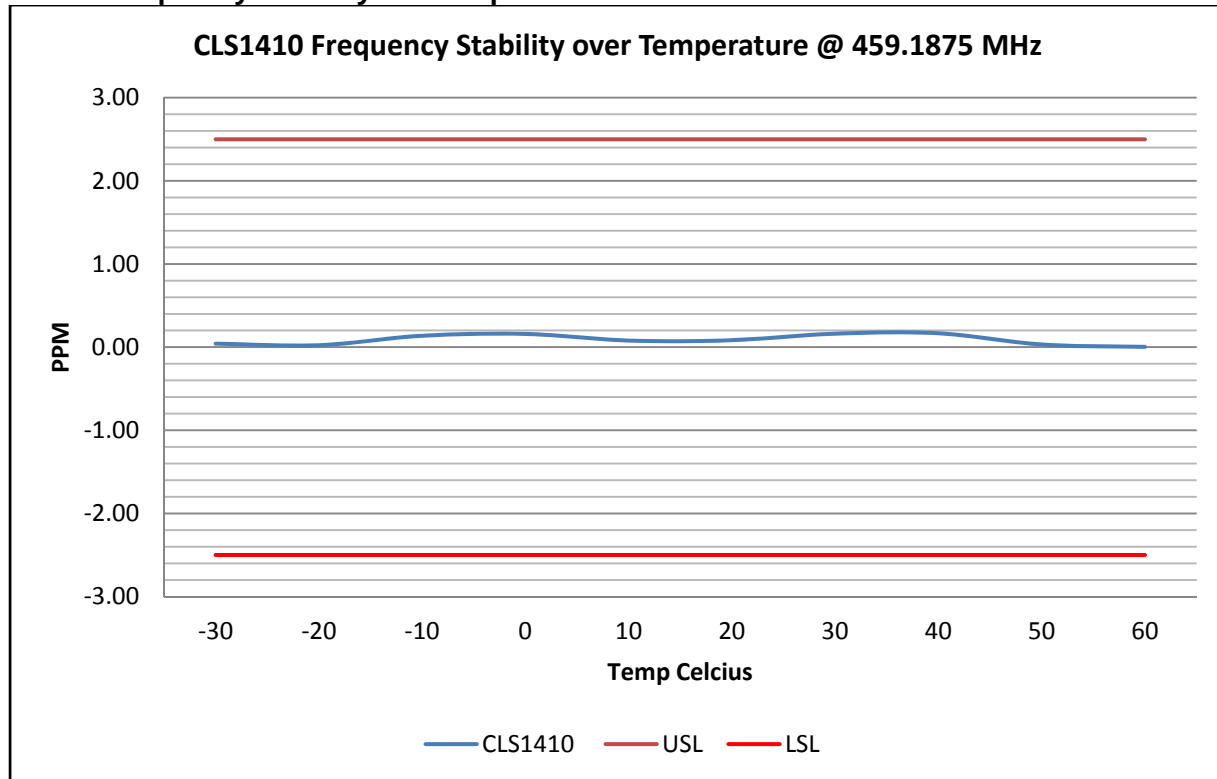
Figure 6E-1: Frequency Stability over Temperature
