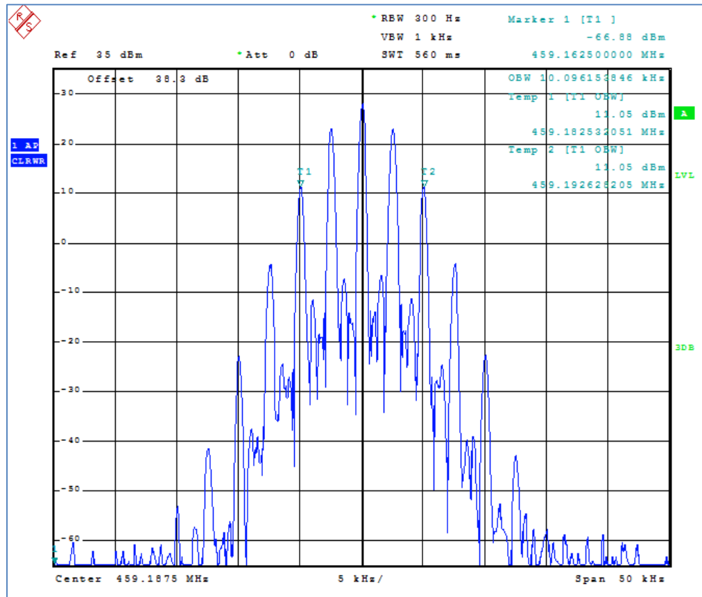
Figure 6C-2: 459.1875 MHz channel occupied bandwidth
