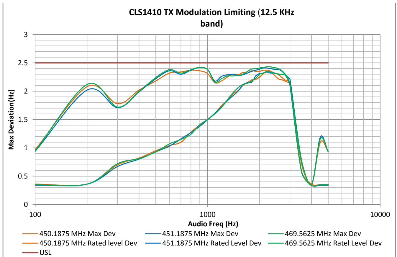
Figure 6B-1: Modulation limiting for 12.5 KHz band.
