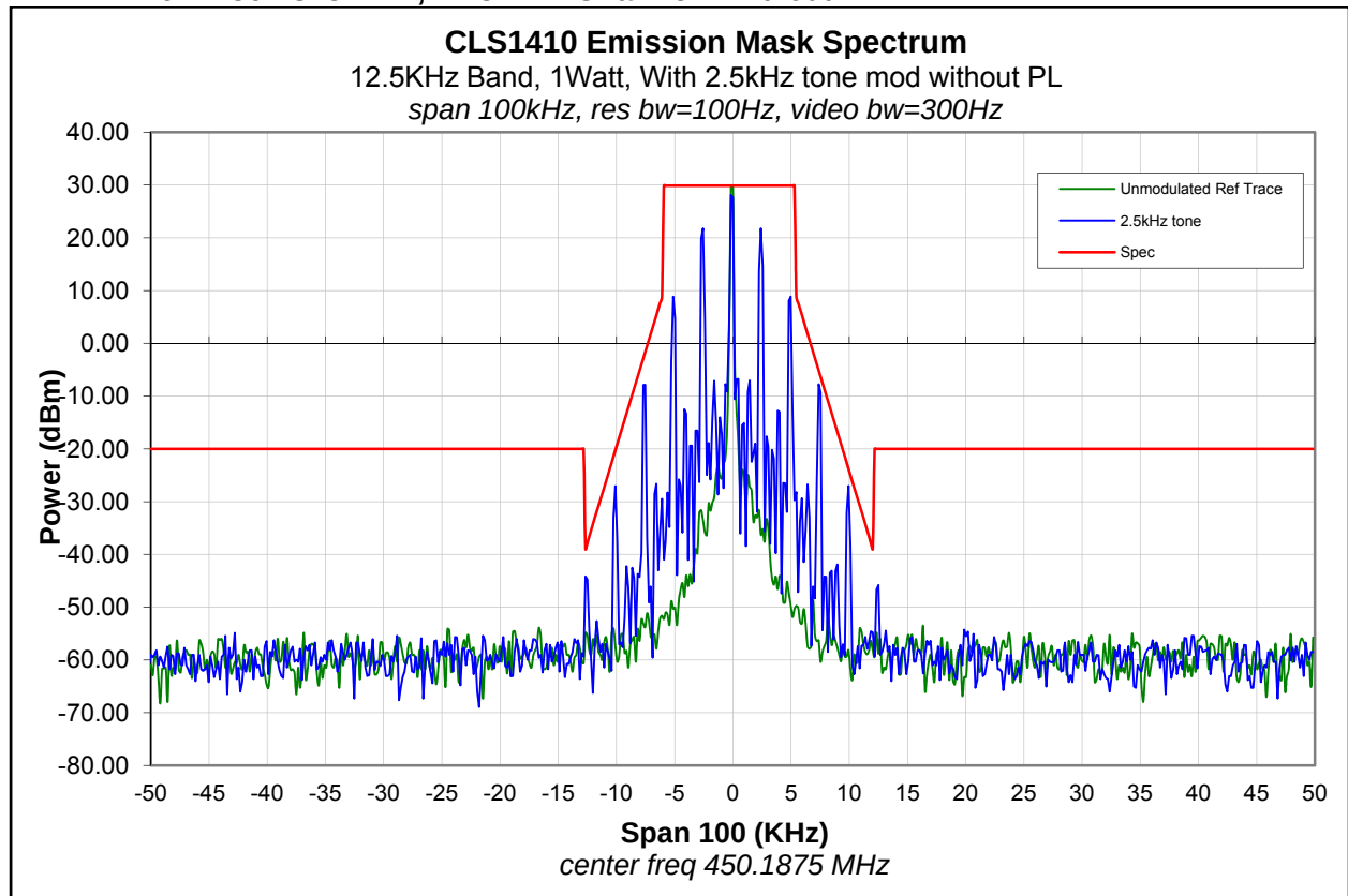
Figure 6C-4: 450.1875 MHz Emission Mask Spectrum without PL
