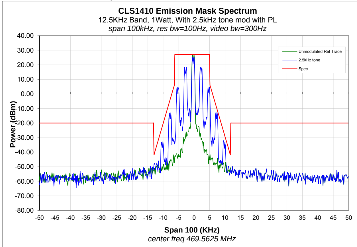
Figure 6C-9: 469.5625 MHz Emission Mask Spectrum with PL
