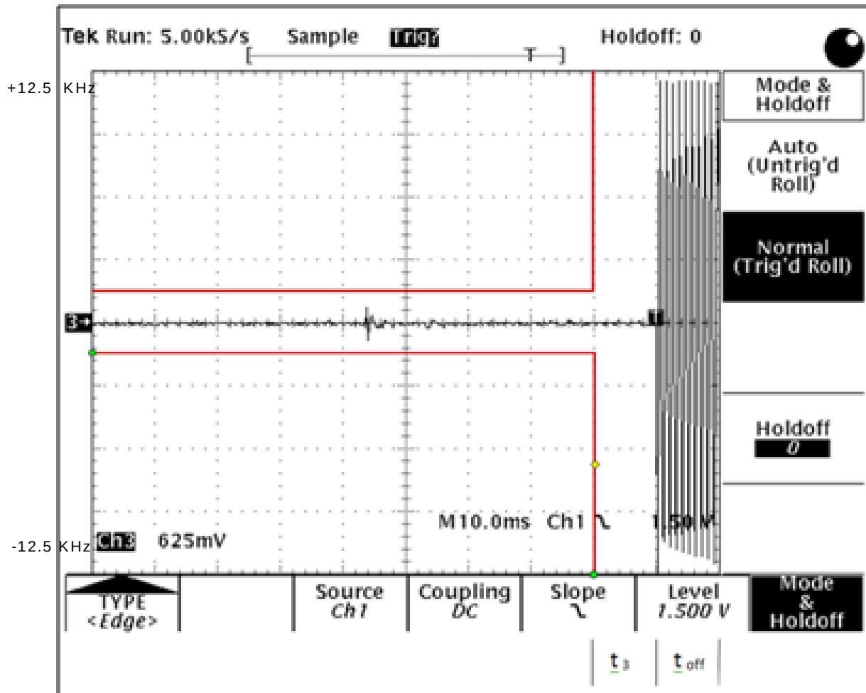
Figure 6F-2: Transient Frequency Behavior On to Off
