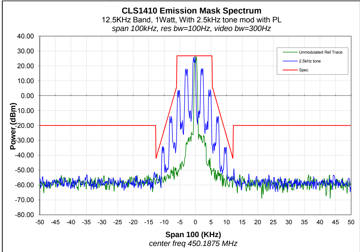
Figure 6C-5: 450.1875 MHz Emission Mask Spectrum with PL
