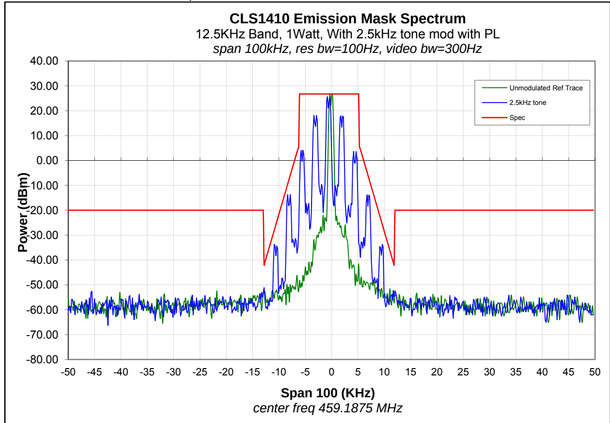
Figure 6C-7: 459.1875 MHz Emission Mask Spectrum with PL
