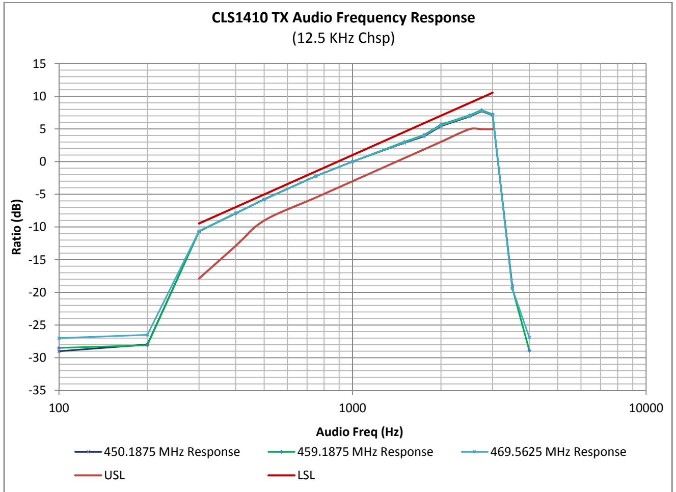
Figure 6B-2: Audio Response for 12.5 KHz band.
