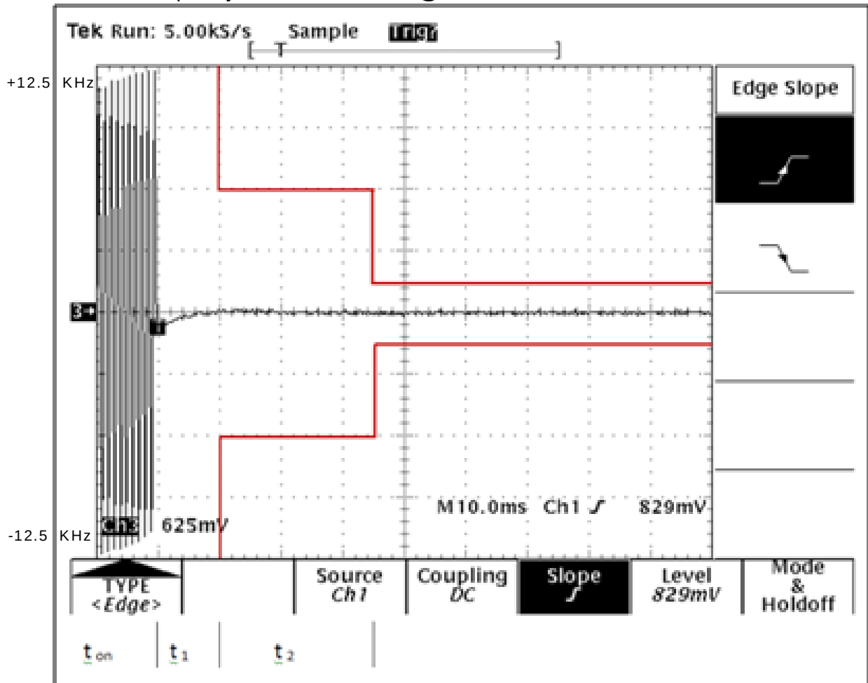
Figure 6F-1: Transient Frequency Behavior Off to On
