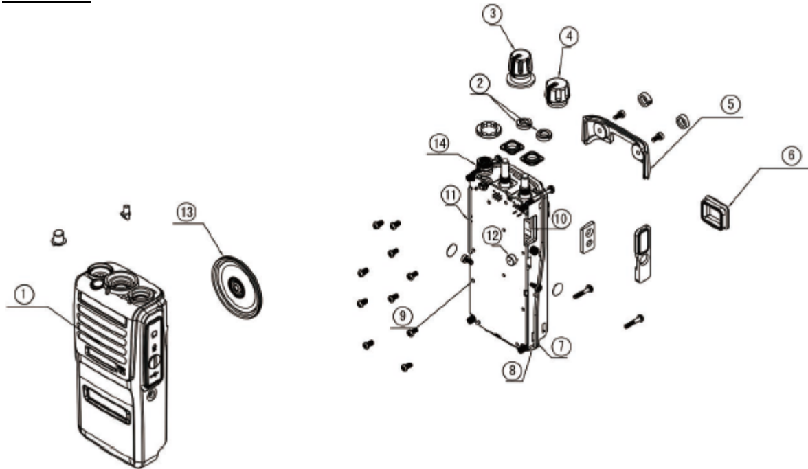
Exploded View of Radio (BC250D)
