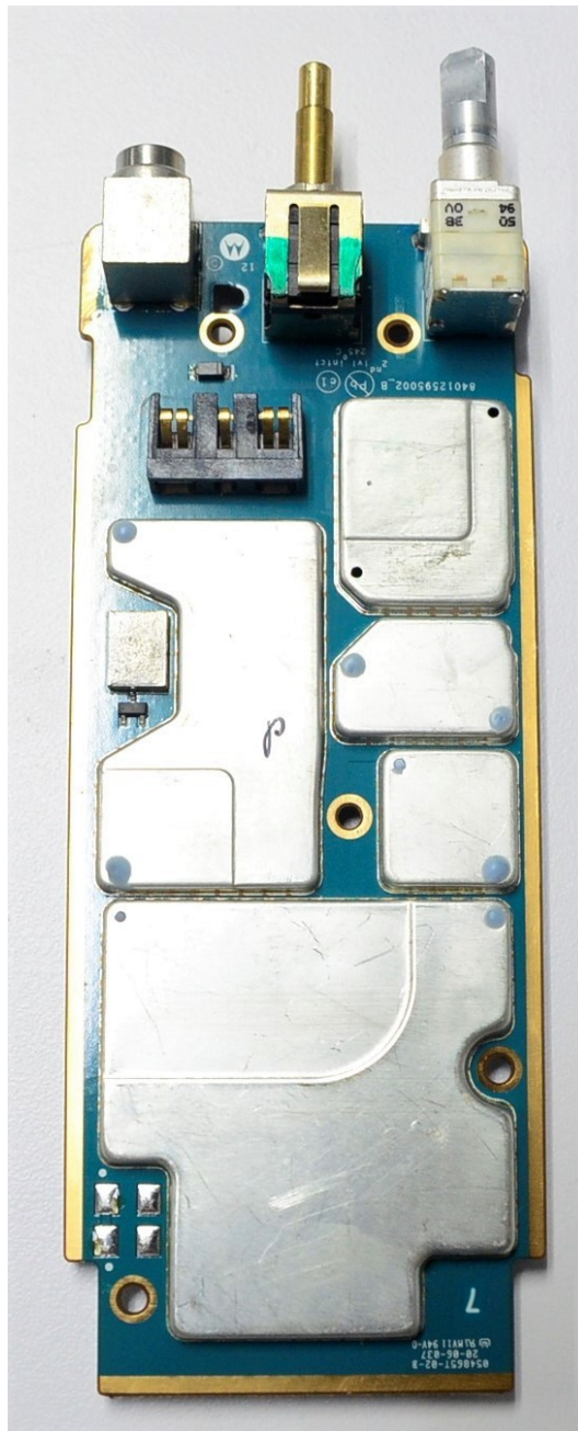
RF board with Shields (Bottom)
