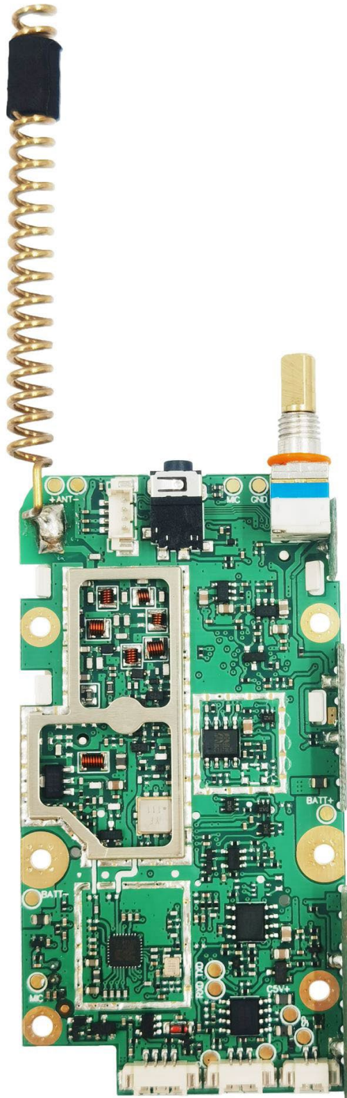
EXHIBIT 9D - RF board without Shields (Bottom)
