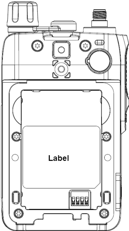
Figure 2: FCC/IC Label Location EVX-S30 (AC146U004)
