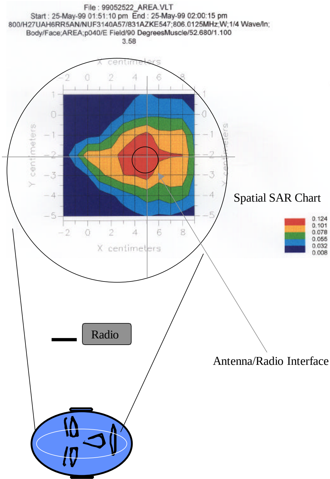
Partial View of Full Body Phantom As Viewed From Tissue Side
