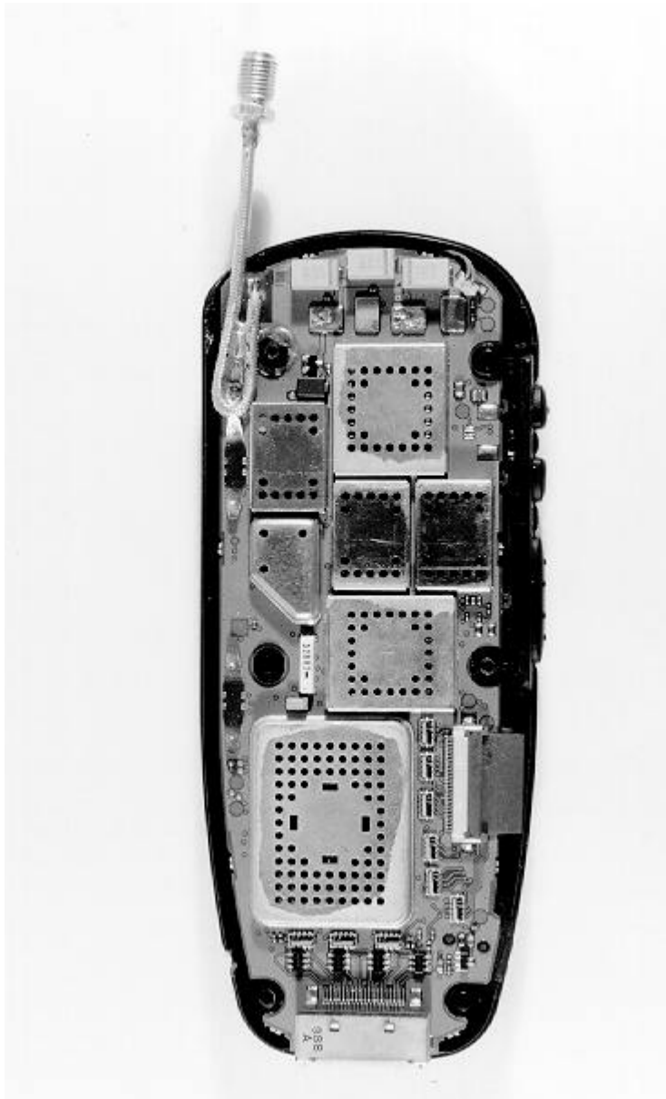
Photograph 7-1: Back side of main circuit board showing a semi rigid cable with female SMA connector soldered on the board.
