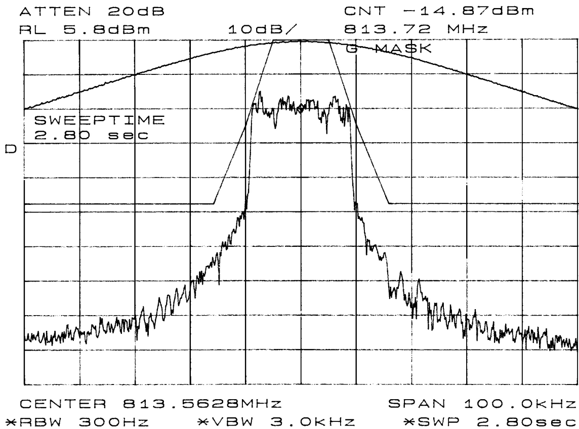
Figure 6-5: Quad-QPSK Modulation performance relative to mask 47 CFR 90.210(g). MAX. POWER (600mW):
