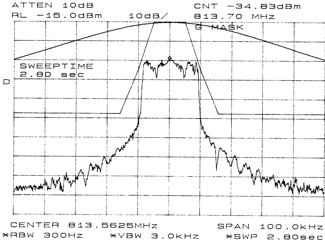
Figure 6-6: Quad-QPSK Modulation performance relative to mask 47 CFR 90.210(g). MIN. POWER (2.4mW):
