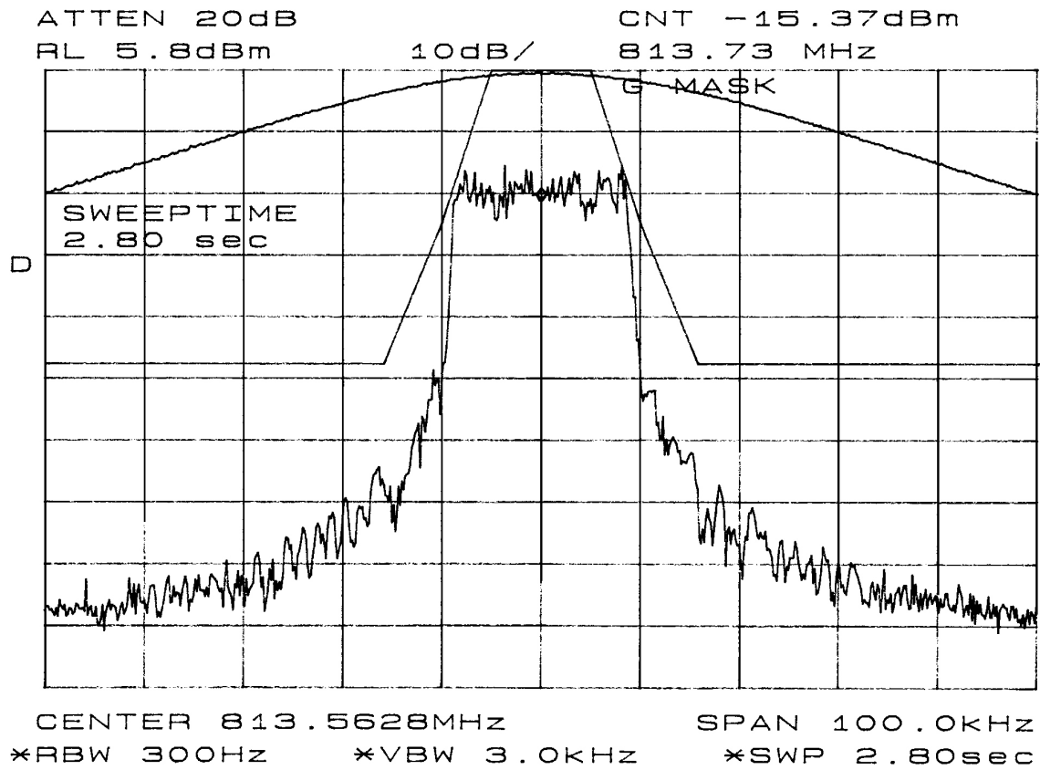
Figure 6-7: Quad-16QAM Modulation performance relative to mask 47 CFR 90.210(g). MAX. POWER (600mW):
