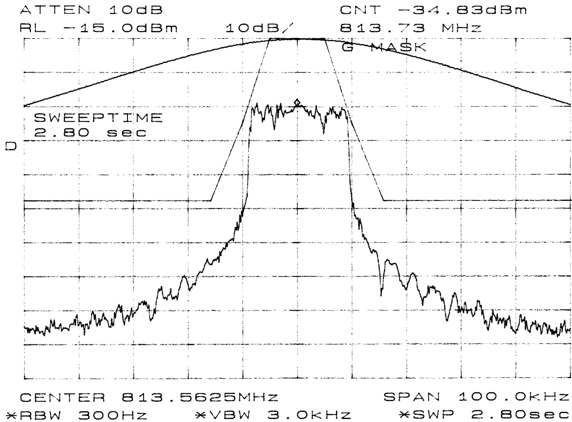
Figure 6-10: Quad-64QAM Modulation performance relative to mask 47 CFR 90.210(g). MIN. POWER (2.4mW):
