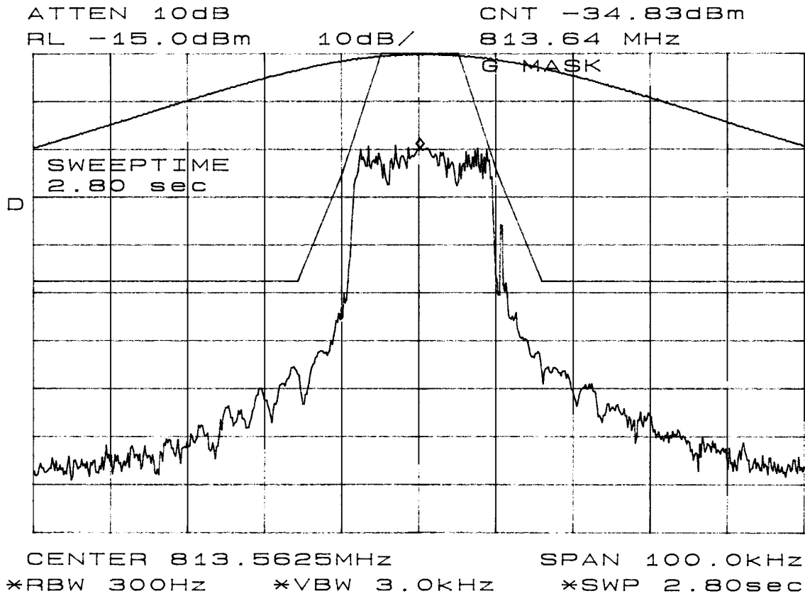
Figure 6-8: Quad-16QAM Modulation performance relative to mask 47 CFR 90.210(g). MIN. POWER (2.4mW):
