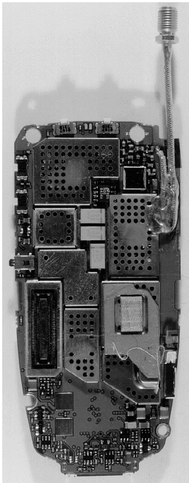
Photograph 7-2: Front side of main circuit board showing a semi rigid cable with female SMA connector soldered on the board.
