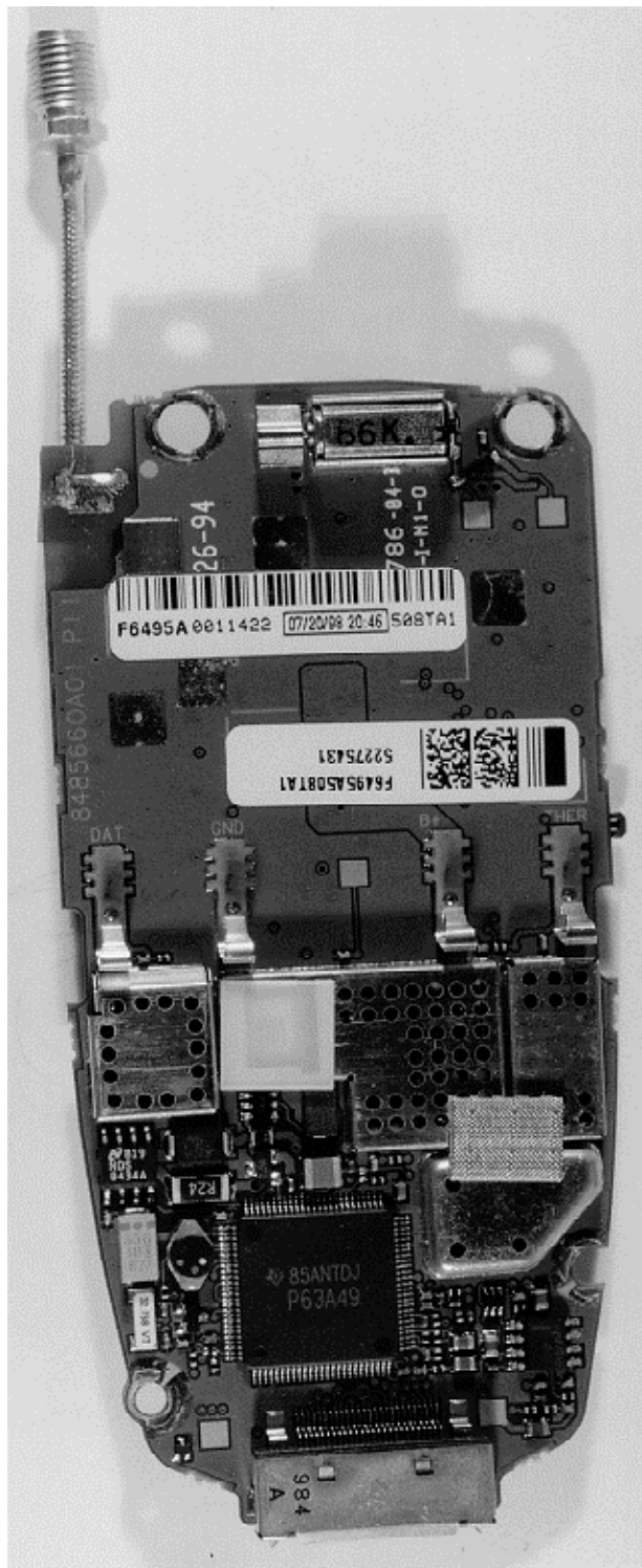
Photograph 7-1: Back side of main circuit board showing a semi rigid cable with female SMA connector soldered on the board.
