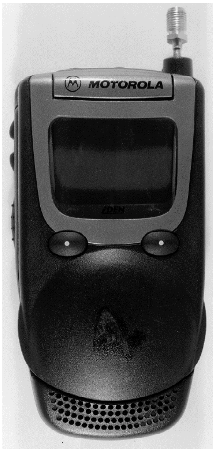
Photograph 7-3: Front view of radio, with a semi rigid cable with female SMA connector soldered on the main circuit board, and enclosed in modified housing for RX/TX conducted emissions testing.
