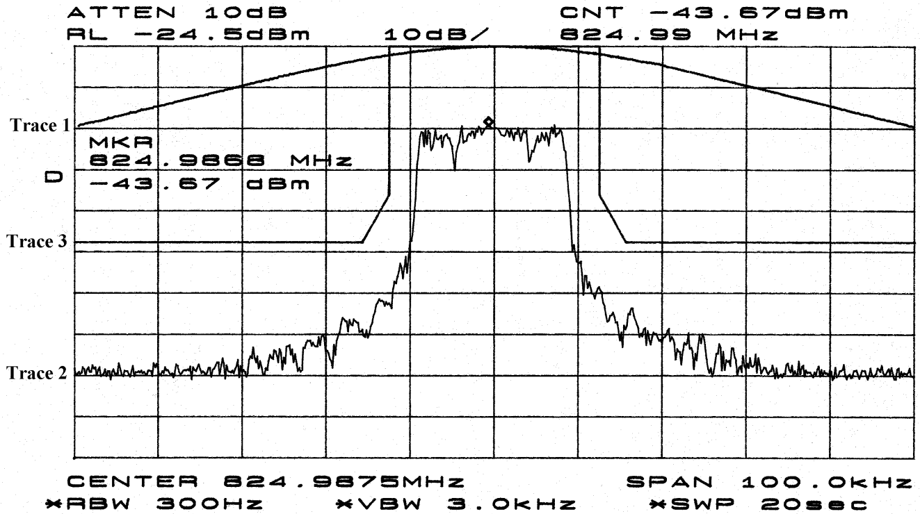
Figure 6-8: Quad-16QAM Modulation performance relative to mask 47 CFR 90.691(a).
