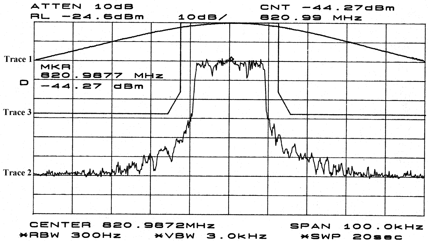
Figure 6-4: Quad-16QAM Modulation performance relative to mask 47 CFR 90.691(a). MIN. POWER:
