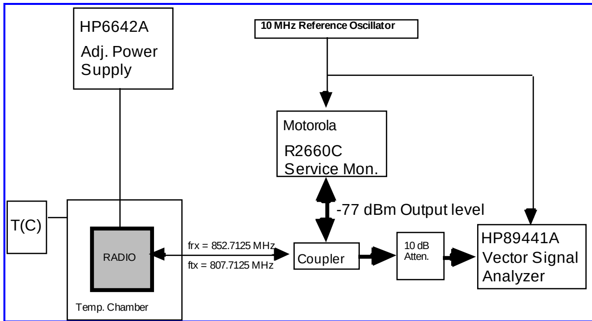
Figure 7-1: Transmit Frequency Measurement Setup
