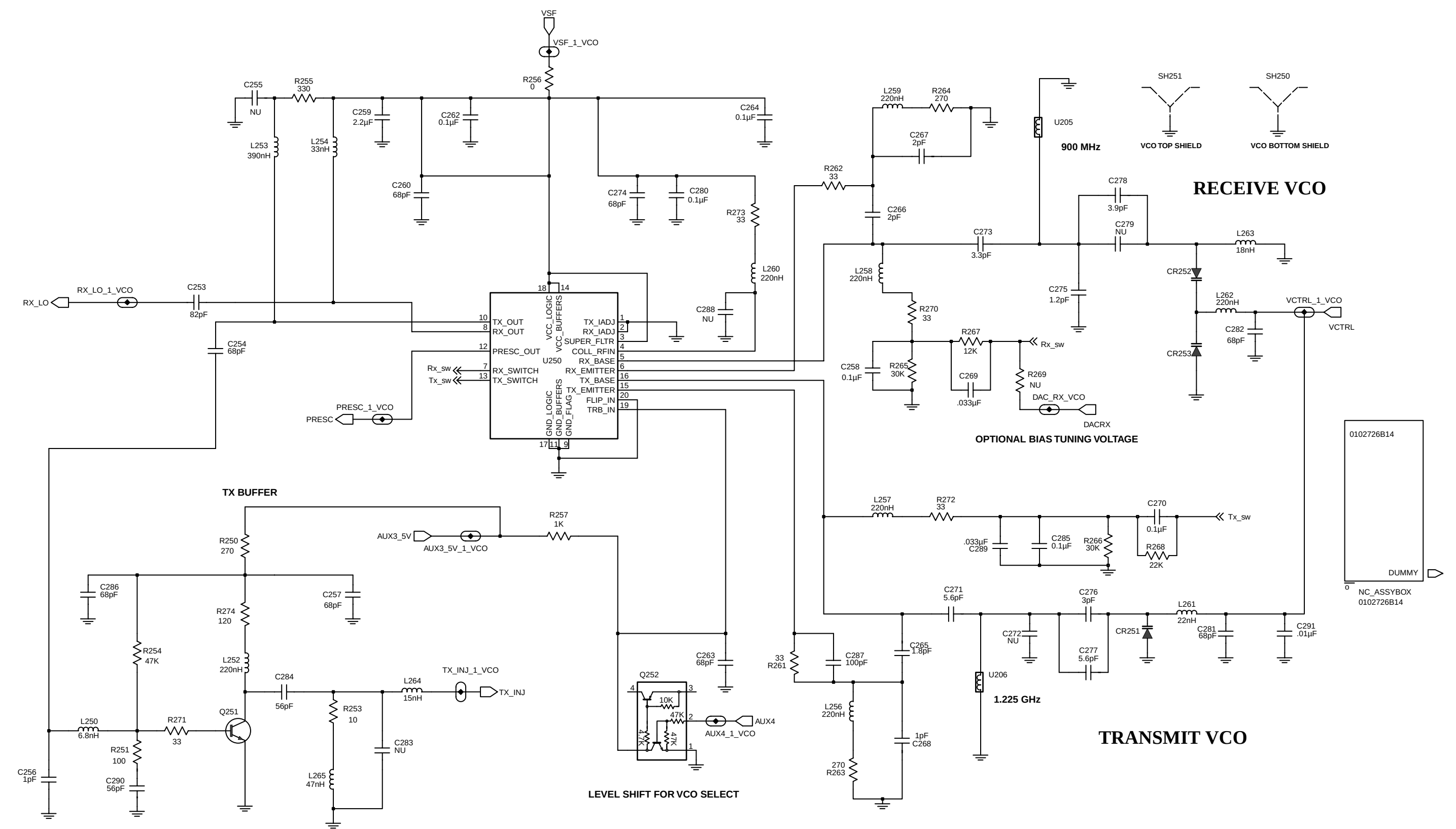
800 MHz Voltage Controlled Oscillator
