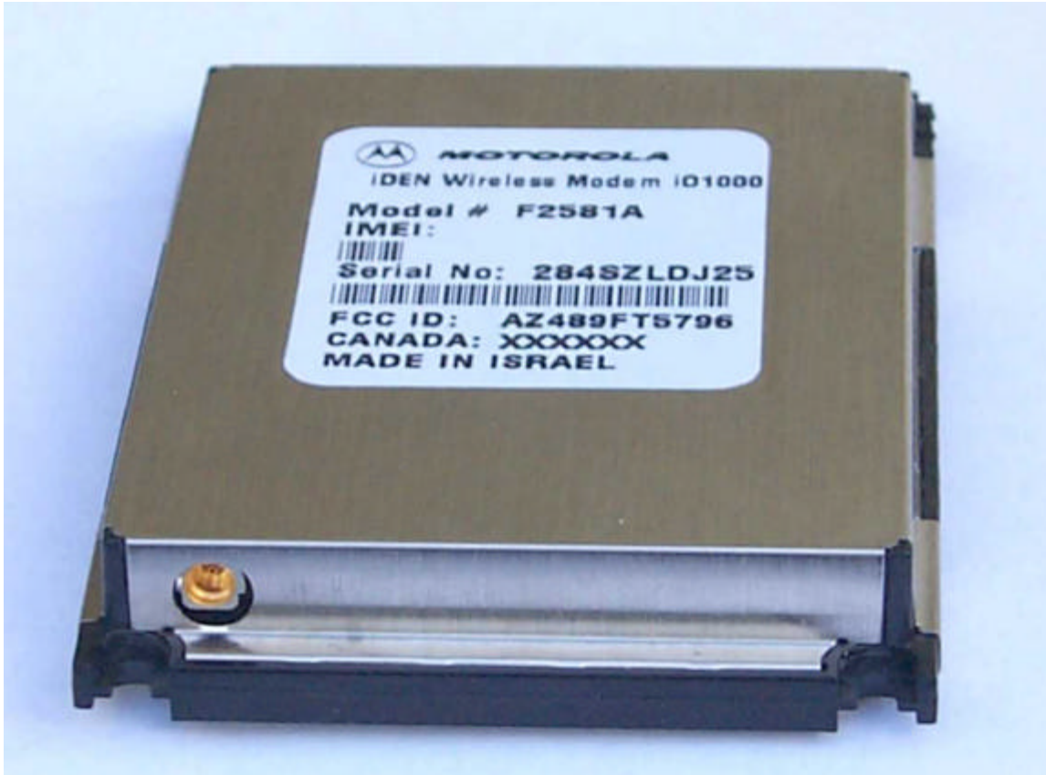
Photograph 3-3: Angled view of transceiver, showing antenna connector
