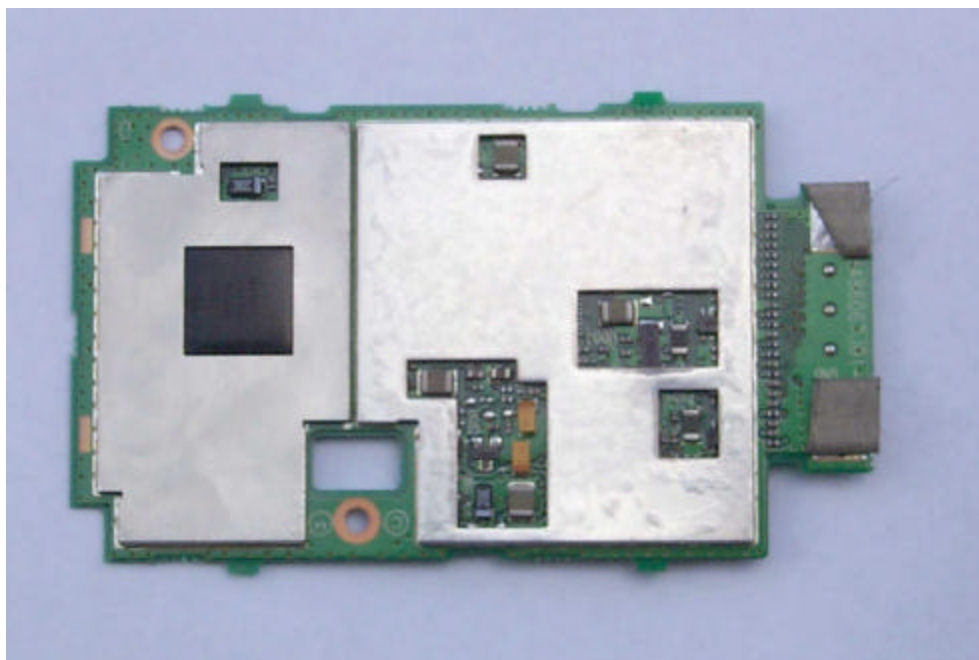
Photograph 9-4: Bottom side of transceiver Logic Board.
