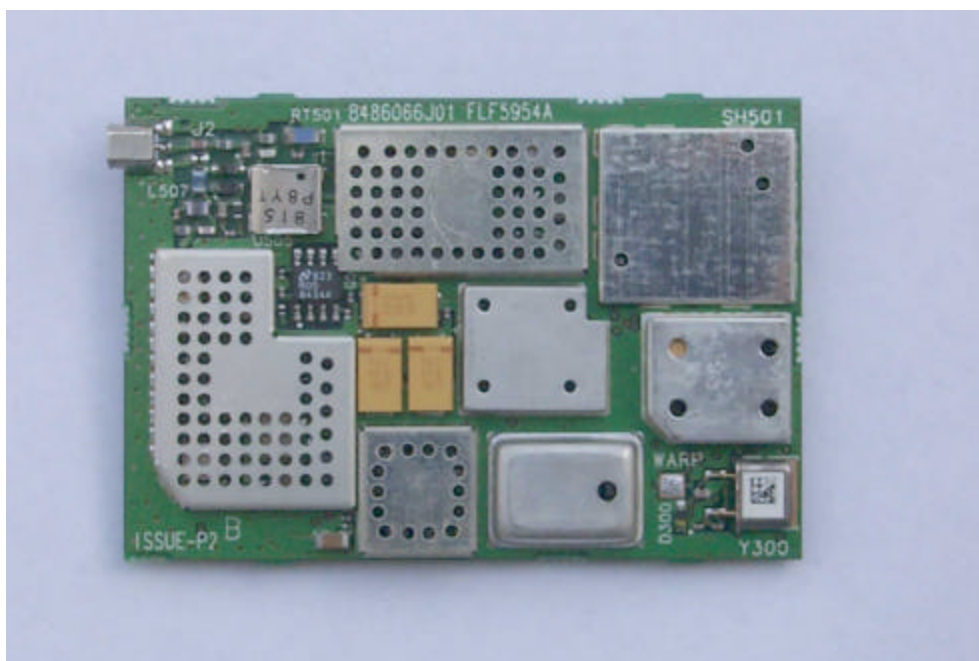
Photograph 9-1: Top side of transceiver RF Board.
