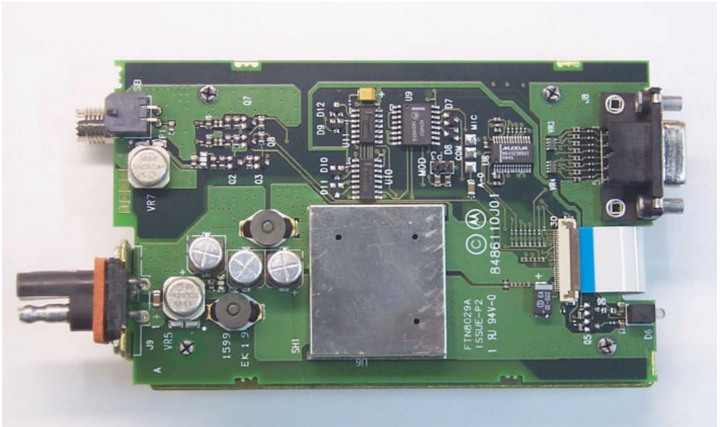
Photograph 9-2: Bottom side of internal chassis, showing the interface board, the 9-pin data connector and the DC power connector.
