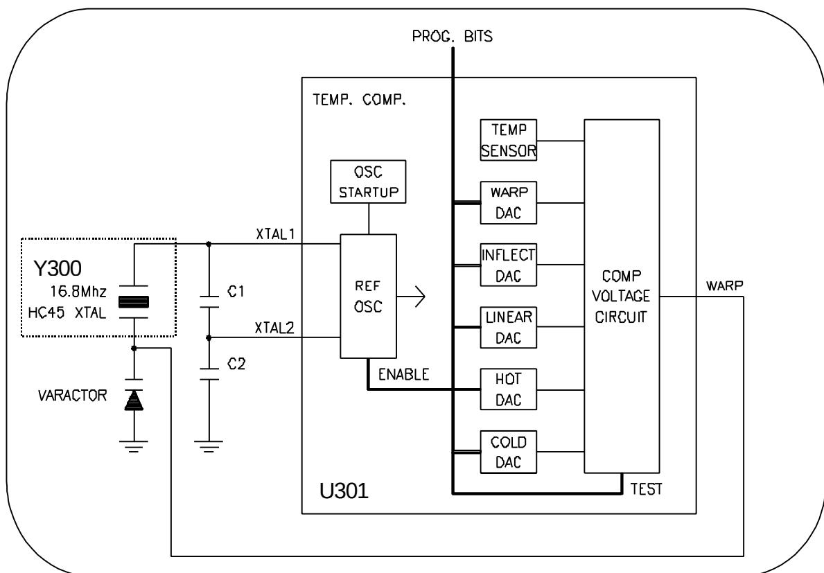
Figure 4-1: 16.8 MHz Reference Oscillator
