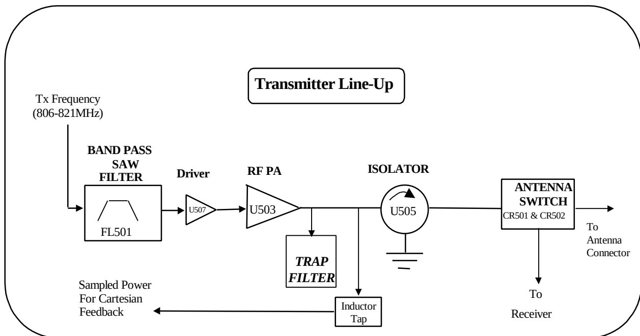
Figure 4-4: Transmitter Line-Up
