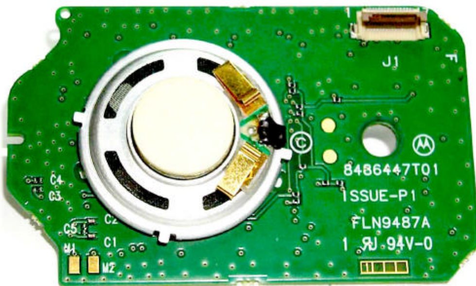
Photograph 9-5: Front side of keypad Board, showing attached speaker.
