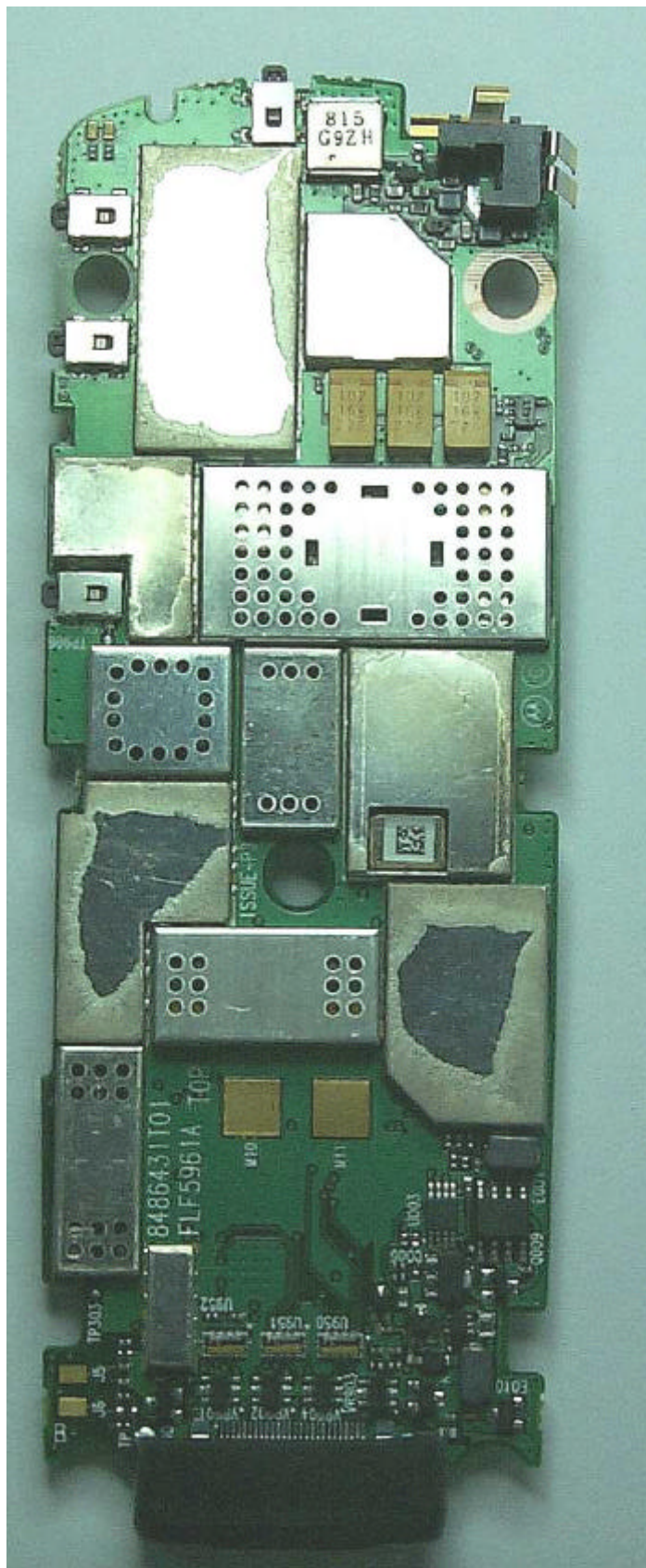
Photograph 9-2: Front side of the radio main Board.
