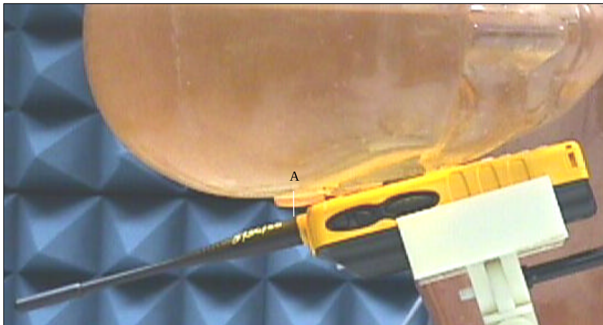
Figure 1b: Head Position - Right Ear.
