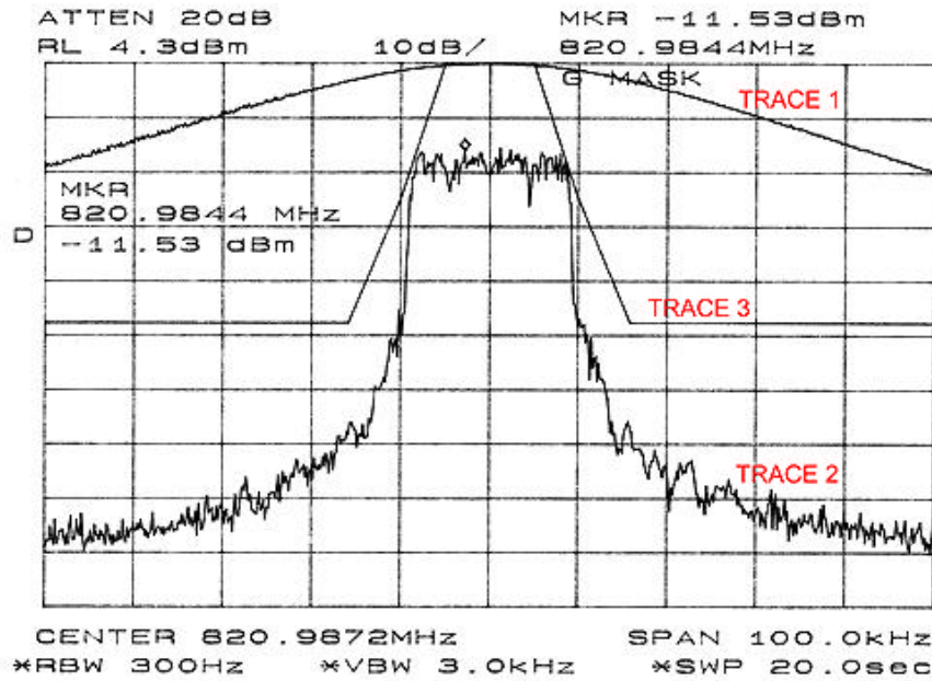
Figure 6-5: Quad-QPSK modulation performance at maximum output power setting
