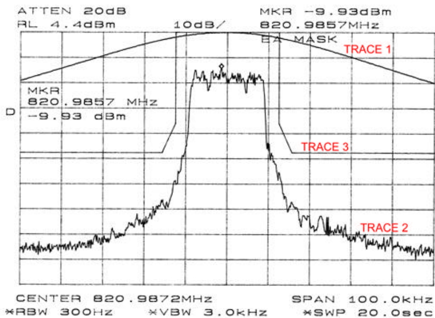
Figure 6-15: Quad-64QAM modulation performance at maximum output power setting
