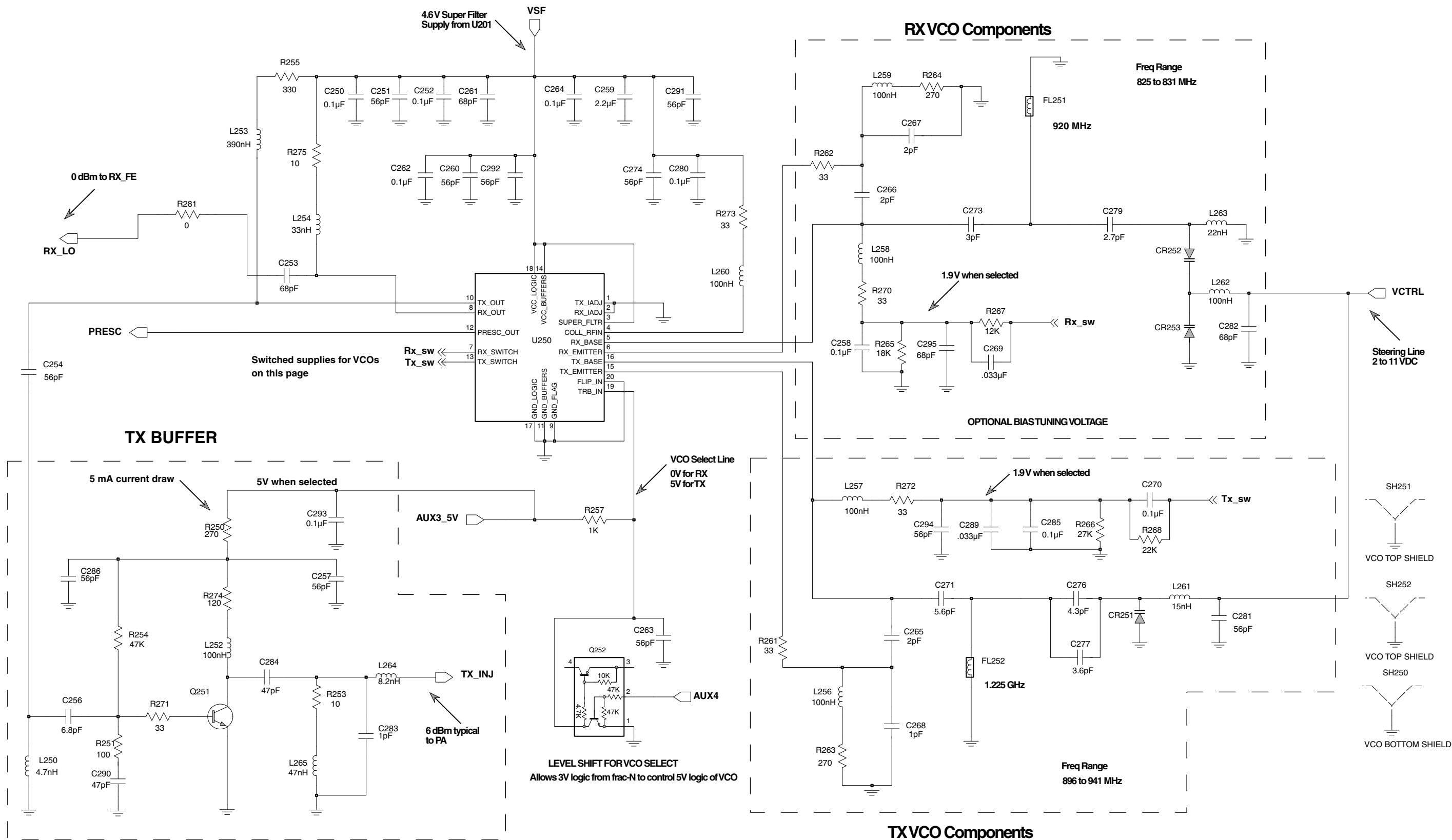
900 MHz Voltage Controlled Oscillator
