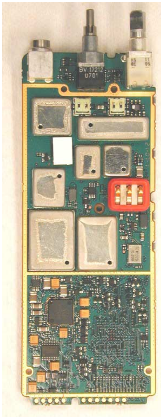
RF board with Shields (Bottom View)
