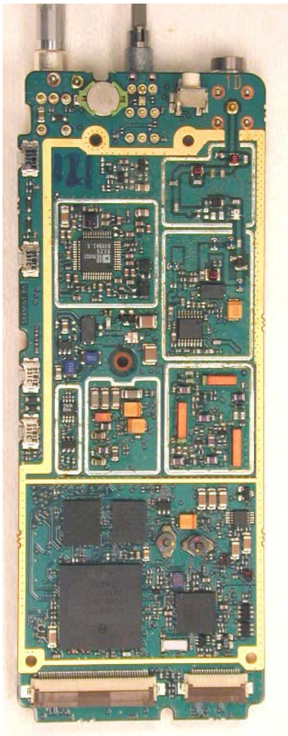
RF board without Shields (Top View)
