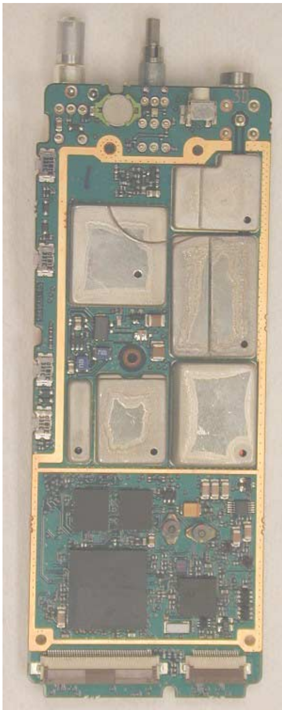
RF board with Shields (Top View)
