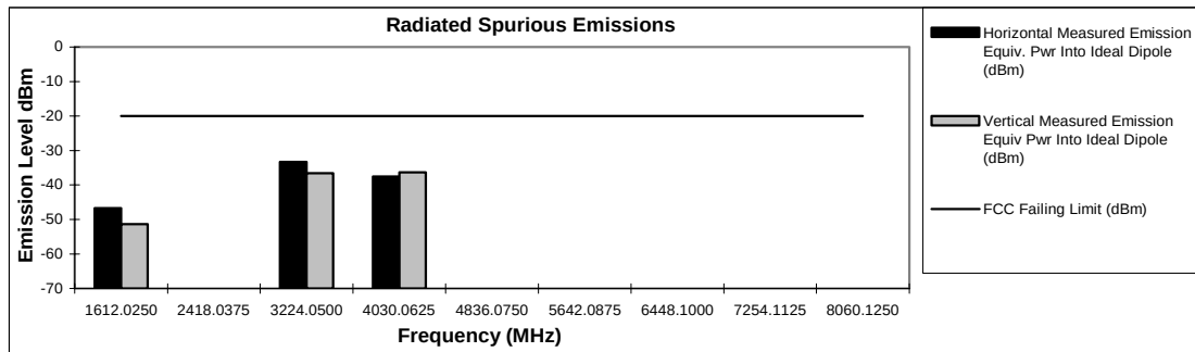
Graph 6G – 4: 3.3 Watts, 806.0125 MHz, 12.5 kHz Channel Spacing
