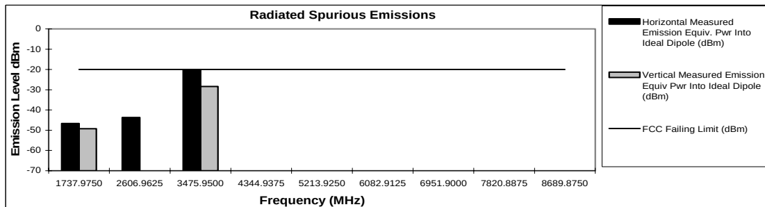
Graph 6G – 7: 3.3 Watts, 868.9875 MHz, 12.5 kHz Channel Spacing
