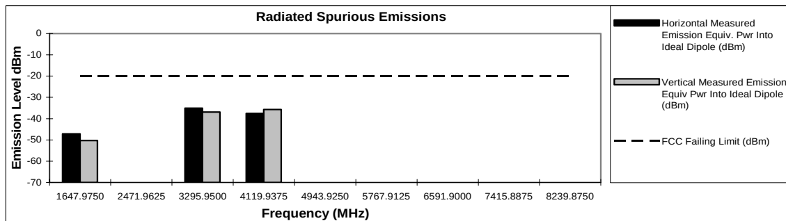
Graph 6G – 5: 3.3 Watts, 823.9875 MHz, 12.5 kHz Channel Spacing
