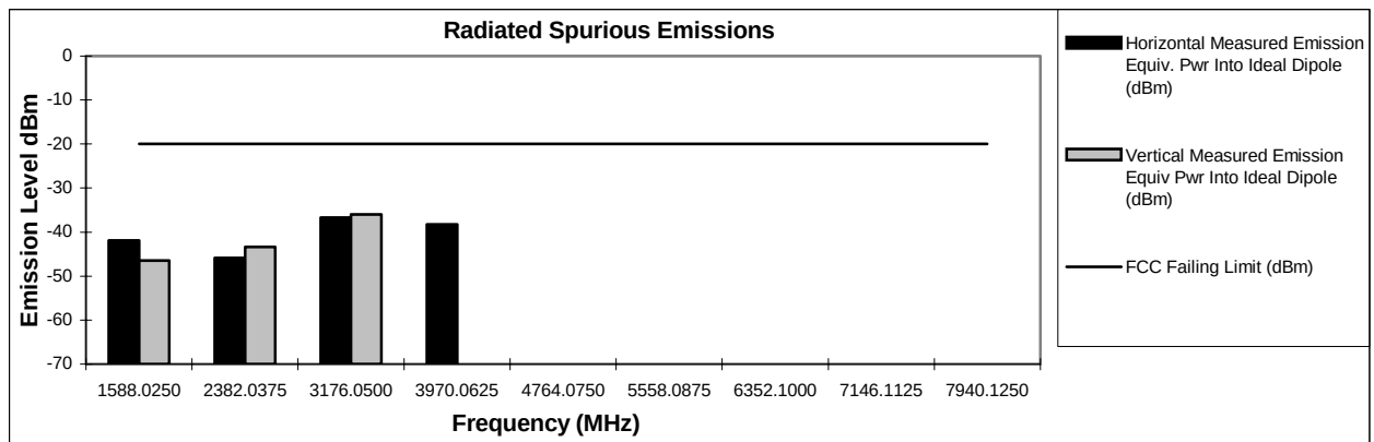
Graph 6G – 3: 2.9 Watts, 794.0125 MHz, 12.5 kHz Channel Spacing
