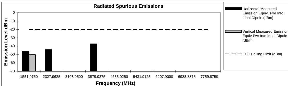
Graph 6G – 2: 2.9 Watts, 775.9875 MHz, 12.5 kHz Channel Spacing
