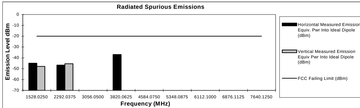
Graph 6G – 1: 2.9 Watts, 764.0125 MHz, 12.5 kHz Channel Spacing
