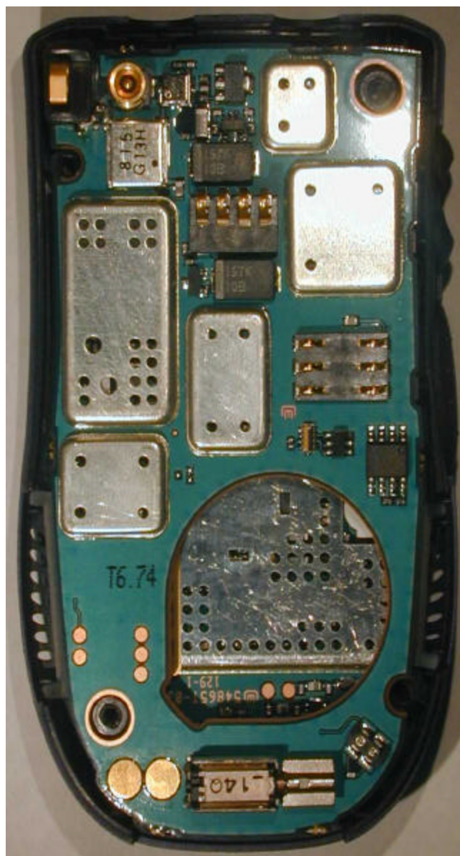
Photograph 9-4: Back side of radio product main board in housing.
