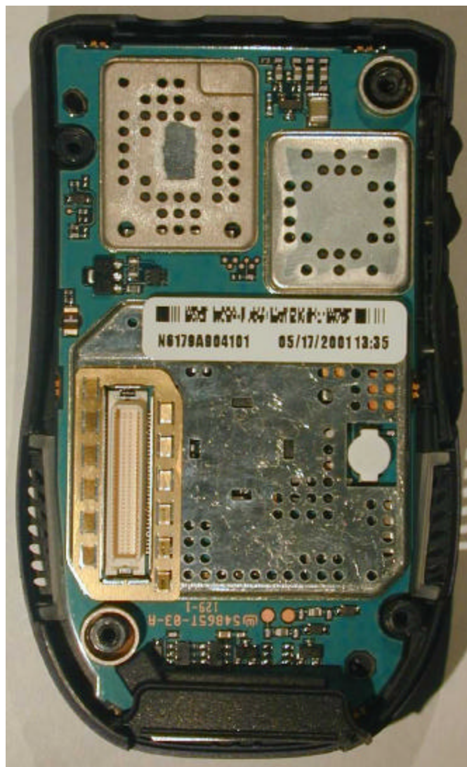
Photograph 9-2: Back side of keypad/controller board in housing.
