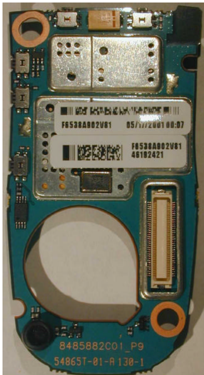
Photograph 9-3: Front side of radio product main board.
