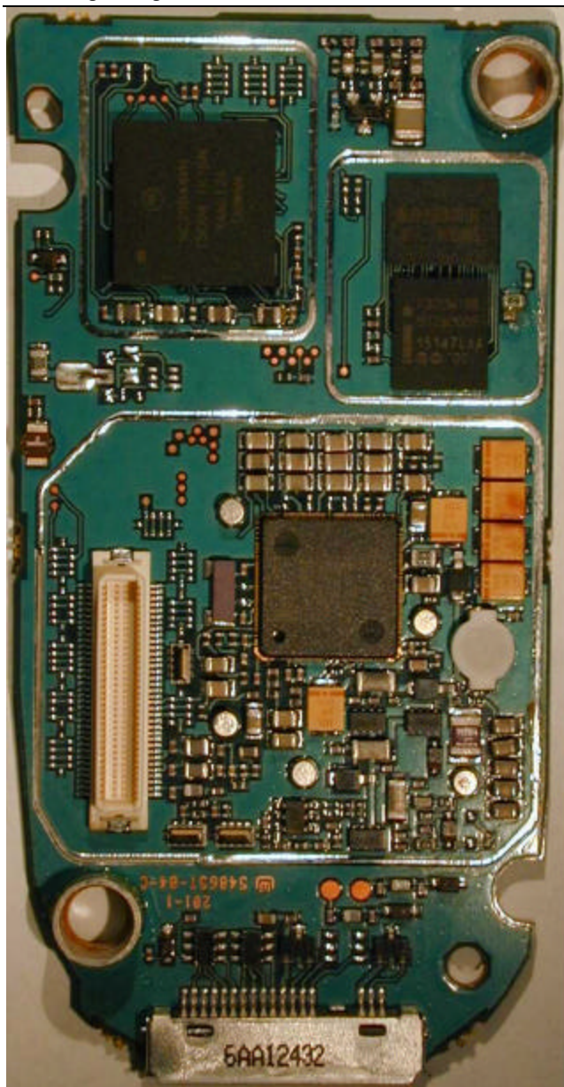
Photograph 9-5: Back side of keypad/controller board with no shields.
