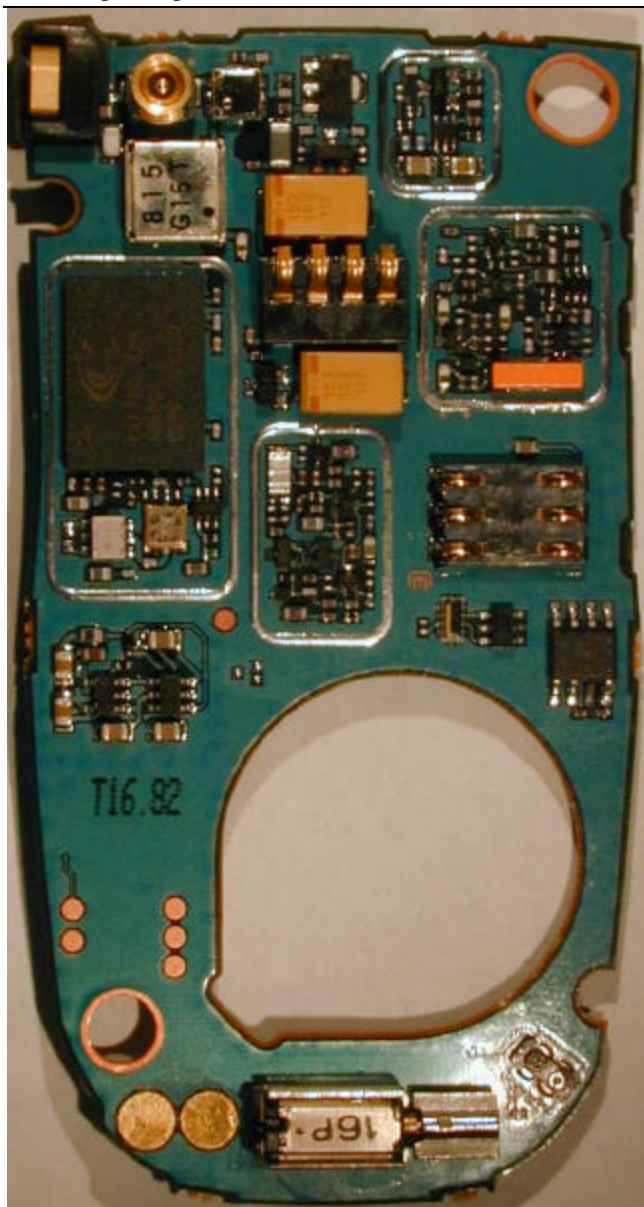
Photograph 9-7: Back side of radio product main board with no shields.
