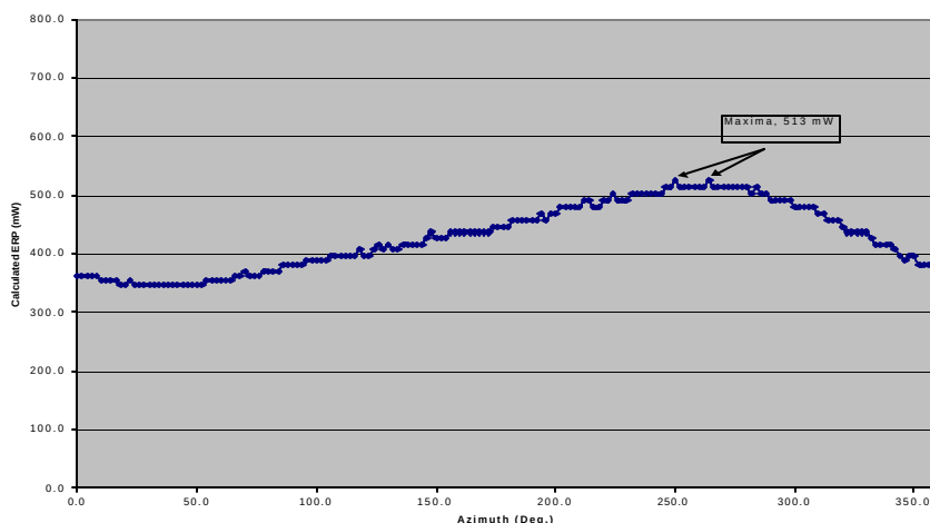
Figure 6-49: Maximum ERP vs. Azimuth
