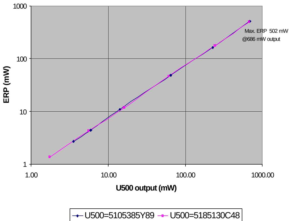
Figure 6-51: Maximum ERP vs. U500 Output Power
