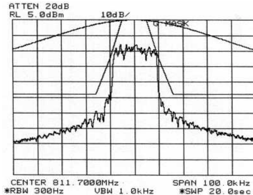
Figure 6-25: Quad-64-QAM Modulation performance (Alternate U500), relative to mask 47 CFR 90.210g. MAXIMUM POWER SETTING:
