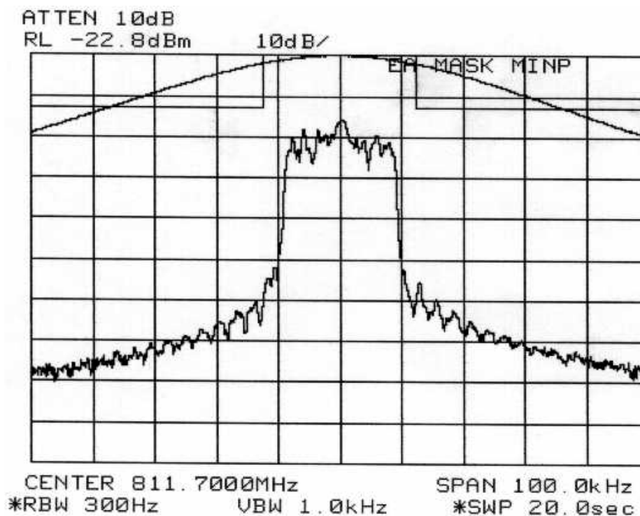
Figure 6-28: Quad-64-QAM Modulation performance (Alternate U500), relative to mask 47 CFR 90.691. MINIMUM POWER SETTING:
