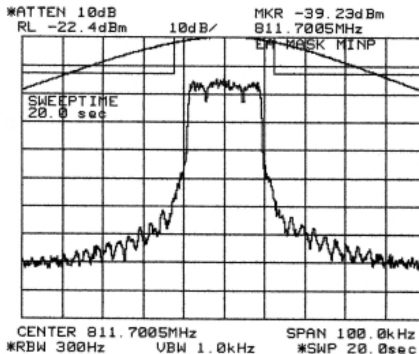
Figure 6-12: Quad-16-QAM Modulation performance (Primary U500), relative to mask 47 CFR 90.691. MINIMUM POWER SETTING:
