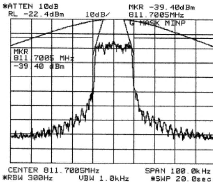
Figure 6-10: Quad-16-QAM Modulation performance (Primary U500), relative to mask 47 CFR 90.210g. MINIMUM POWER SETTING:
