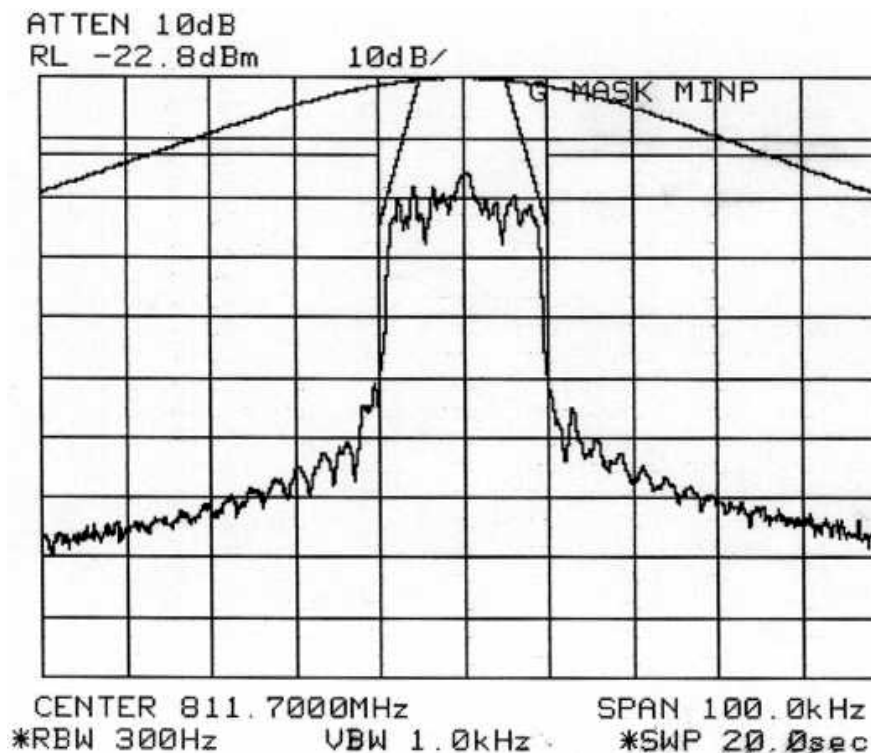
Figure 6-26: Quad-64-QAM Modulation performance (Alternate U500), relative to mask 47 CFR 90.210g. MINIMUM POWER SETTING:
