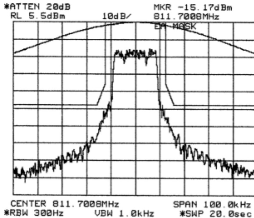
Figure 6-11: Quad-16-QAM Modulation performance (Primary U500), relative to mask 47 CFR 90.691. MAXIMUM POWER SETTING:
