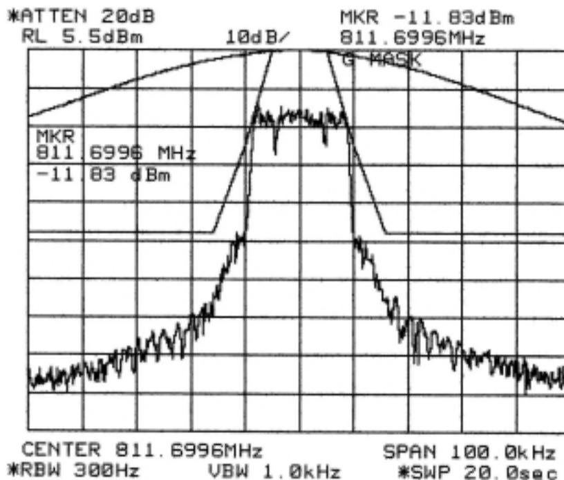
Figure 6-5: Quad-QPSK Modulation performance (Primary U500), relative to mask 47 CFR 90.210g. MAXIMUM POWER SETTING:
