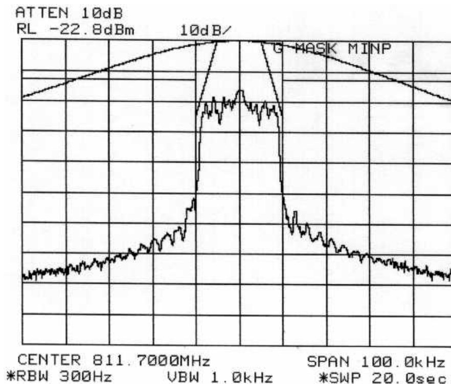
Figure 6-22: Quad-16-QAM Modulation performance (Alternate U500), relative to mask 47 CFR 90.210g. MINIMUM POWER SETTING:
