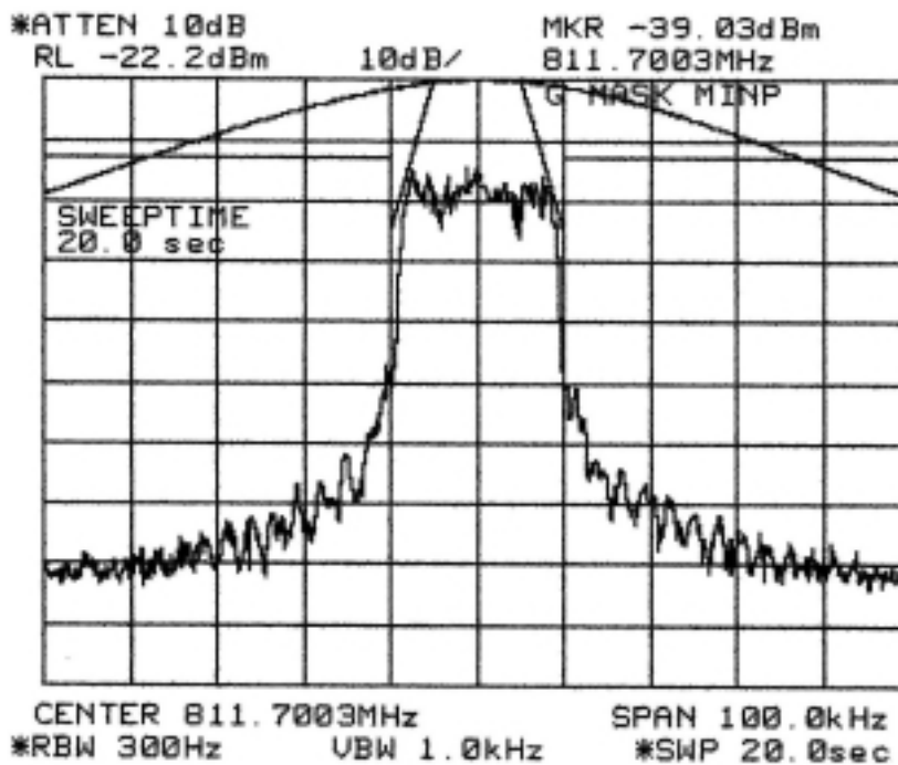
Figure 6-6: Quad-QPSK Modulation performance (Primary U500), relative to mask 47 CFR 90.210g. MINIMUM POWER SETTING:
