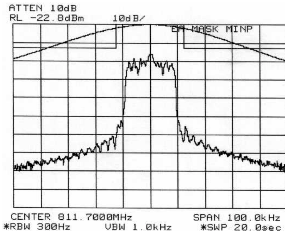
Figure 6-24: Quad-16-QAM Modulation performance (Alternate U500), relative to mask 47 CFR 90.691. MINIMUM POWER SETTING:
