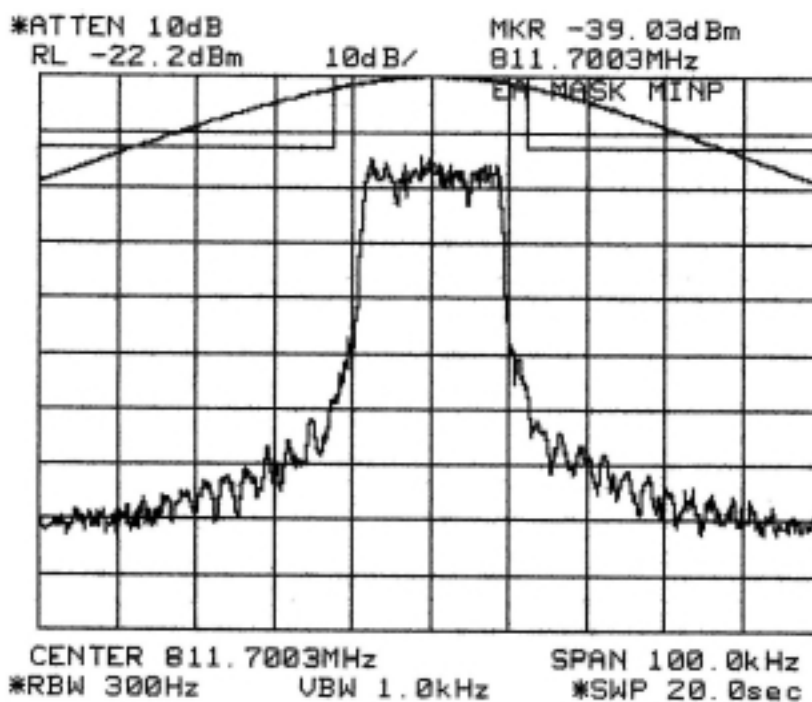
Figure 6-8: Quad-QPSK Modulation performance (Primary U500), relative to mask 47 CFR 90.691. MINIMUM POWER SETTING:
