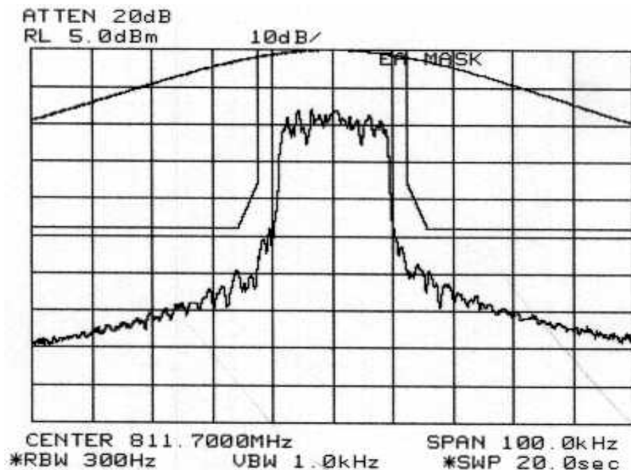
Figure 6-23: Quad-16-QAM Modulation performance (Alternate U500), relative to mask 47 CFR 90.691. MAXIMUM POWER SETTING:
