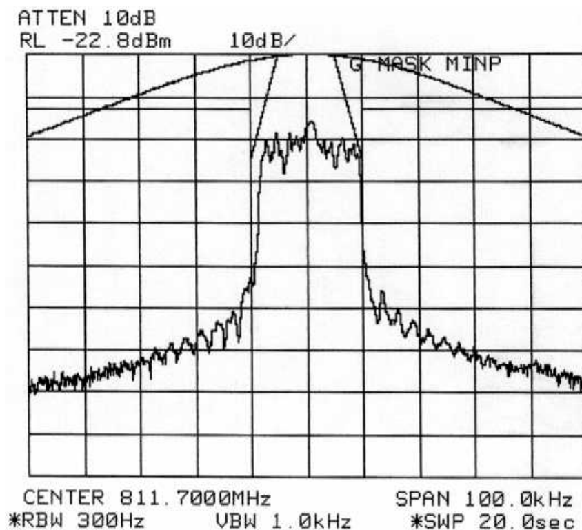
Figure 6-18: Quad-QPSK Modulation performance (Alternate U500), relative to mask 47 CFR 90.210g. MINIMUM POWER SETTING:
