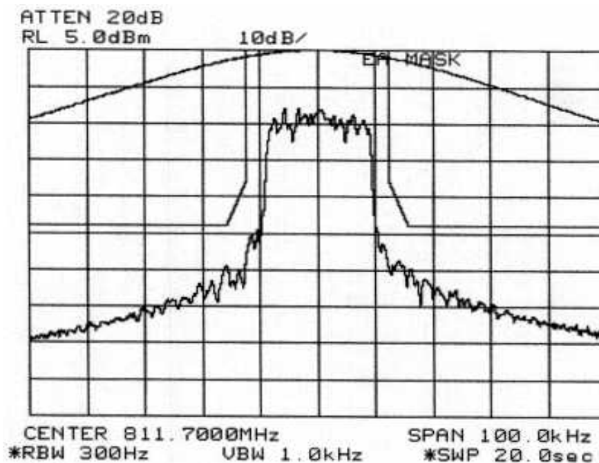
Figure 6-27: Quad-64-QAM Modulation performance (Alternate U500), relative to mask 47 CFR 90.691. MAXIMUM POWER SETTING:
