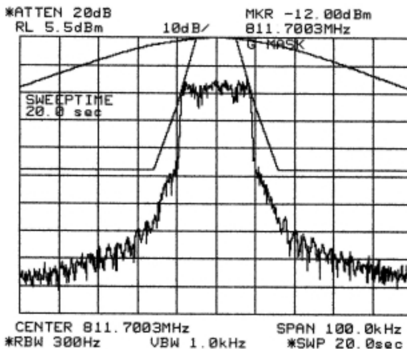
Figure 6-13: Quad-64-QAM Modulation performance (Primary U500), relative to mask 47 CFR 90.210g, MAXIMUM POWER SETTING:
