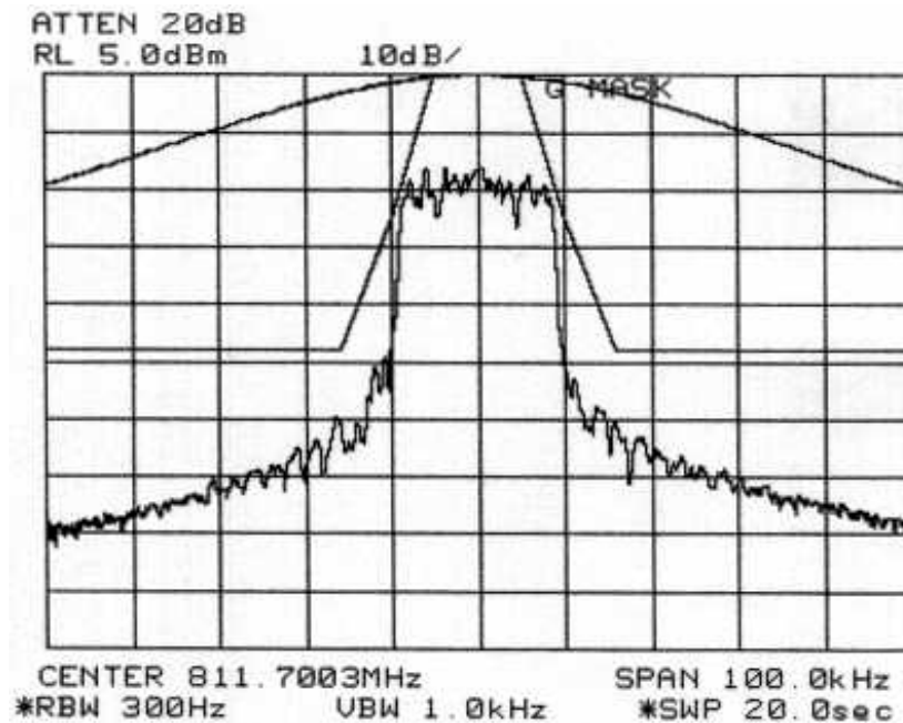
Figure 6-17: Quad-QPSK Modulation performance (Alternate U500), relative to mask 47 CFR 90.210g. MAXIMUM POWER SETTING:
