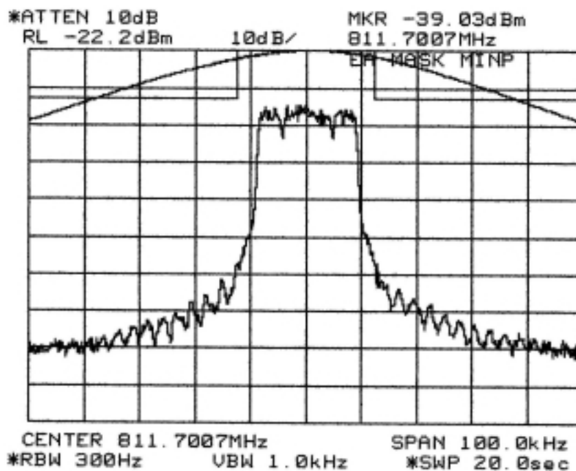
Figure 6-16: Quad-64-QAM Modulation performance (Primary U500), relative to mask 47 CFR 90.691. MINIMUM POWER SETTING:
