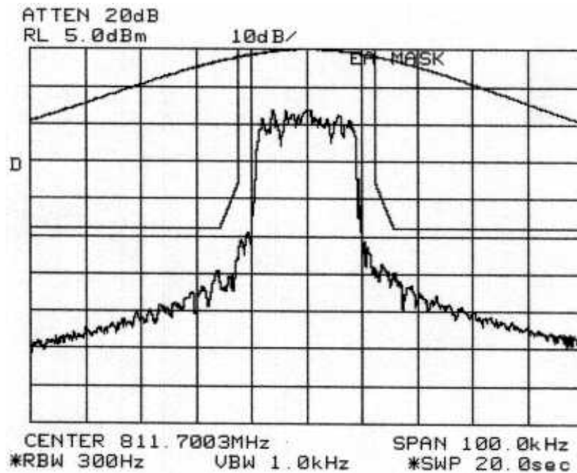
Figure 6-19: Quad-QPSK Modulation performance (Alternate U500), relative to mask 47 CFR 90.691. MAXIMUM POWER SETTING:
