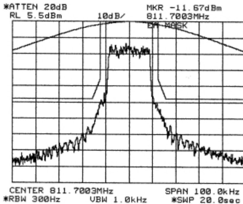
Figure 6-15: Quad-64-QAM Modulation performance (Primary U500), relative to mask 47 CFR 90.691. MAXIMUM POWER SETTING:
