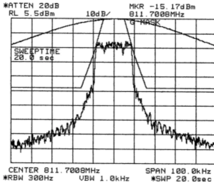
Figure 6-9: Quad-16-QAM Modulation performance (Primary U500), relative to mask 47 CFR 90.210g. MAXIMUM POWER SETTING:
