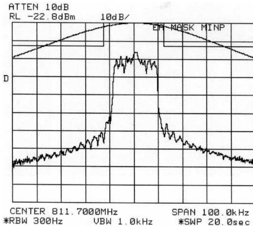
Figure 6-20: Quad-QPSK Modulation performance (Alternate U500), relative to mask 47 CFR 90.691. MINIMUM POWER SETTING:
