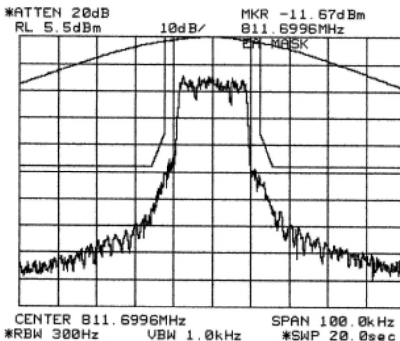
Figure 6-7: Quad-QPSK Modulation performance (Primary U500), relative to mask 47 CFR 90.691. MAXIMUM POWER SETTING:
