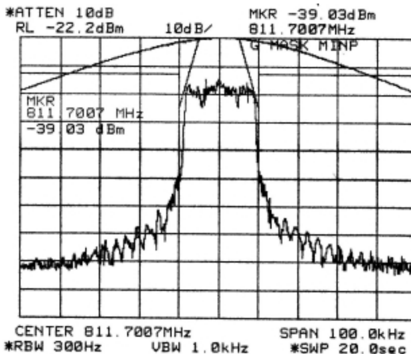
Figure 6-14: Quad-64-QAM Modulation performance (Primary U500), relative to mask 47 CFR 90.210g, MINIMUM POWER SETTING:
