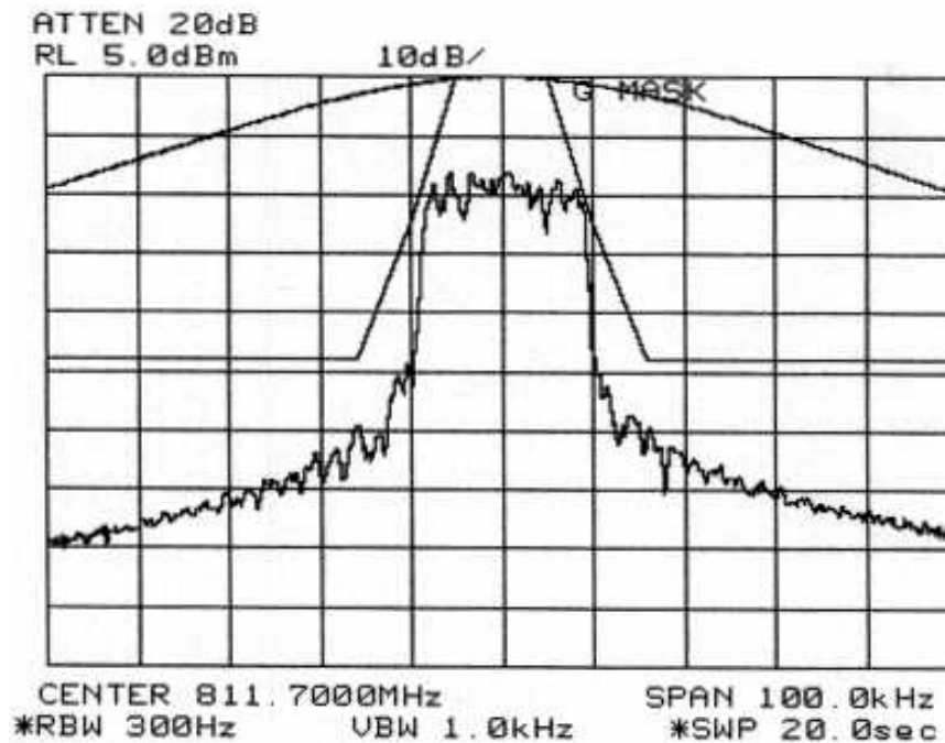
Figure 6-21: Quad-16-QAM Modulation performance (Alternate U500), relative to mask 47 CFR 90.210g. MAXIMUM POWER SETTING:
