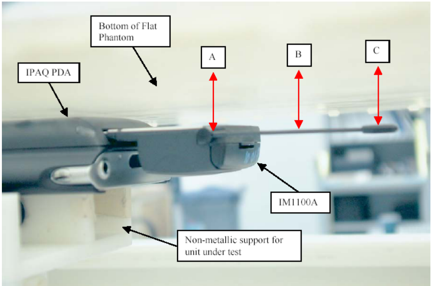
Figure 2: iM1100A with iPAQ PDA Palm/Pocket Computer
