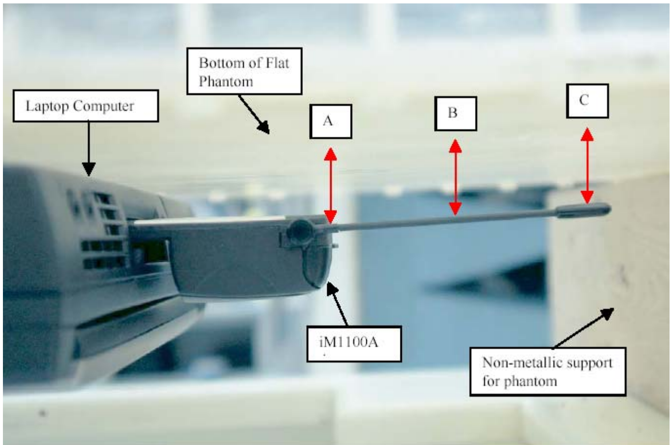
Figure 1: iM1100A with Laptop Computer
