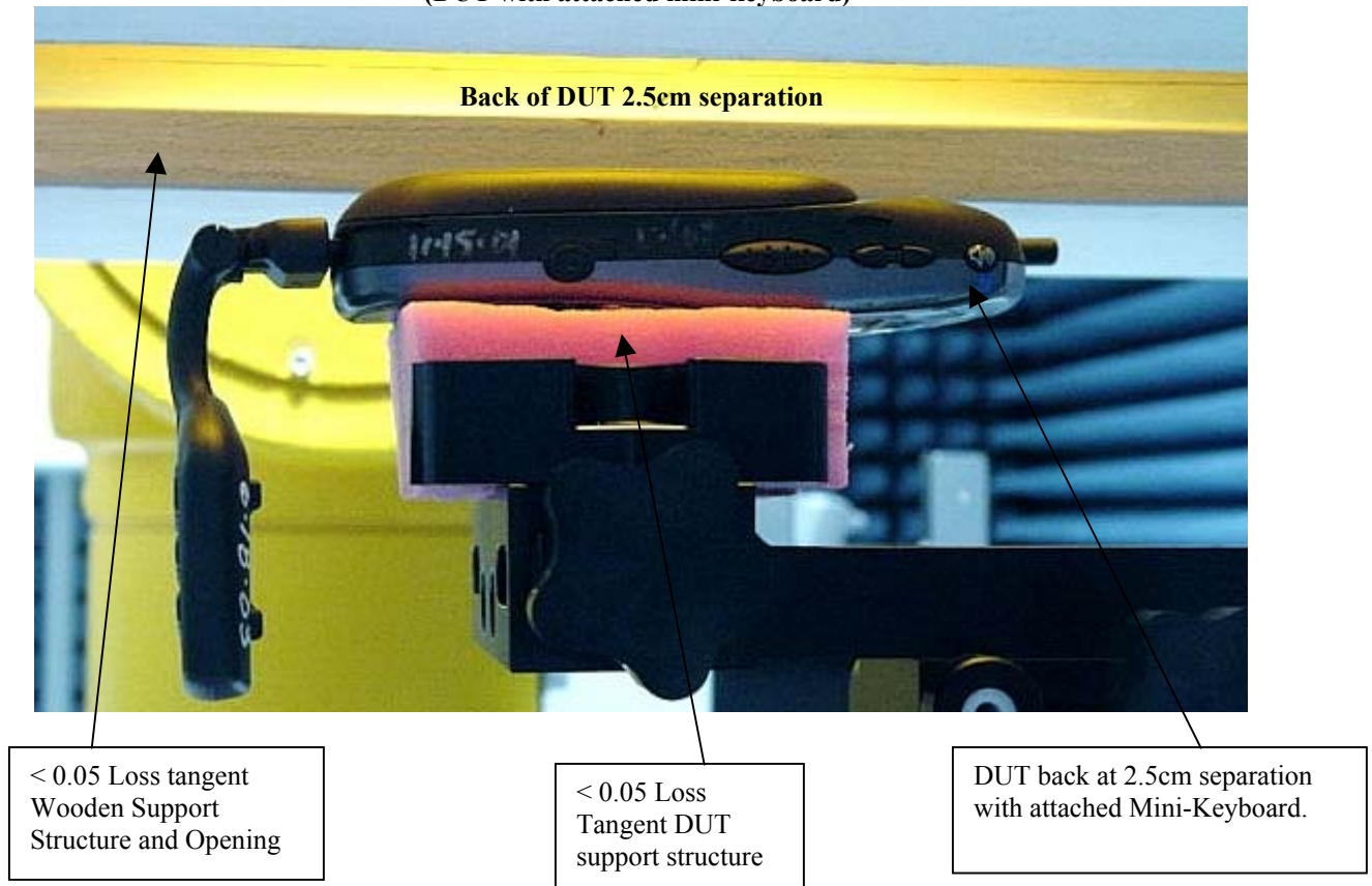
Figure 1: Highest S.A.R. Test Position (DUT with attached mini-keyboard)
