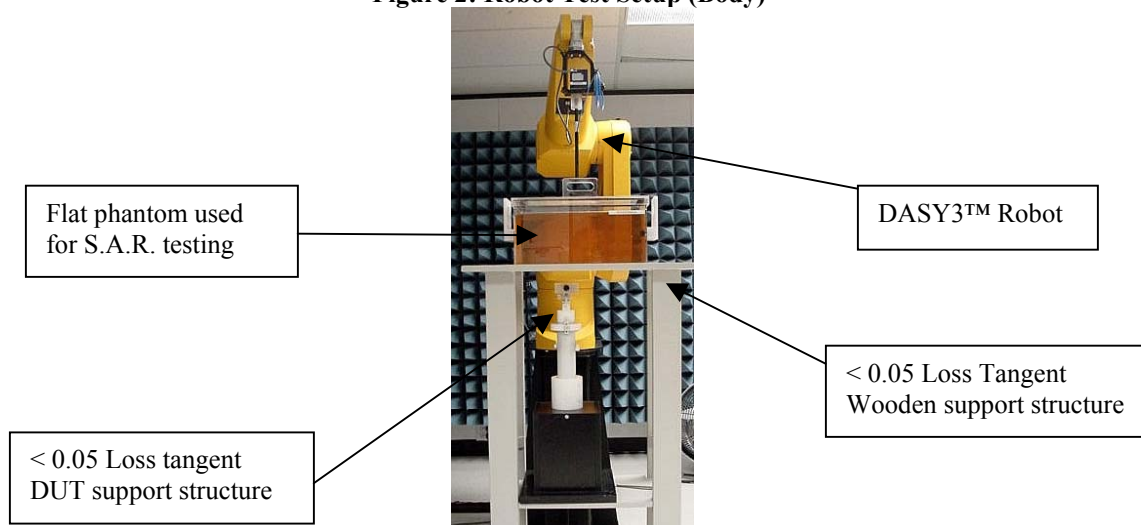
Figure 2: Robot Test Setup (Body)
