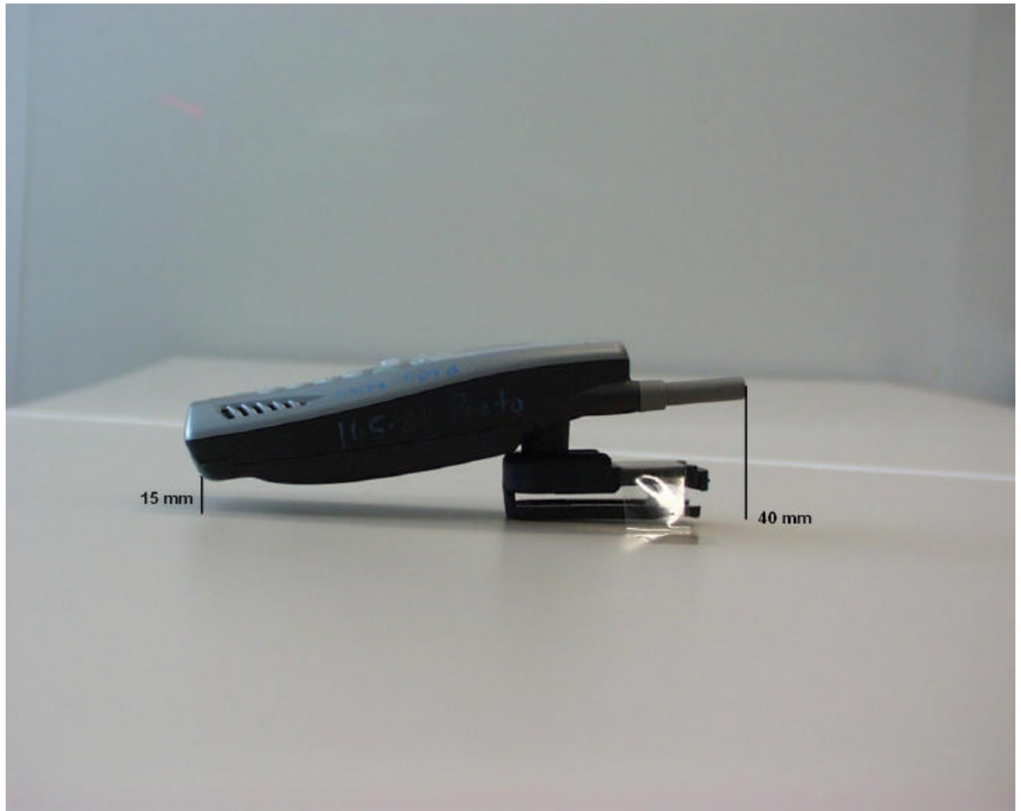
Figure 19. Spacing Dictated the Belt-Clip with Antenna Retracted
