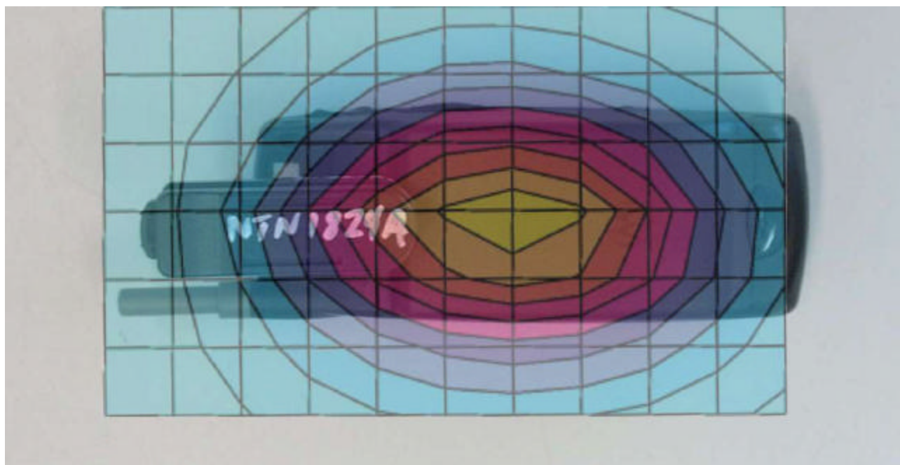
Figure 6. Typical Antenna Extended Body Worn Contour Overlaid on the Back of the Phone the Belt-Clip
