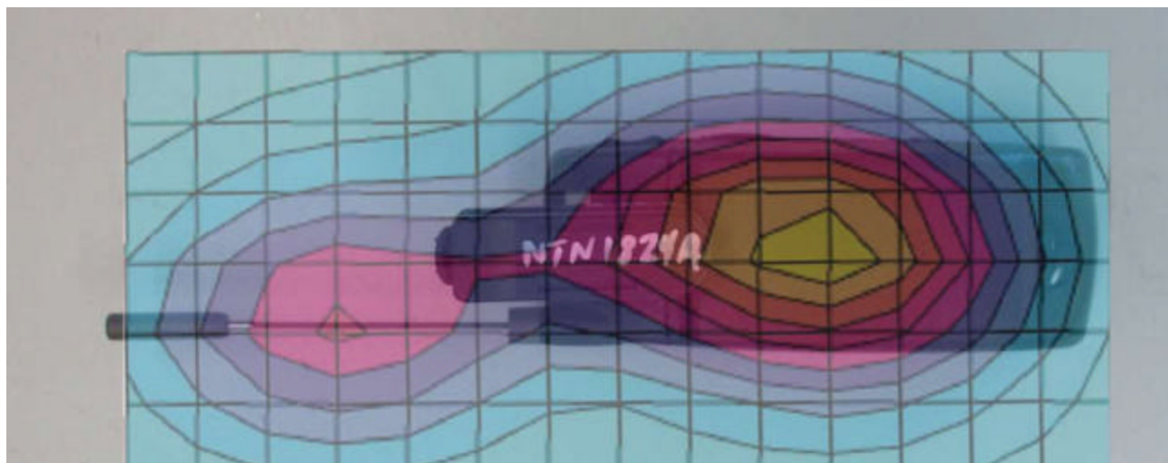
Figure 9. Typical Antenna Extended Body Worn Contour Overlaid on the Back of the Phone with Belt-clip
