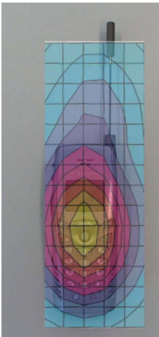
Figure 3. Typical Push-to-Talk Mode with the Antenna Extended Contour Plot Overlaid on Face of the Phone
