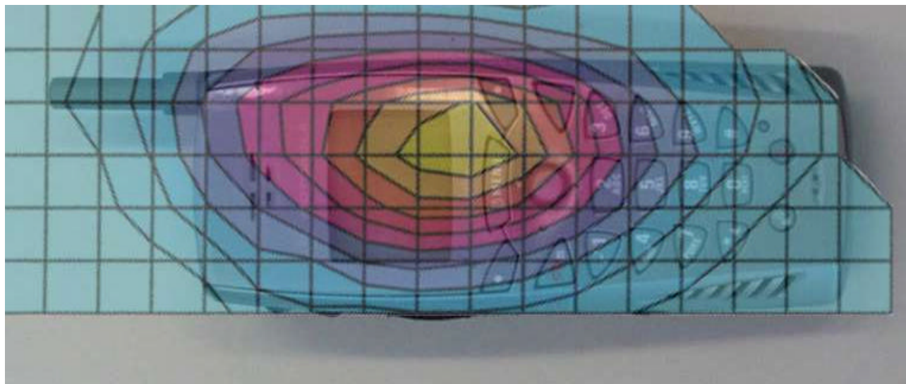
Figure 8. Typical 900MHz Phone Mode Antenna Retracted Head Adjacent Contour Plot Overlaid on Face of the Phone
