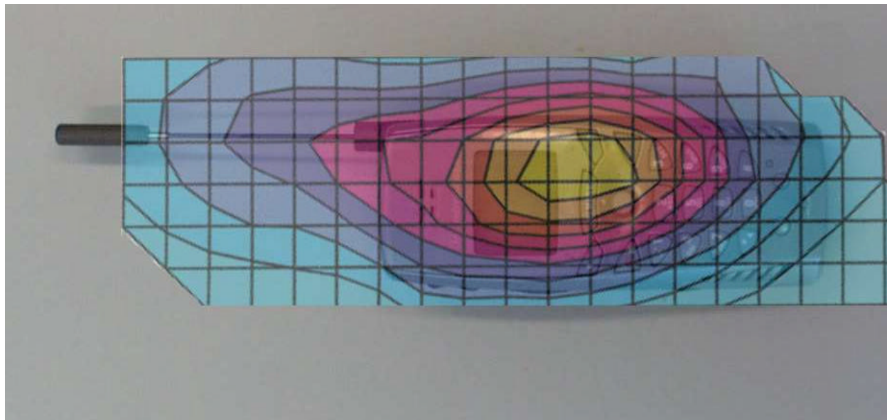
Figure 1. Typical 800MHz Phone Mode Antenna Extended Head Adjacent Contour Plot Overlaid on Face of the Phone
