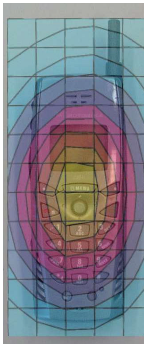
Figure 4. Typical Push-to-Talk Mode with the Antenna Retracted Plot Overlaid on Face of the Phone
