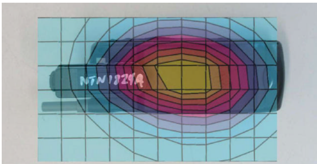
Figure 10. Typical Antenna Extended Body Worn Contour Overlaid on the Back of the Phone with Belt-clip
