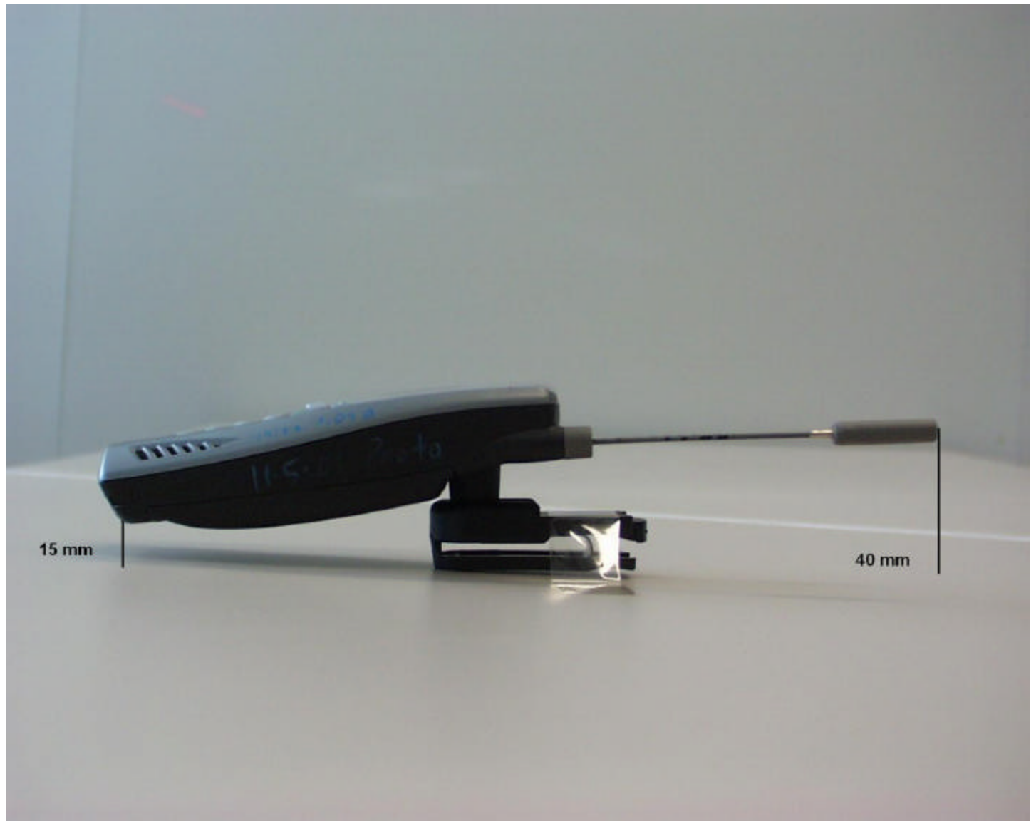
Figure 18. Spacing Dictated By the Belt-Clip with Antenna Extended
