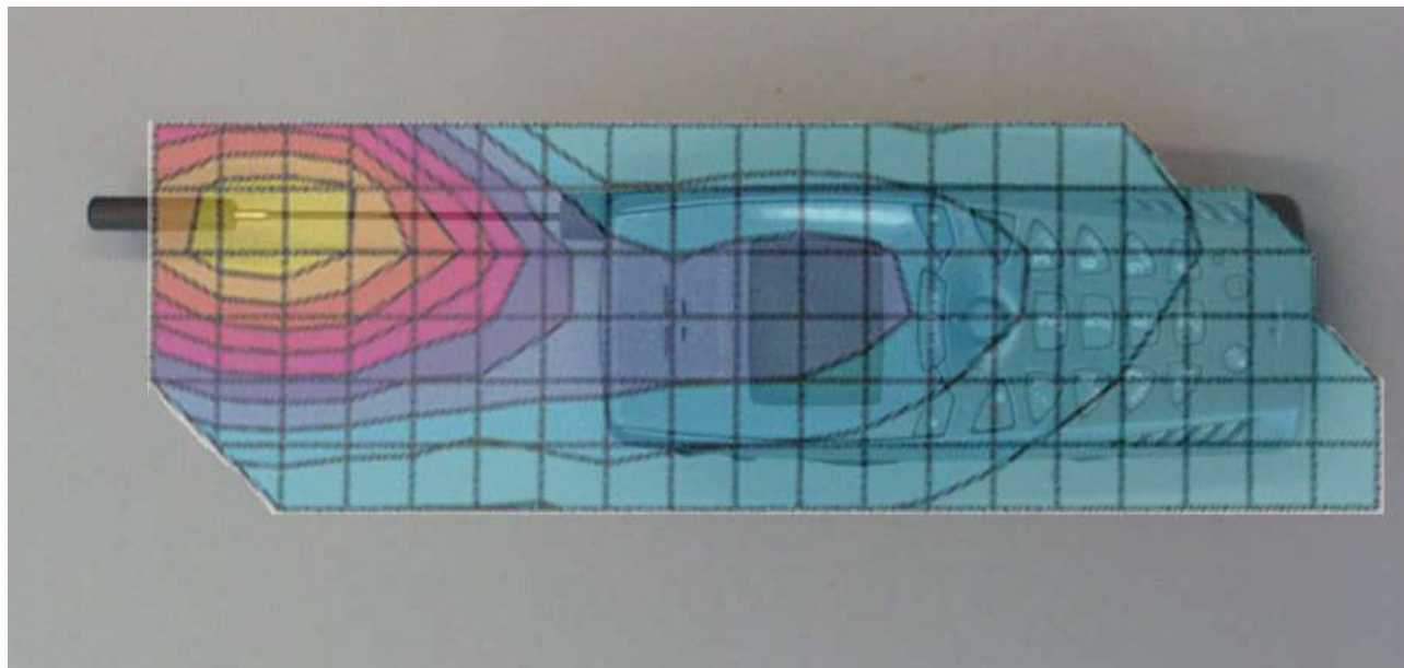
Figure 7. Typical 900MHz Phone Mode Antenna Extended Head Adjacent Contour Plot Overlaid on Face of the Phone
