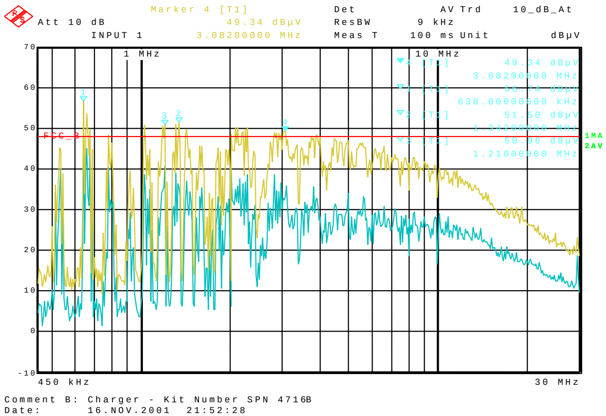
Figure 6-26: Neutral Line Voltage with a Peak and Average detector (Radio in transmit mode at 806.0625 MHz)
