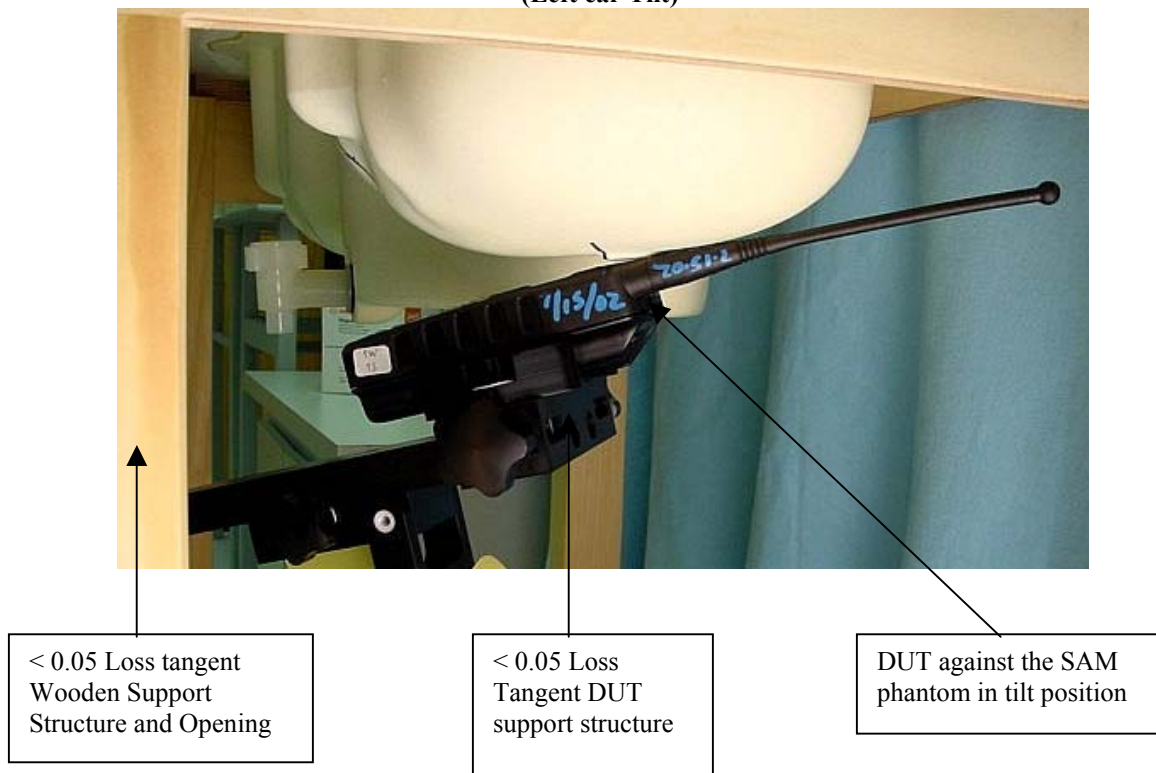
Figure 1: Highest S.A.R. Test Position (Left ear Tilt)
