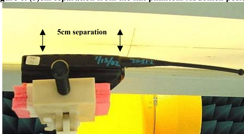
Figure 6. (5)cm separation from the flat phantom Abdomen position
