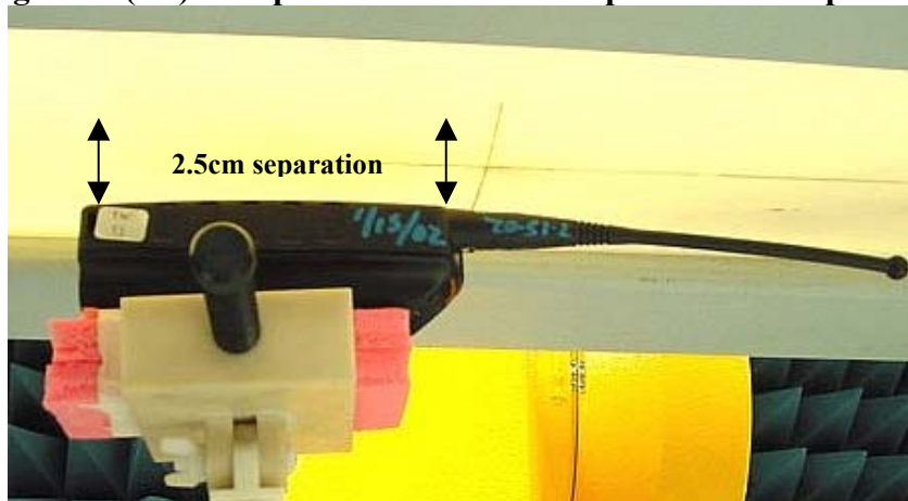
Figure 5. (2.5)cm separation from the flat phantom Face position
