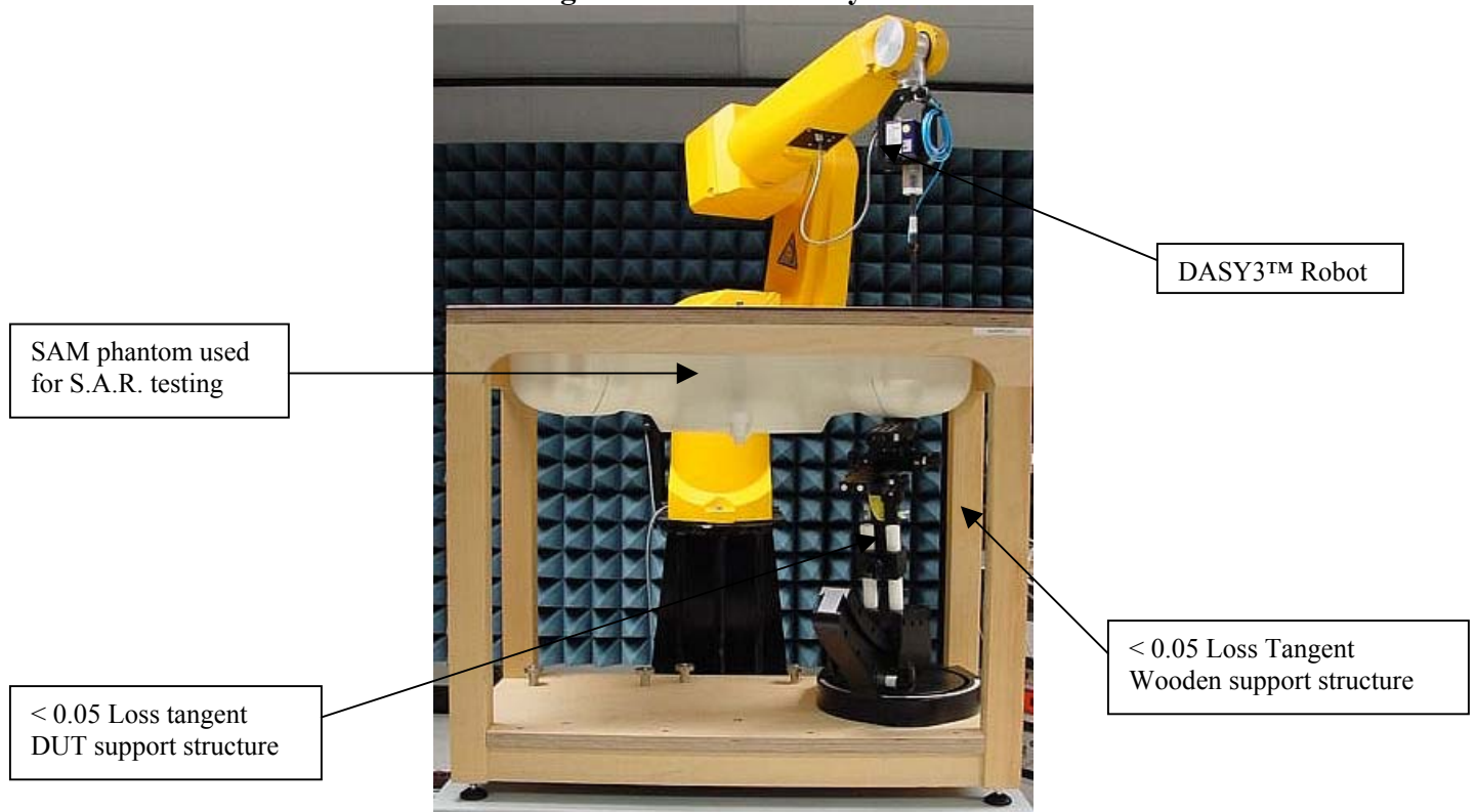
Figure 8: Robot Test System
