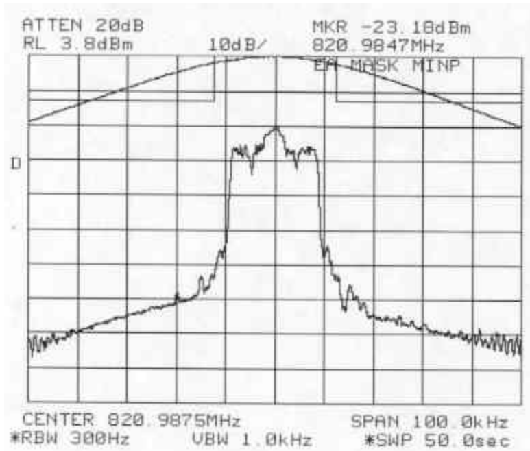
Figure 6-12b: Quad-16QAM Modulation performance relative to mask 47 CFR 90.691. (MINIMUM POWER SETTING) (Split 3:1 Interleaving)
