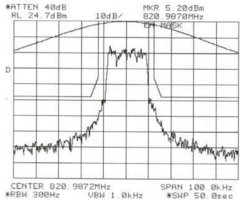
Figure 6-11a: Quad-16QAM Modulation performance relative to mask 47 CFR 90.691. (MAXIMUM POWER SETTING)
