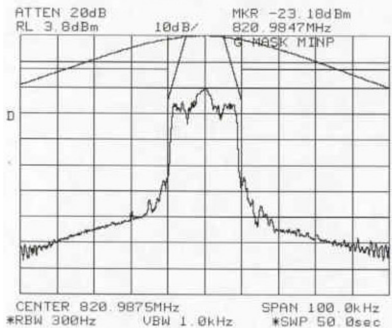
Figure 6-10a: Quad-16QAM Modulation performance relative to mask 47 CFR 90.210(g) (MINIMUM POWER SETTING)
