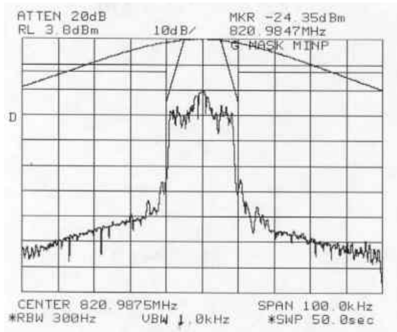
Figure 6-6: Quad-QPSK Modulation performance relative to mask 47 CFR 90.210(g) (MINIMUM POWER SETTING)
