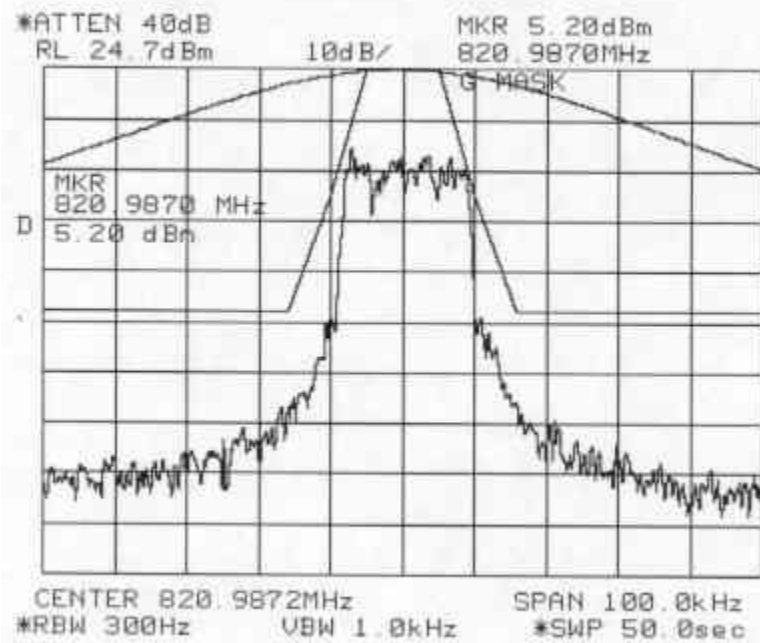
Figure 6-9b: Quad-16QAM Modulation performance relative to mask 47 CFR 90.210(g) (MAXIMUM POWER SETTING) (Split 3:1 Interleaving)
