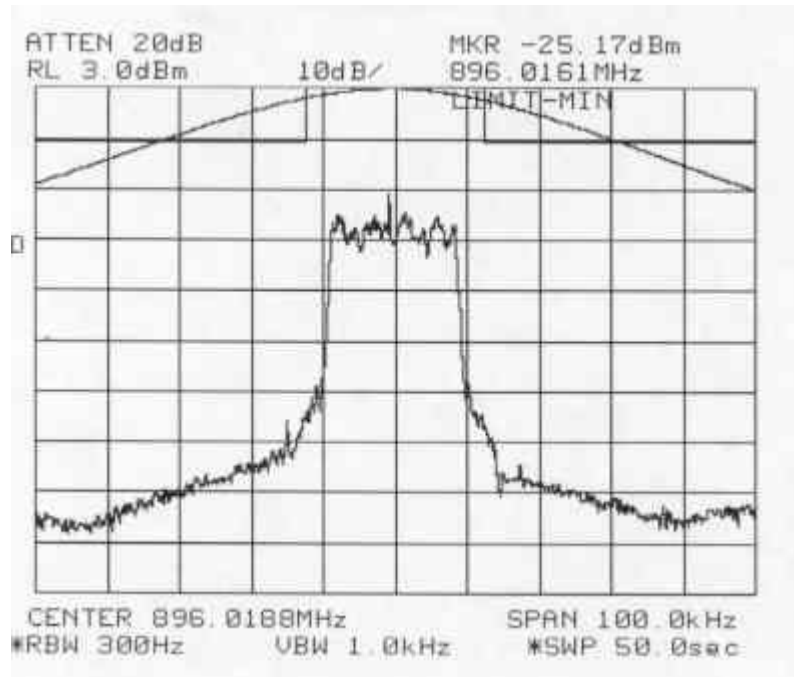
Figure 6-18: Quad-QPSK Modulation performance relative to mask 47 CFR 90.669(a) (MINIMUM POWER SETTING)
