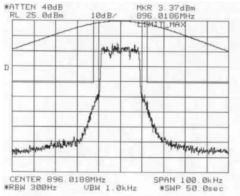
Figure 6-19a: Quad-16QAM Modulation performance relative to mask 47 CFR 90.669(a) (MAXIMUM POWER SETTING)
