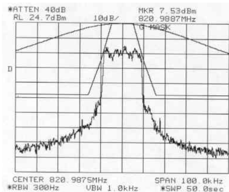
Figure 6-5: Quad-QPSK Modulation performance relative to mask 47 CFR 90.210(g) (MAXIMUM POWER SETTING)
