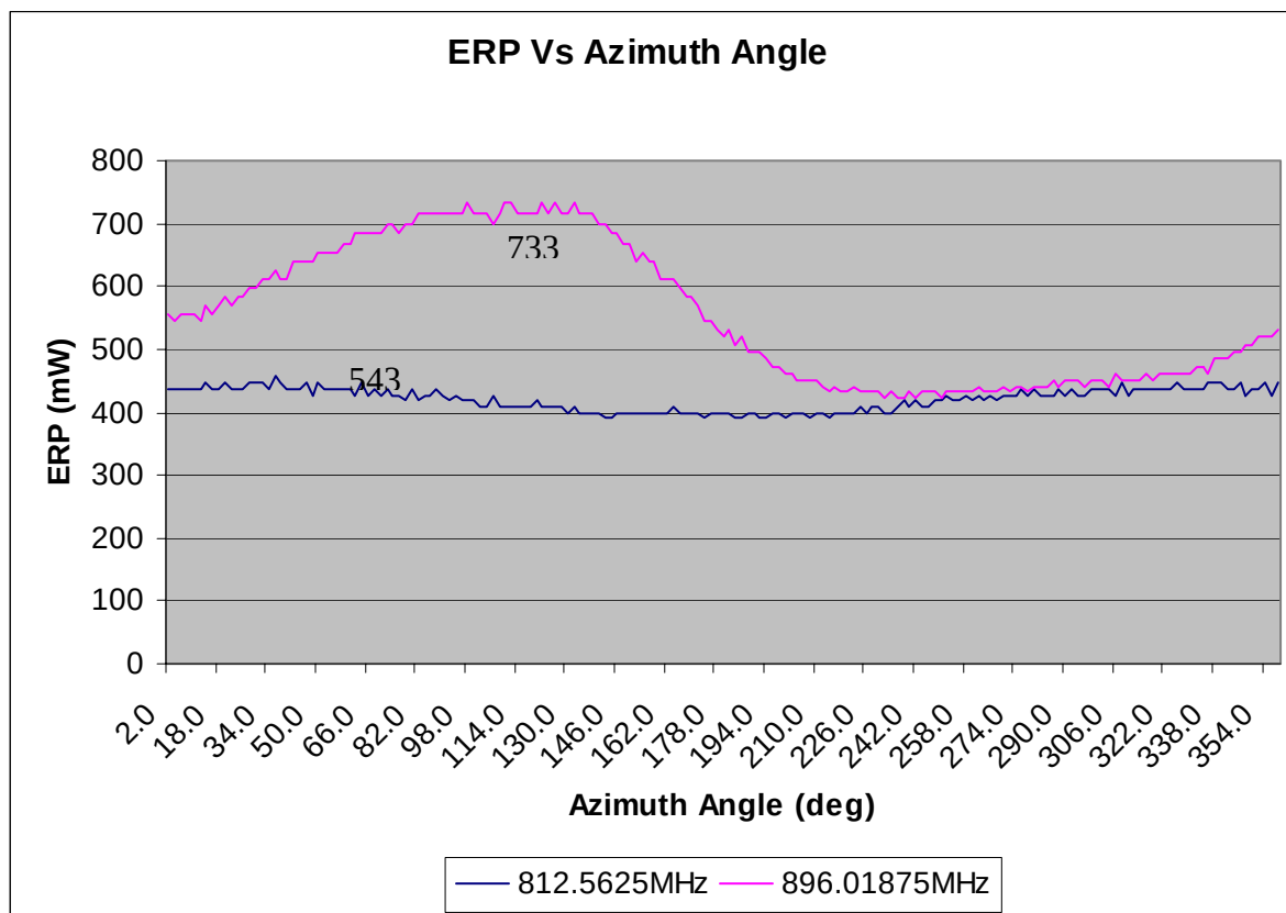
Figure 6-37: Scaled ERP vs. Azimuth Angle
