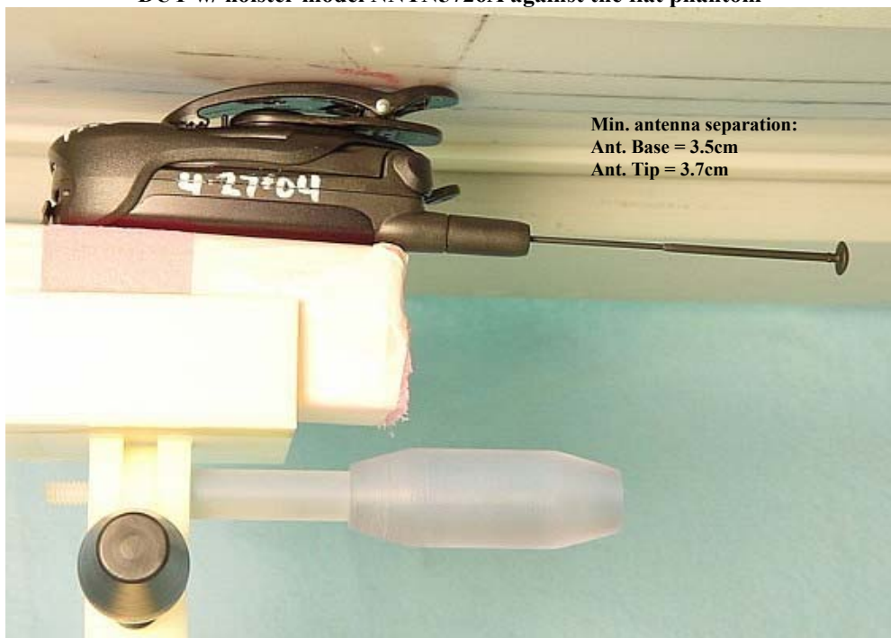
Figure 8. Assessment @ Body DUT w/ holster model NNTN5726A against the flat phantom
