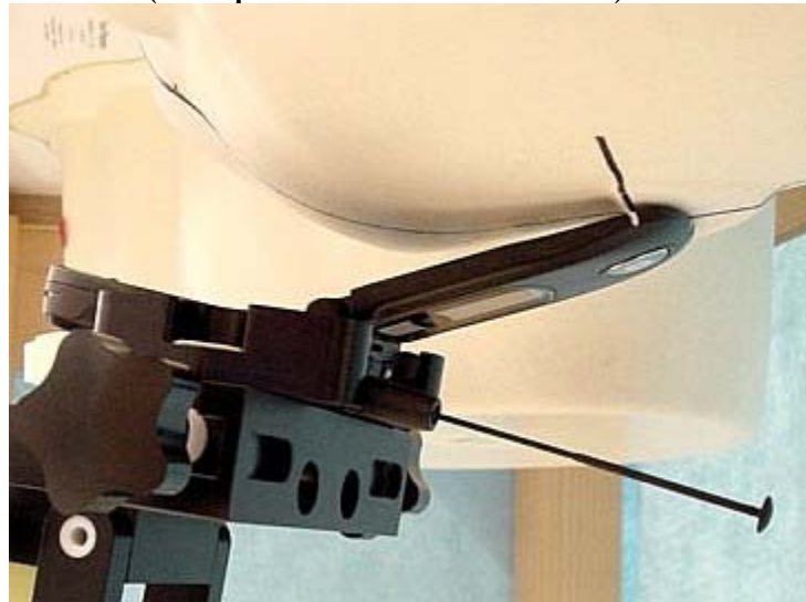
Figure 2. Assessment @ the Left ear DUT in 15° tilt position (Same position for antenna retracted)
