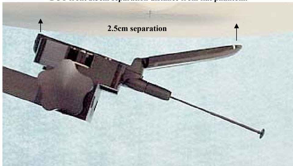
Figure 6. Assessment @ the Face (Flip opened) DUT front 2.5cm separation distance from flat phantom.
