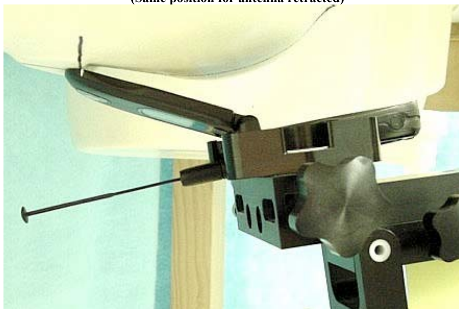
Figure 4. Assessment @ the Right ear DUT in 15° tilt position (Same position for antenna retracted)
