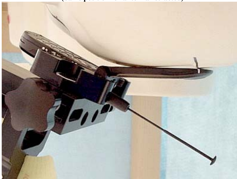
Figure 3. Assessment @ the Left ear DUT in Cheek touch position (Same position for antenna retracted)
