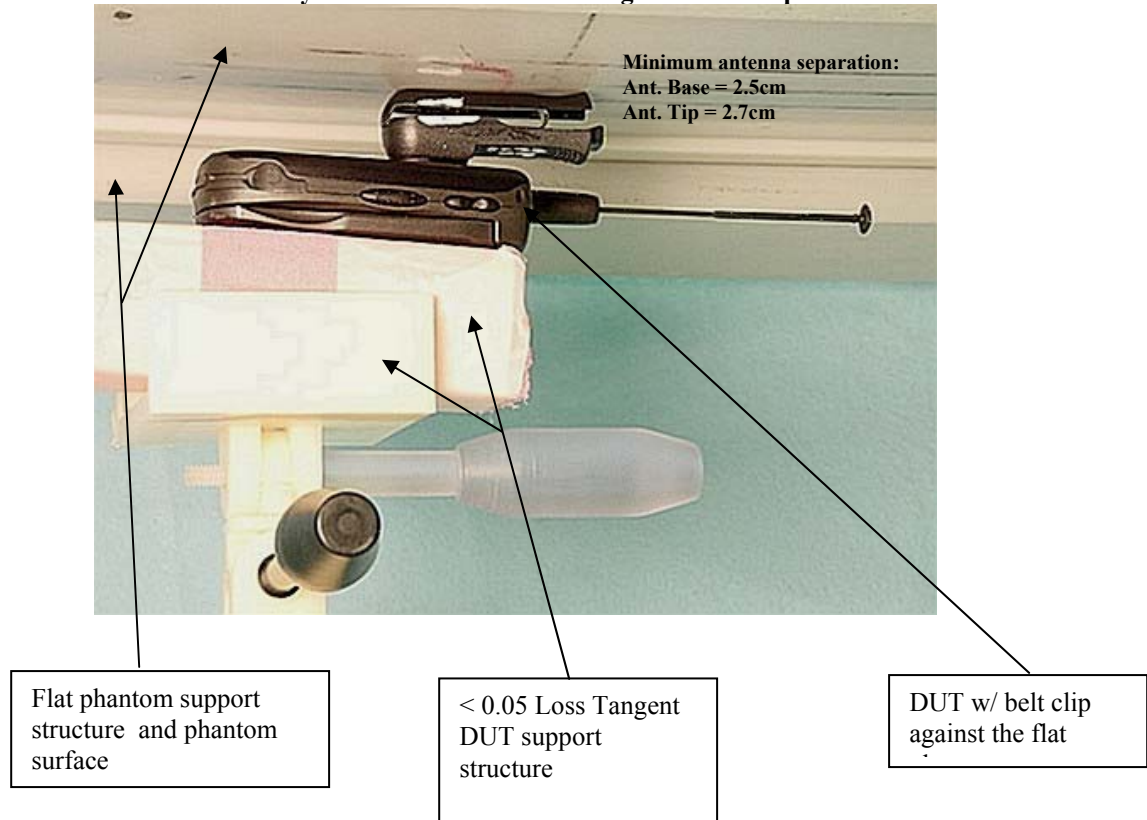
Figure 1: Highest S.A.R. Test Position (@ body) DUT with carry case model NNTN4747A against the flat phantom.
