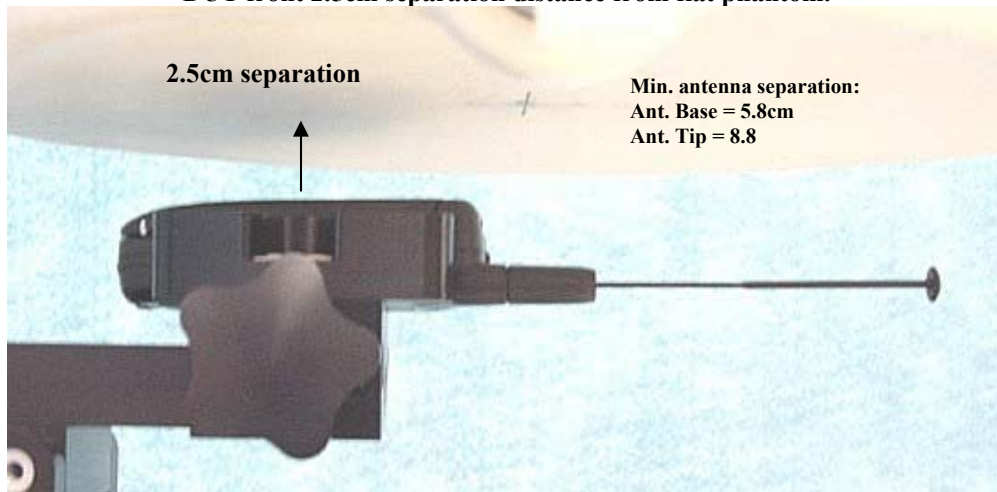
Figure 7. Assessment @ the Face (Flip closed) DUT front 2.5cm separation distance from flat phantom.
