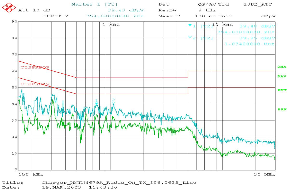
Figure 6-35: Phase Line Voltage with a Peak and Average Detector (Radio in transmit mode at 806.0625 MHz)
