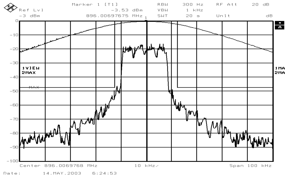
Figure 6-19a: Quad-16QAM Modulation performance relative to mask 47 CFR 90.669(a) (MAXIMUM POWER SETTING)
