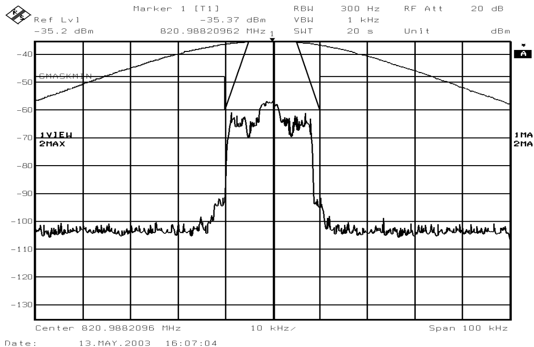
Figure 6-13: Quad-64QAM Modulation performance relative to mask 47 CFR 90.210(g) (MAXIMUM POWER SETTING)
