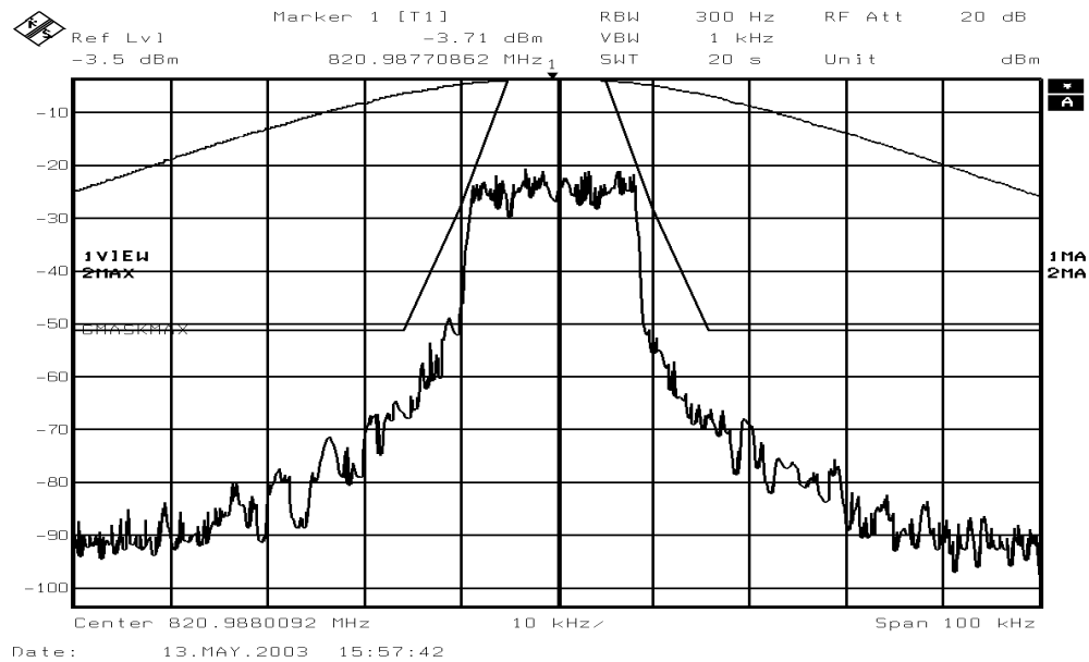
Figure 6-13: Quad-64QAM Modulation performance relative to mask 47 CFR 90.210(g) (MAXIMUM POWER SETTING)
