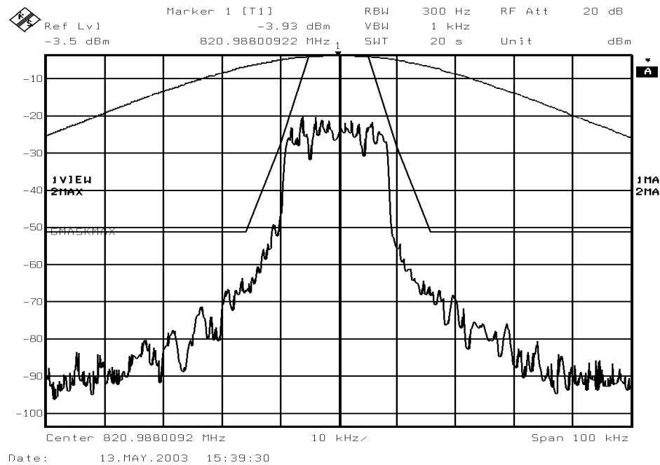
Figure 6-9a: Quad-16QAM Modulation performance relative to mask 47 CFR 90.210(g) (MAXIMUM POWER SETTING)
