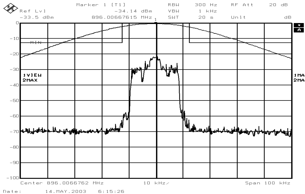
Figure 6-19a: Quad-16QAM Modulation performance relative to mask 47 CFR 90.669(a) (MAXIMUM POWER SETTING)
