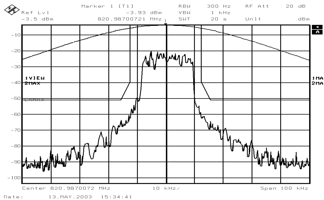
Figure 6-11a: Quad-16QAM Modulation performance relative to mask 47 CFR 90.691. (MAXIMUM POWER SETTING)
