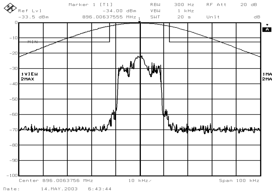
Figure 6-22: Quad-64QAM Modulation performance relative to mask 47 CFR 90.669(a) (MINIMUM POWER SETTING)
