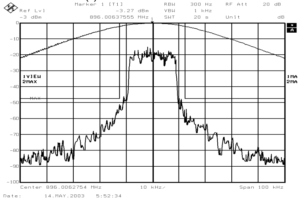
Figure 6-17: Quad-QPSK Modulation performance relative to mask 47 CFR 90.669(a)
