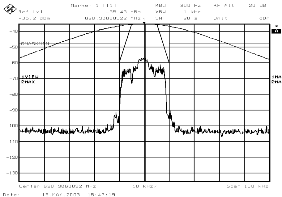
Figure 6-10a: Quad-16QAM Modulation performance relative to mask 47 CFR 90.210(g) (MINIMUM POWER SETTING)
