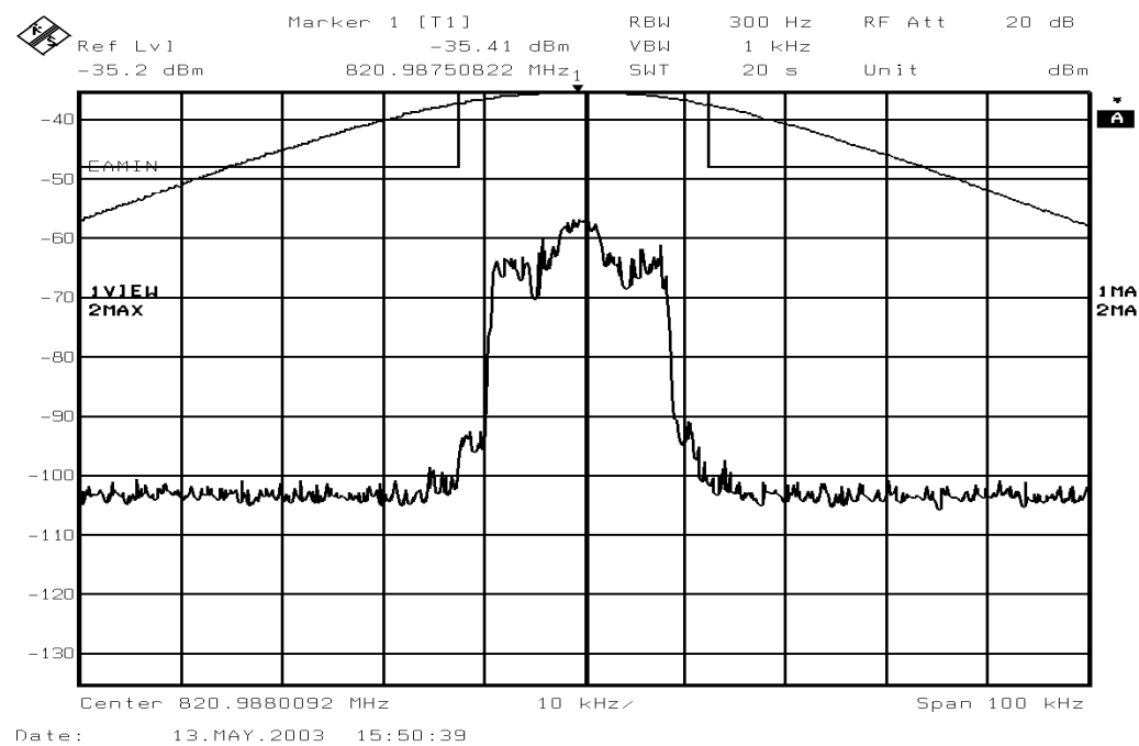
Figure 6-11a: Quad-16QAM Modulation performance relative to mask 47 CFR 90.691. (MAXIMUM POWER SETTING)
