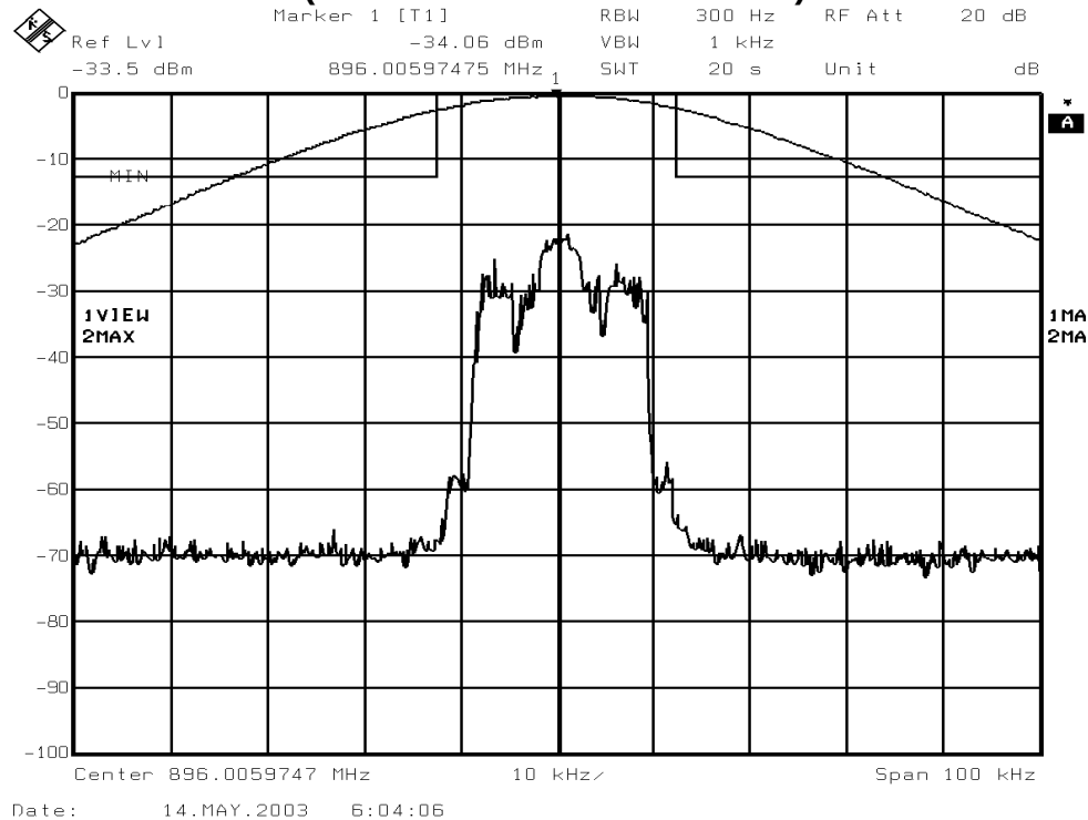
Figure 6-18: Quad-QPSK Modulation performance relative to mask 47 CFR 90.669(a) (MINIMUM POWER SETTING)
