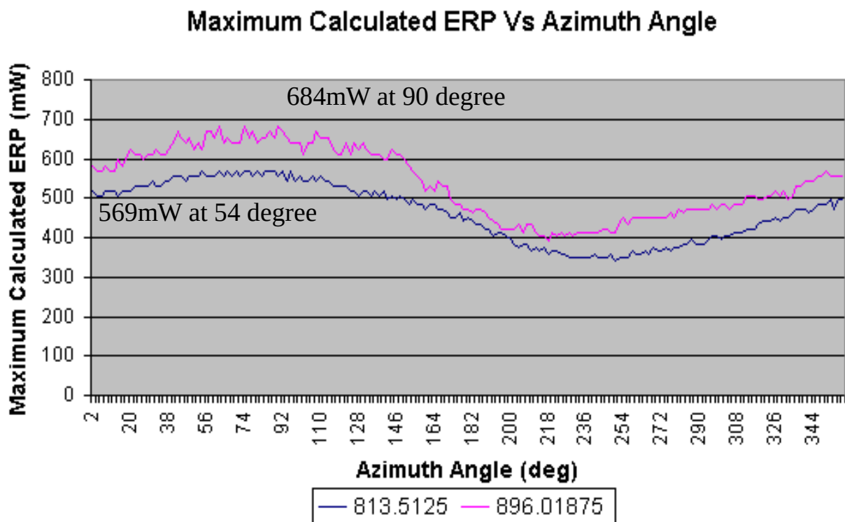
Figure 6-37: Figure 6-37: Scaled ERP vs. Azimuth Angle
