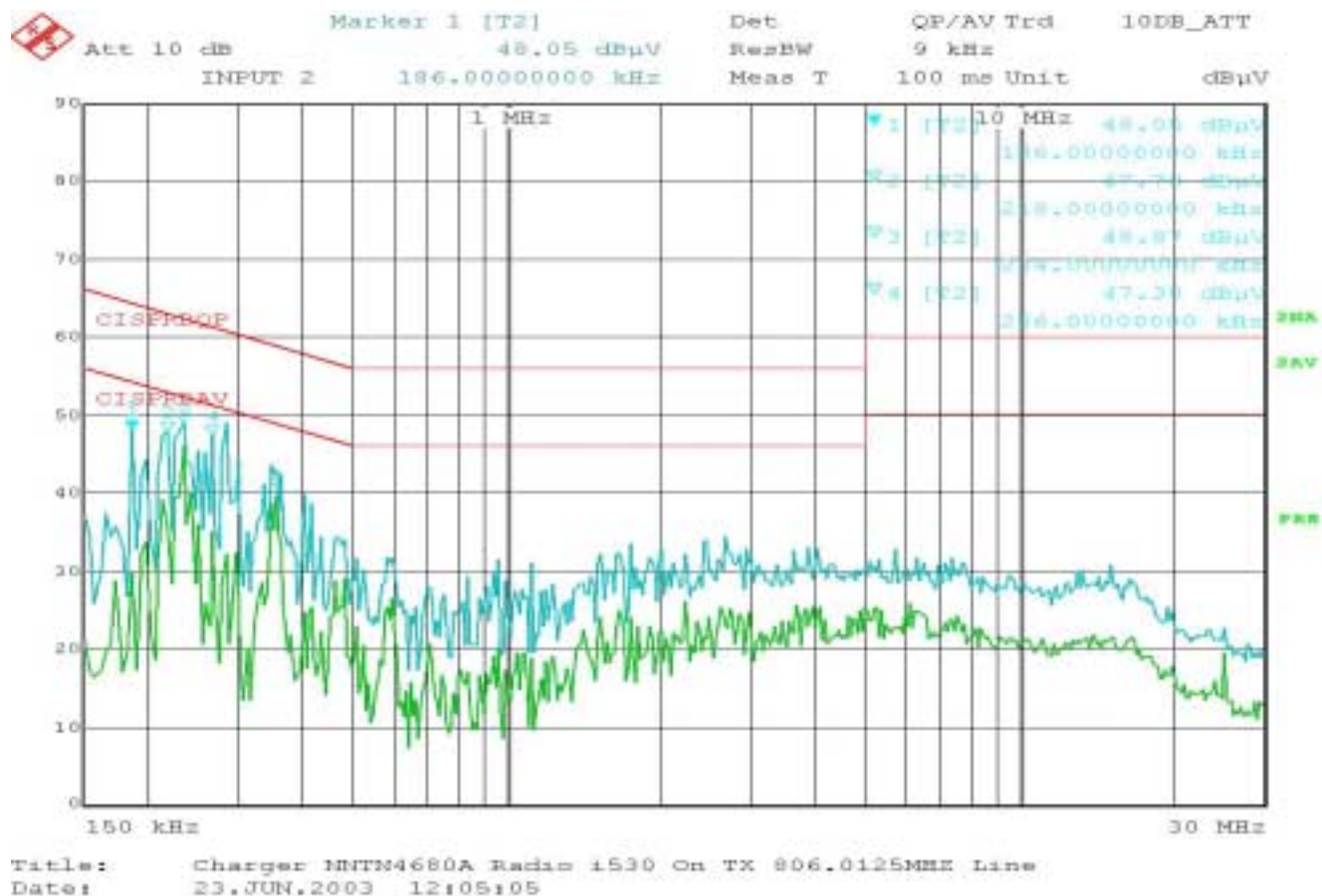
Figure 6-35: Phase Line Voltage with a Peak and Average Detector (Radio in transmit mode at 806.0125 MHz)
