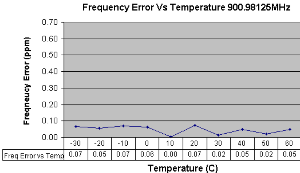
Figure 6-32: Transmitter Frequency Stability (900 MHz band) – Frequency Error vs. Temperature
