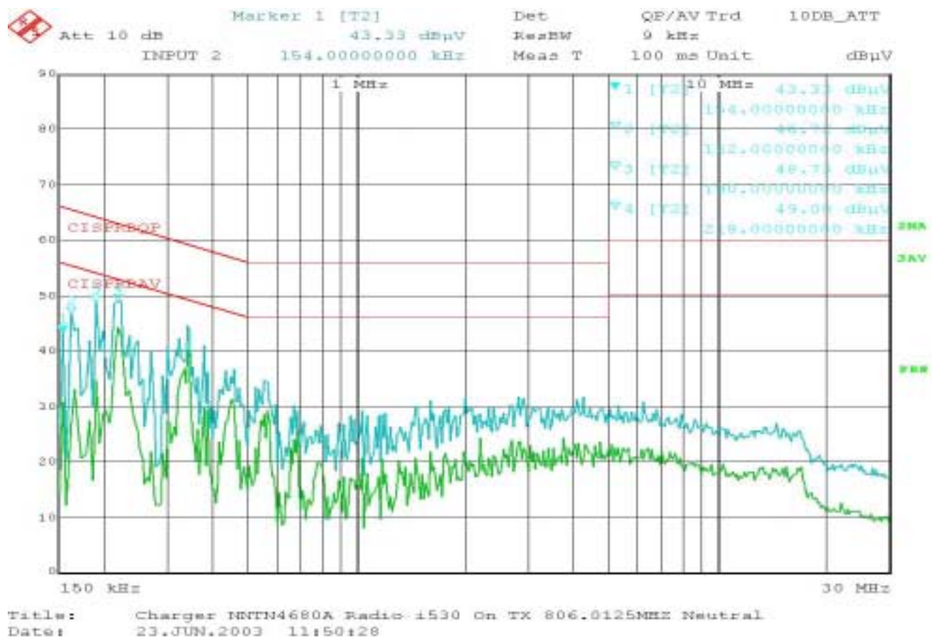
Figure 6-36: Neutral Line Voltage with a Peak and Average detector (Radio in transmit mode at 806.0125 MHz)
