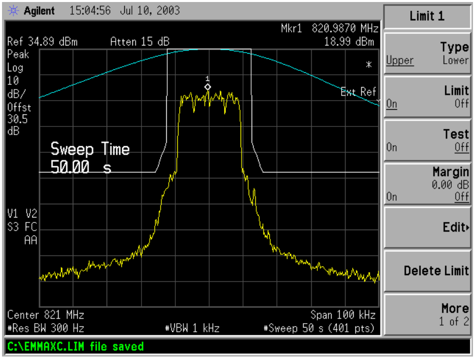
Figure 6-15: Quad-64QAM Modulation performance relative to mask 47 CFR 90.691. (MAXIMUM POWER SETTING)
