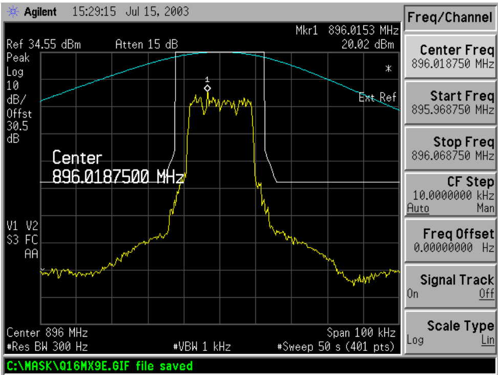
Figure 6-17: Quad-QPSK Modulation performance relative to mask 47 CFR 90.669(a) (MAXIMUM POWER SETTING)
