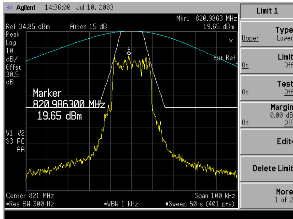
Figure 6-13: Quad-64QAM Modulation performance relative to mask 47 CFR 90.210(g) (MAXIMUM POWER SETTING)
