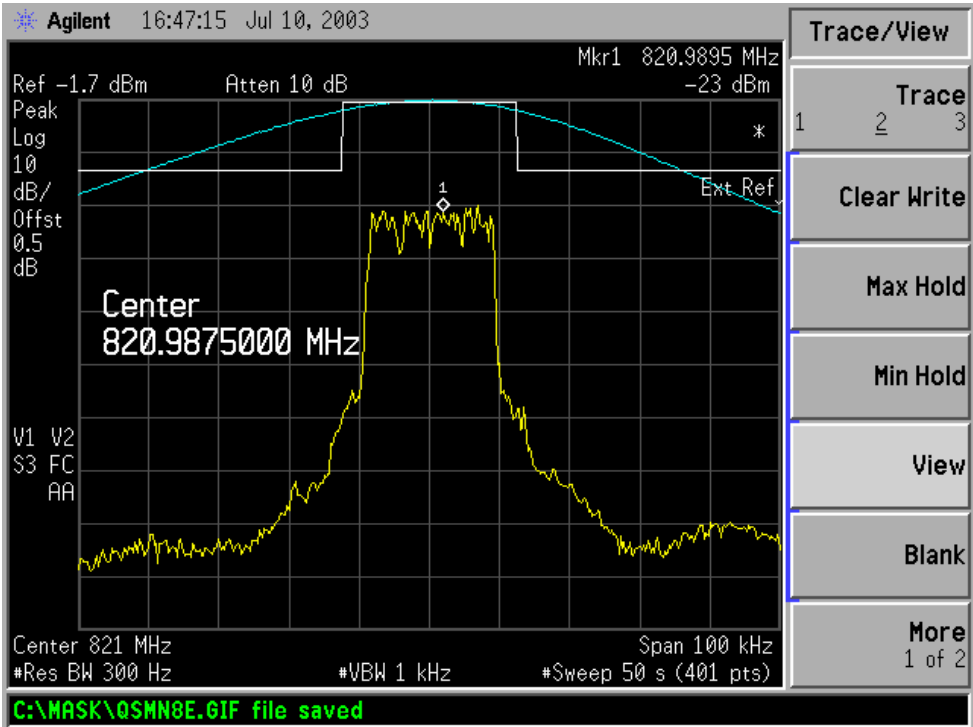
Figure 6-12a: Quad-16QAM Modulation performance relative to mask 47 CFR 90.691. (MINIMUM POWER SETTING)
