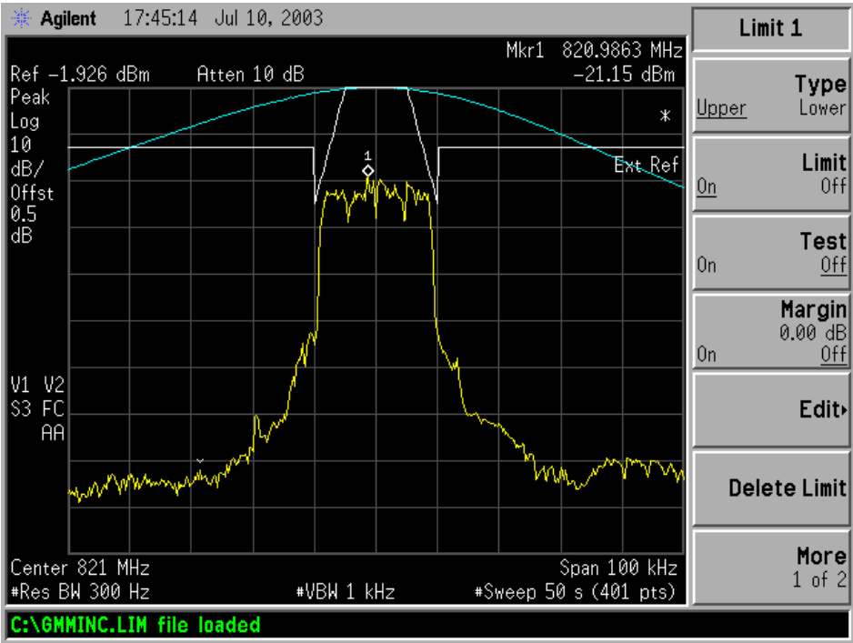
Figure 6-14: Quad-64QAM Modulation performance relative to mask 47 CFR 90.210(g) (MINIMUM POWER SETTING)
