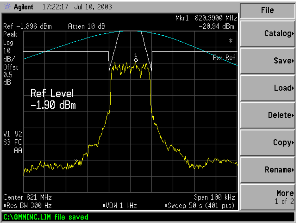
Figure 6-10b: Quad-16QAM Modulation performance relative to mask 47 CFR 90.210(g) (MINIMUM POWER SETTING) (Split 3:1 Interleaving)
