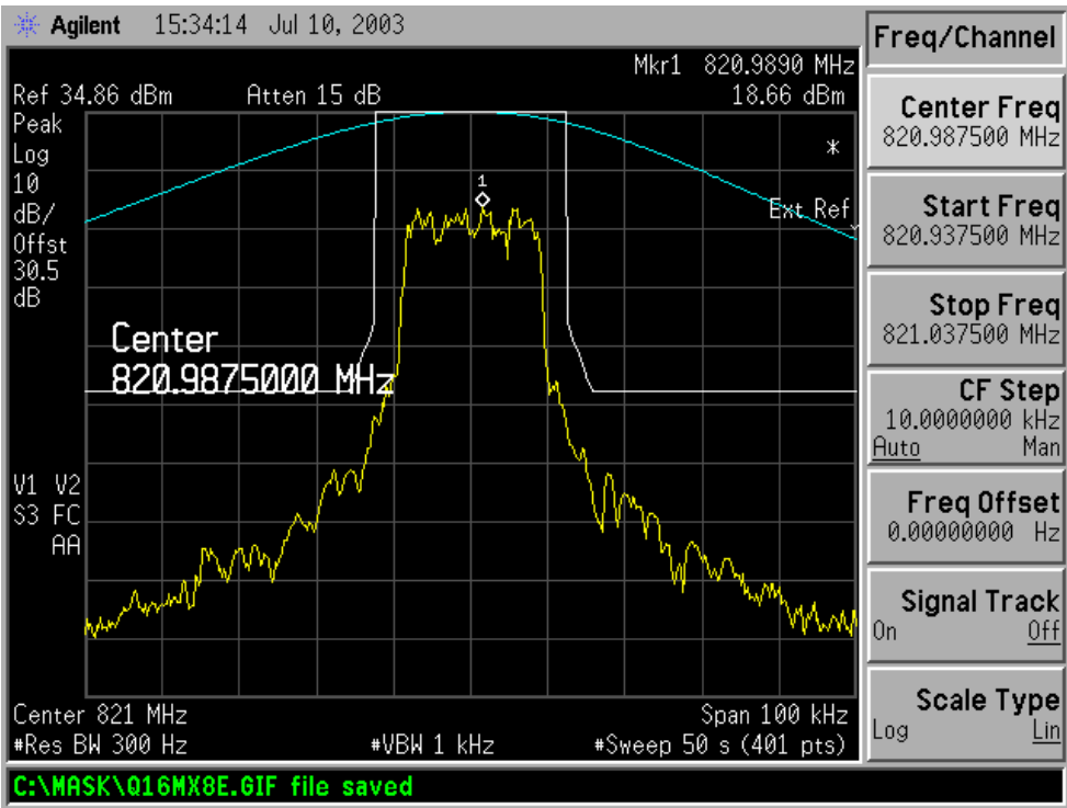
Figure 6-11b: Quad-16QAM Modulation performance relative to mask 47 CFR 90.691. (MAXIMUM POWER SETTING) (Split 3:1 Interleaving)
