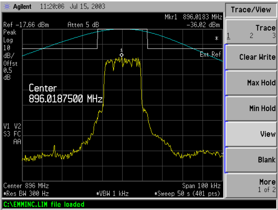
Figure 6-20a: Quad-16QAM Modulation performance relative to mask 47 CFR 90.669(a) (MINIMUM POWER SETTING)
