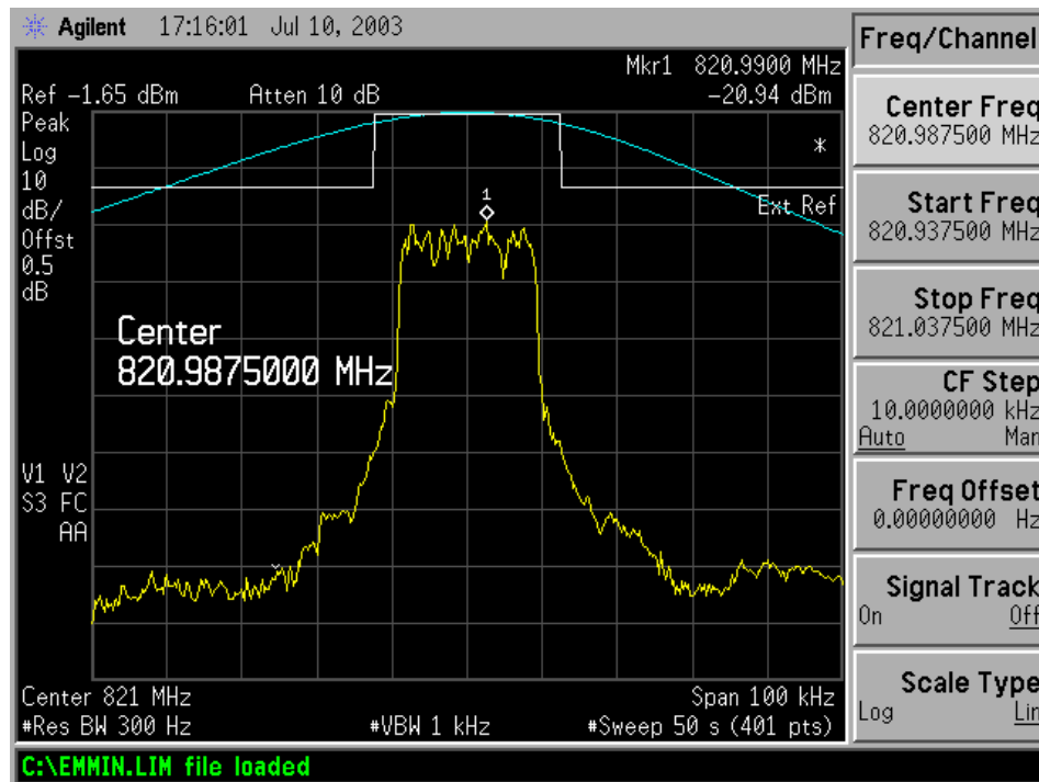
Figure 6-12b: Quad-16QAM Modulation performance relative to mask 47 CFR 90.691. (MINIMUM POWER SETTING) (Split 3:1 Interleaving)
