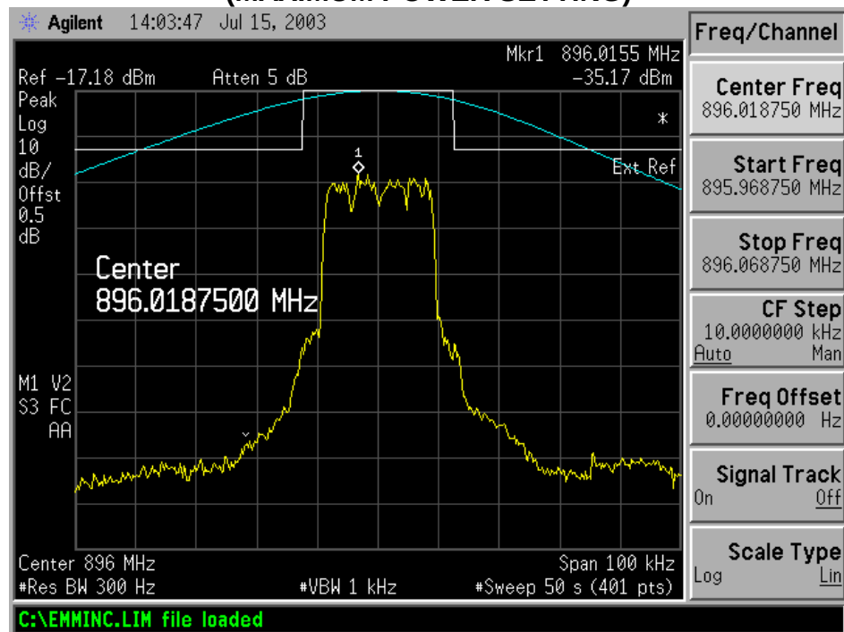
Figure 6-21: Quad-64QAM Modulation performance relative to mask 47 CFR 90.669(a) (MAXIMUM POWER SETTING)
