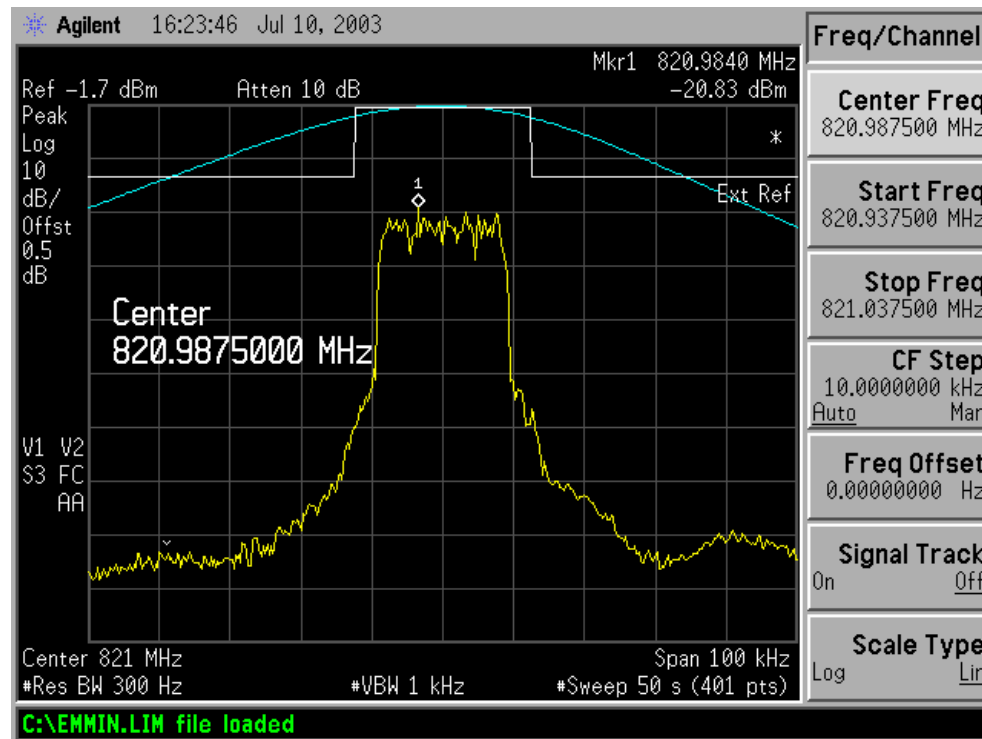
Figure 6-8: Quad-QPSK Modulation performance relative to mask 47 CFR 90.691. (MINIMUM POWER SETTING)
