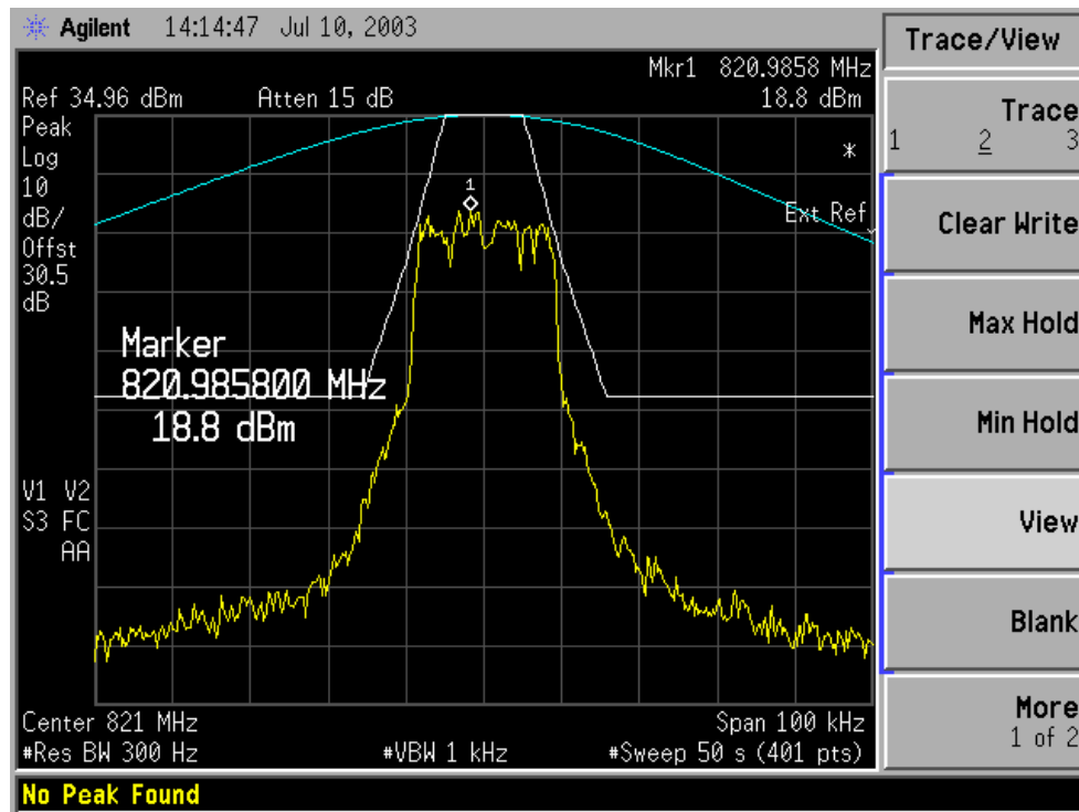
Figure 6-9b: Quad-16QAM Modulation performance relative to mask 47 CFR 90.210(g) (MAXIMUM POWER SETTING) (Split 3:1 Interleaving)
