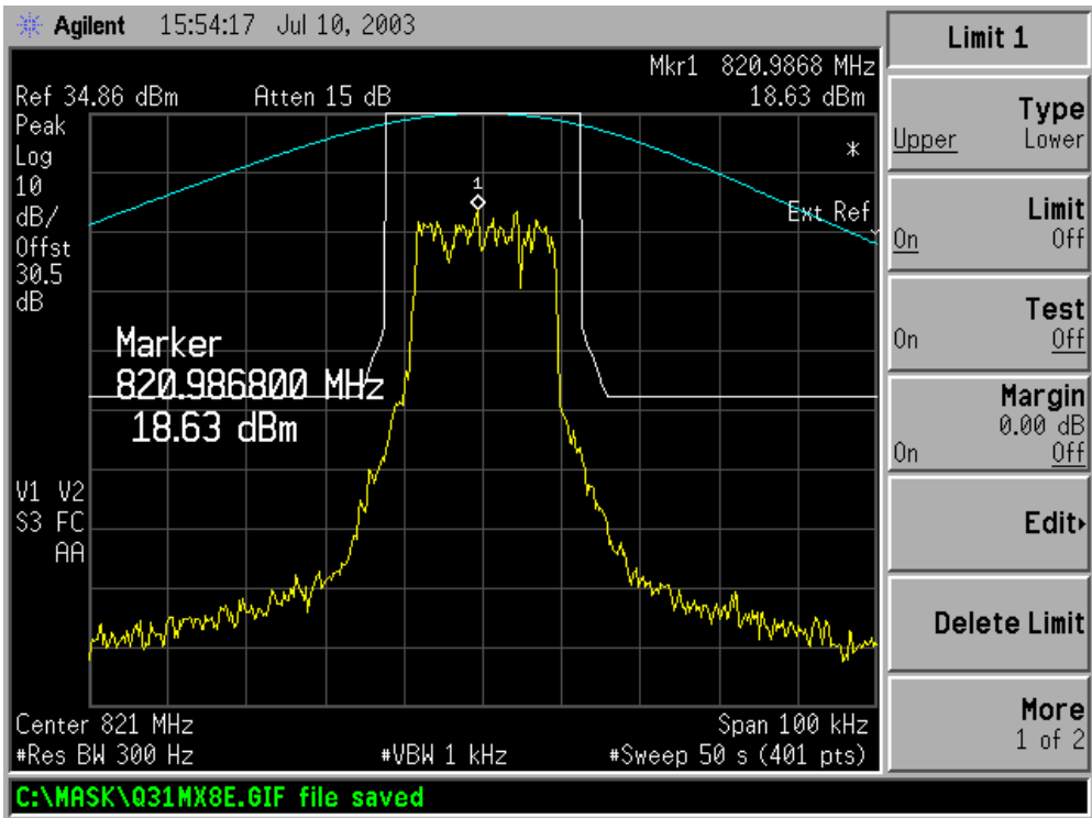
Figure 6-7: Quad-QPSK Modulation performance relative to mask 47 CFR 90.691. (MAXIMUM POWER SETTING)
