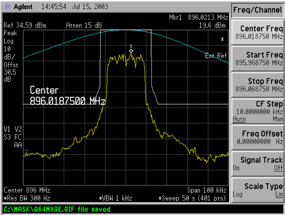
Figure 6-19b: Quad-16QAM Modulation performance relative to mask 47 CFR 90.669(a) (MAXIMUM POWER SETTING) (Split 3:1 Interleaving)
