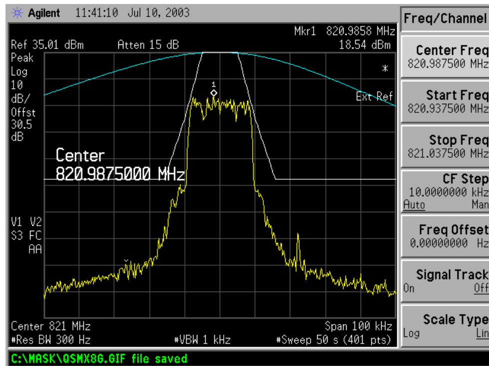
Figure 6-9a: Quad-16QAM Modulation performance relative to mask 47 CFR 90.210(g) (MAXIMUM POWER SETTING)
