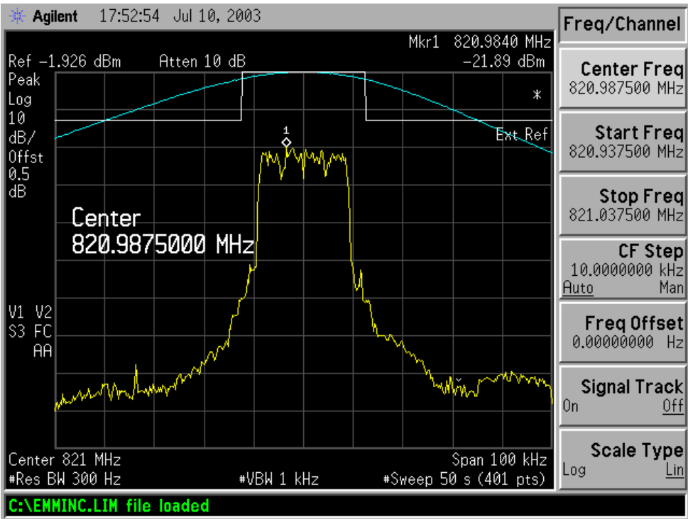
Figure 6-16: Quad-64QAM Modulation performance relative to mask 47 CFR 90.691. (MINIMUM POWER SETTING)
