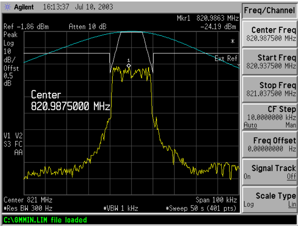
Figure 6-6: Quad-QPSK Modulation performance relative to mask 47 CFR 90.210(g) (MINIMUM POWER SETTING)
