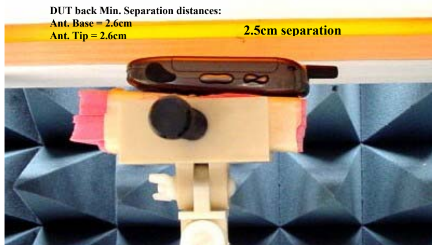
Figure 9. Assessment @ the Body DUT Back w/ 2.5cm separation.
