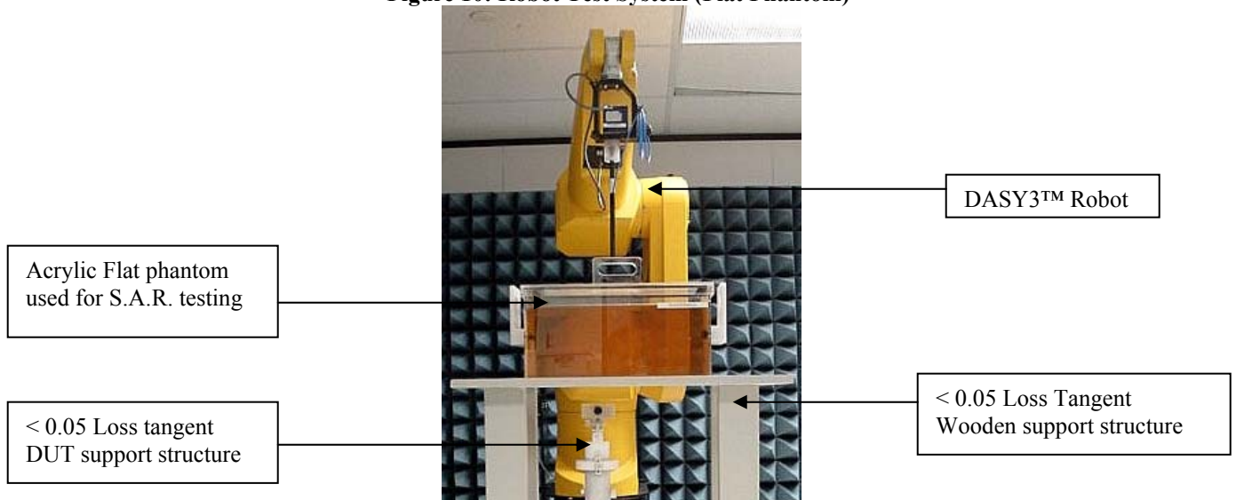
Figure 10: Robot Test System (Flat Phantom)
