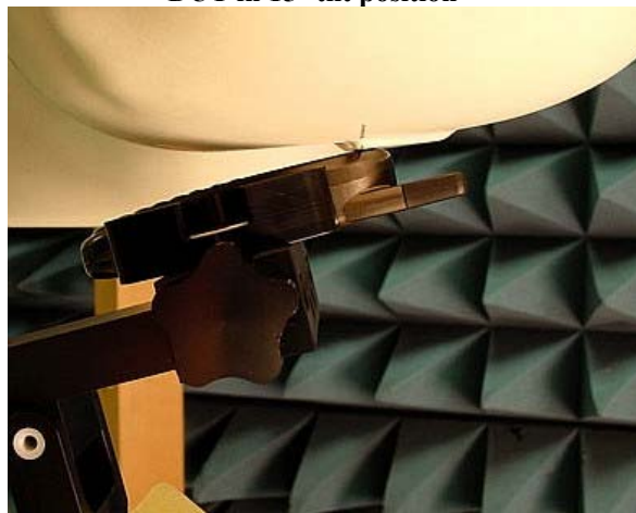
Figure 2. Assessment @ the Left ear DUT in 15° tilt position
