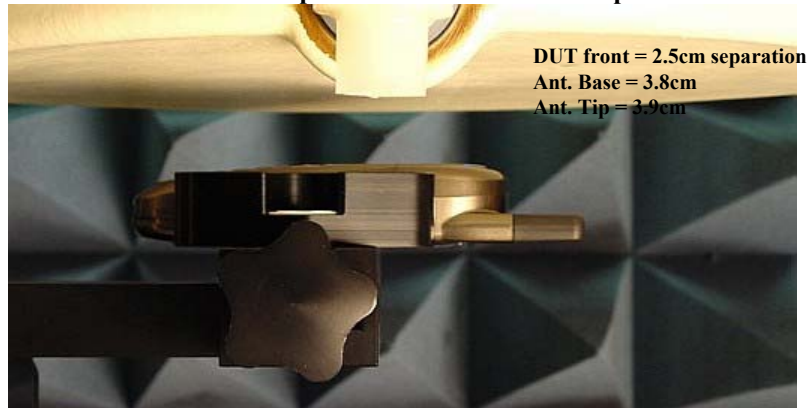
Figure 5. Assessment @ the Face DUT front 2.5cm separation distance from flat phantom.
