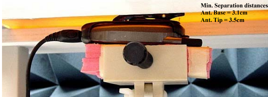
Figure 7. Assessment @ the Body DUT w/ belt clip model NNTN4747A and attached data cable model NKN6560A. (Same position used w/ data cable model NKN6559A attached, w/o any attachments, as well as w/ each of the offered audio accessories)
