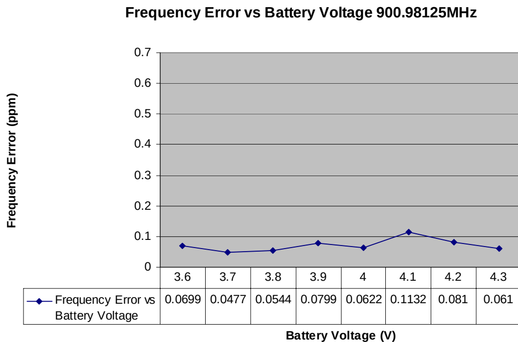
Figure 6-34: Transmitter Frequency Stability (900 MHz band)- Frequency Error vs. Voltage
