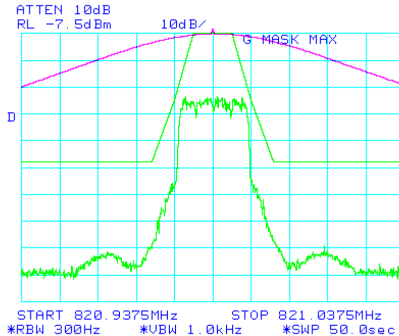
Figure 6-9a: Quad-16QAM Modulation performance relative to mask 47 CFR 90.210(g) (MAXIMUM POWER SETTING)
