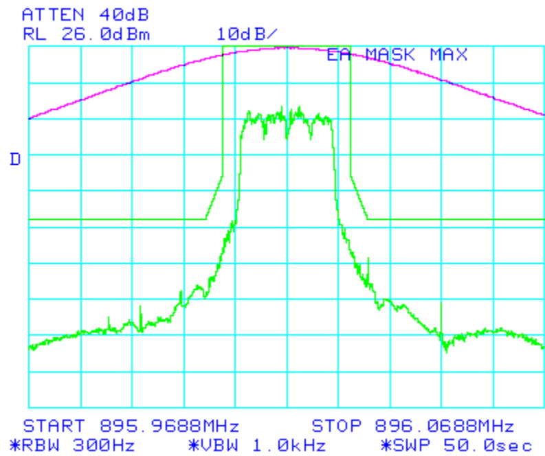
Figure 6-19b: Quad-16QAM Modulation performance relative to mask 47 CFR 90.669(a) (MAXIMUM POWER SETTING) (Split 3:1 Interleaving)
