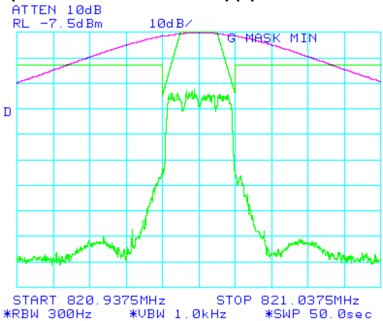
Figure 6-9b: Quad-16QAM Modulation performance relative to mask 47 CFR 90.210(g) (MAXIMUM POWER SETTING) (Split 3:1 Interleaving)
