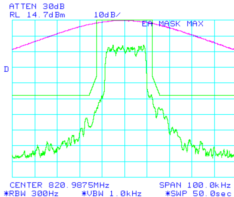
Figure 6-15: Quad-64QAM Modulation performance relative to mask 47 CFR 90.691. (MAXIMUM POWER SETTING)
