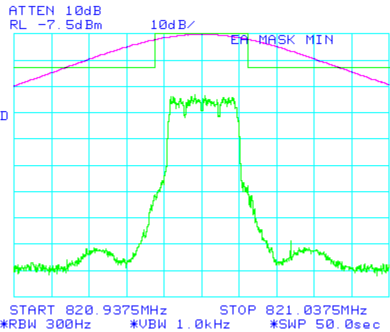
Figure 6-12a: Quad-16QAM Modulation performance relative to mask 47 CFR 90.691. (MINIMUM POWER SETTING)
