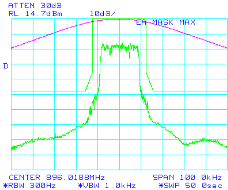
Figure 6-18: Quad-QPSK Modulation performance relative to mask 47 CFR 90.669(a) (MINIMUM POWER SETTING)
