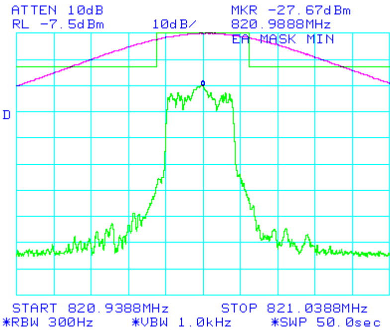
Figure 6-16: Quad-64QAM Modulation performance relative to mask 47 CFR 90.691. (MINIMUM POWER SETTING)
