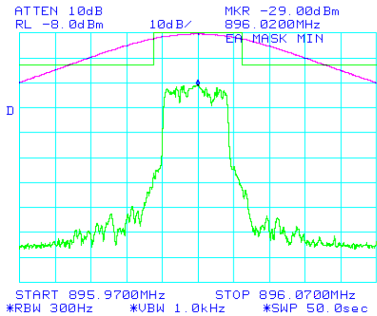
Figure 6-21: Quad-64QAM Modulation performance relative to mask 47 CFR 90.669(a) (MAXIMUM POWER SETTING)
