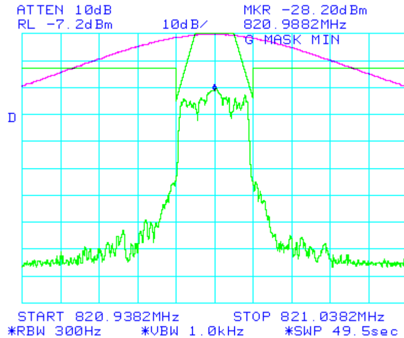
Figure 6-14: Quad-64QAM Modulation performance relative to mask 47 CFR 90.210(g) (MINIMUM POWER SETTING)
