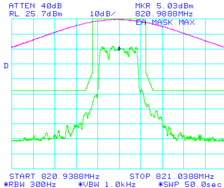
Figure 6-7: Quad-QPSK Modulation performance relative to mask 47 CFR 90.691. (MAXIMUM POWER SETTING)
