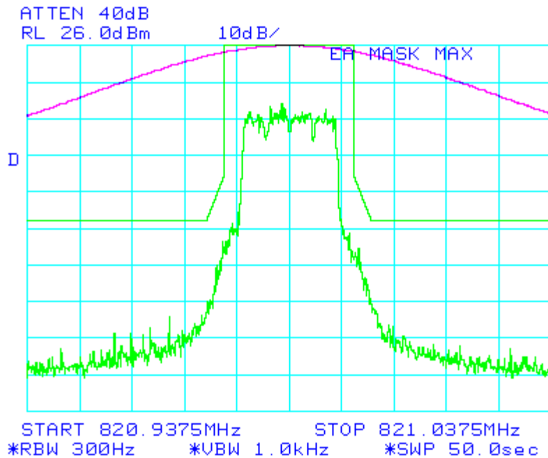
Figure 6-10b: Quad-16QAM Modulation performance relative to mask 47 CFR 90.210(g) (MINIMUM POWER SETTING) (Split 3:1 Interleaving)
