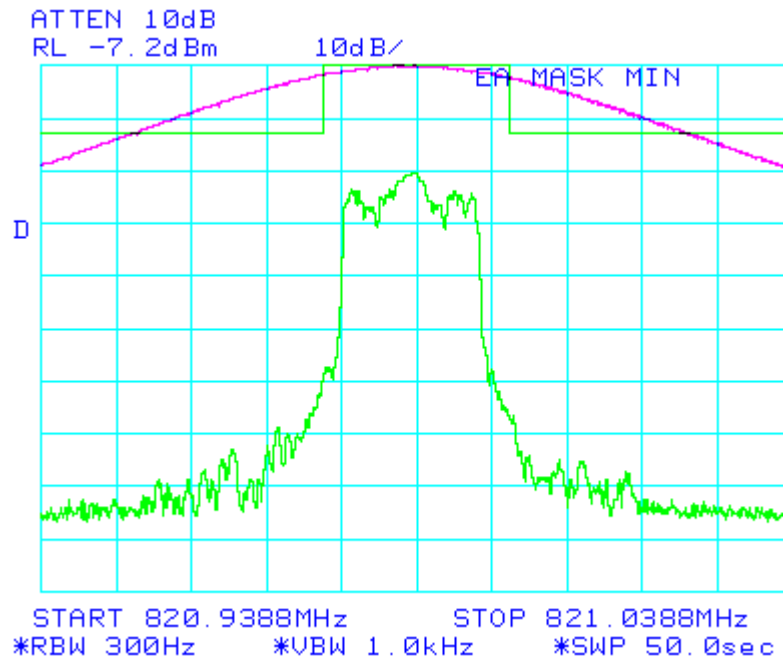
Figure 6-8: Quad-QPSK Modulation performance relative to mask 47 CFR 90.691. (MINIMUM POWER SETTING)
