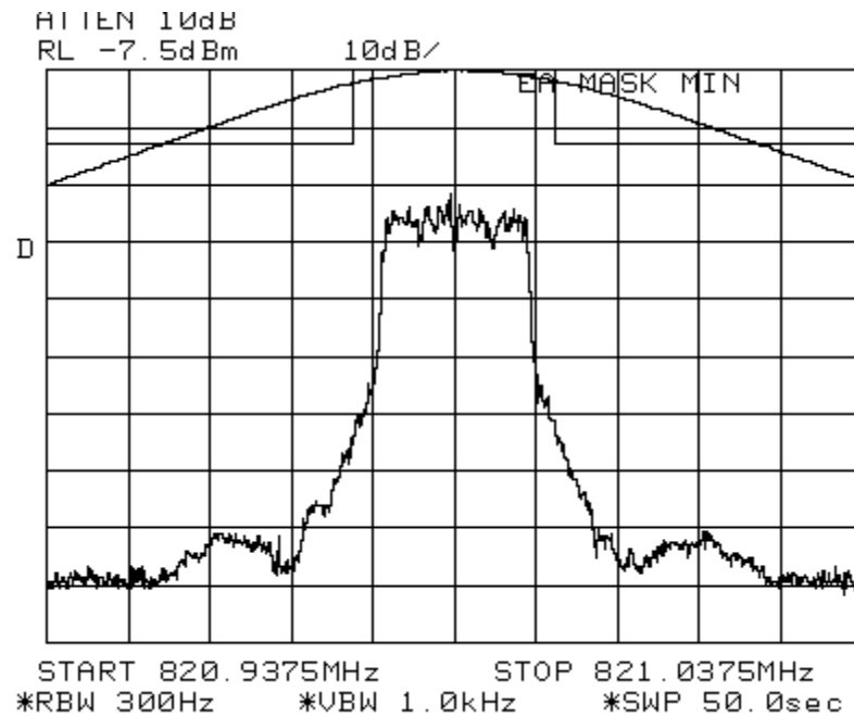
Figure 6-12b: Quad-16QAM Modulation performance relative to mask 47 CFR 90.691.
