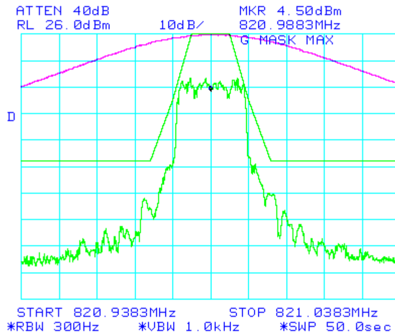
Figure 6-13: Quad-64QAM Modulation performance relative to mask 47 CFR 90.210(g)
