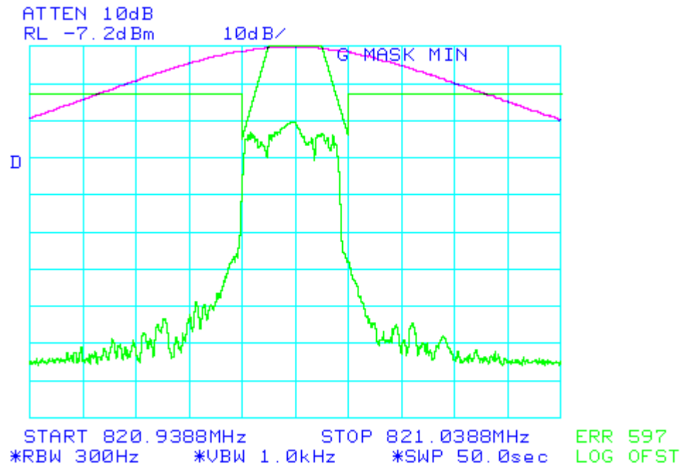
Figure 6-6: Quad-QPSK Modulation performance relative to mask 47 CFR 90.210(g) (MINIMUM POWER SETTING)
