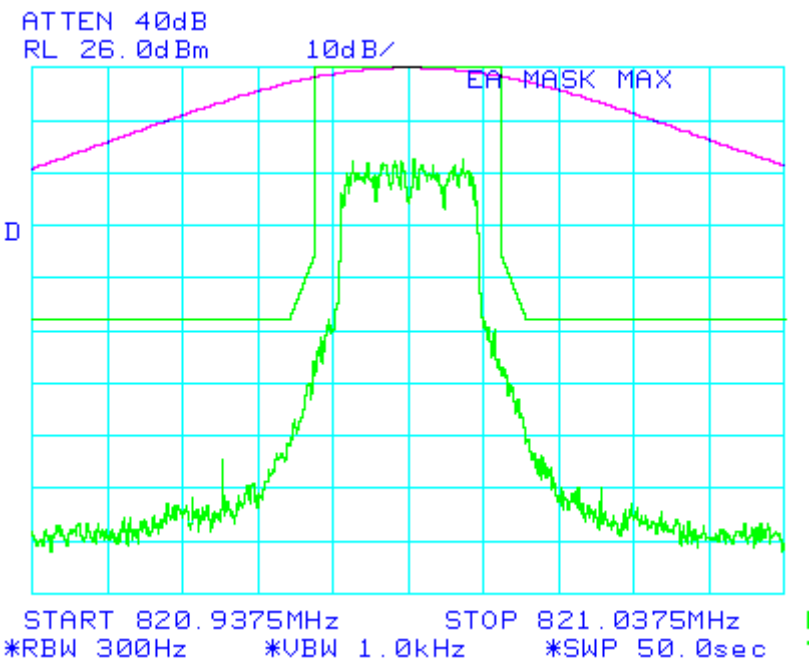
Figure 6-11b: Quad-16QAM Modulation performance relative to mask 47 CFR 90.691. (MAXIMUM POWER SETTING) (Split 3:1 Interleaving)
