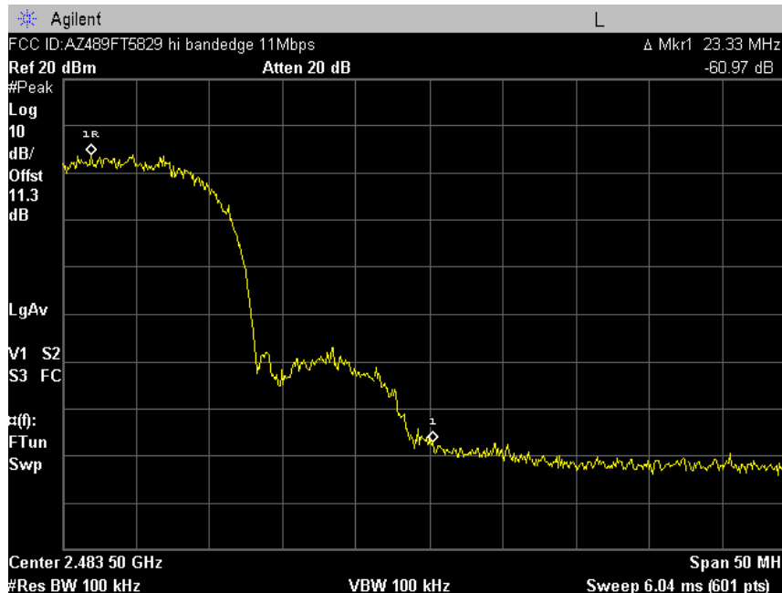
Plot A-14. Occupied Band Edge Plot – Ch. 11 – 11 Mbps
