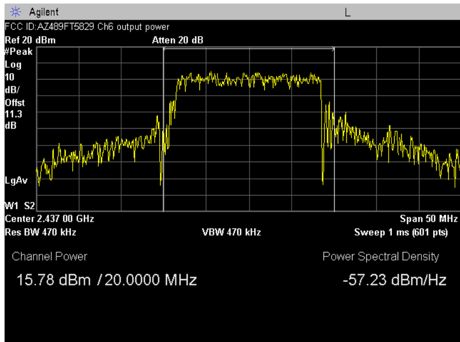
Plot A-8. Max. Output Power Plot – Ch. 06 – 36 Mbps
