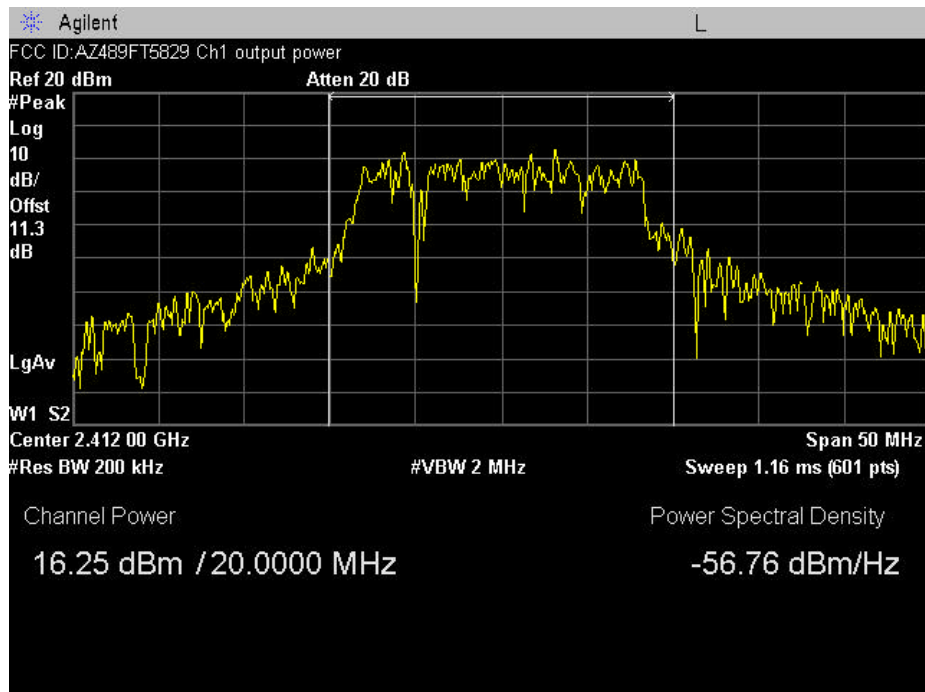
Plot A-7. Max. Output Power Plot – Ch. 01- 36 Mbps
