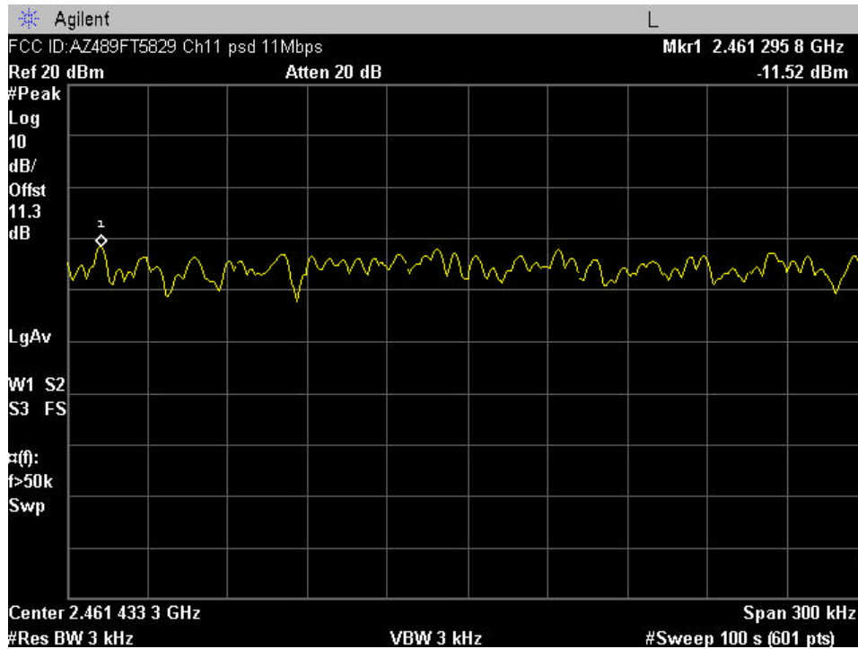
Plot A-12. Max. Power Density Plot – Ch. 11
