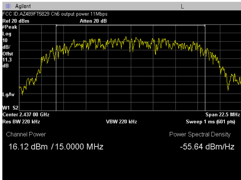
Plot A-5. Max. Output Power Plot – Ch. 06 – 11 Mbps
