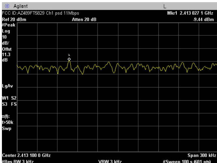
Plot A-10. Max. Power Density Plot – Ch. 01
