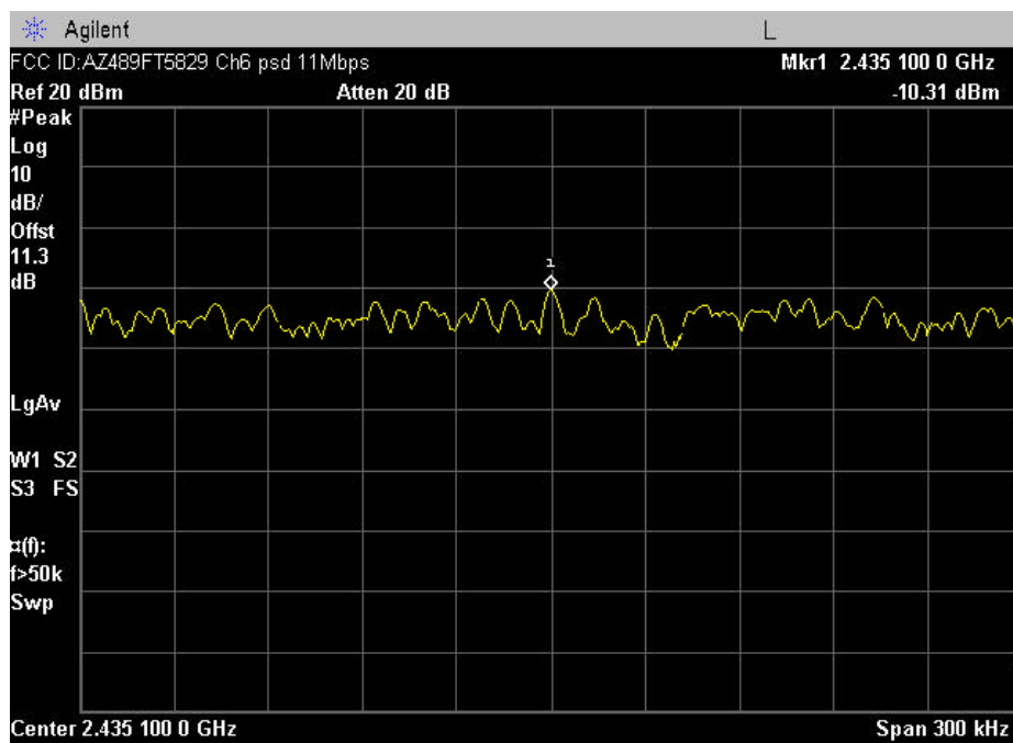
Plot A-11. Max. Power Density Plot – Ch. 06
