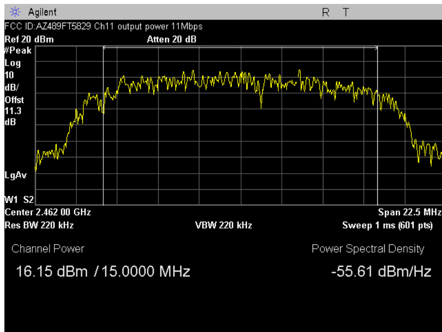
Plot A-6. Max. Output Power Plot – Ch. 11 – 11 Mbps
