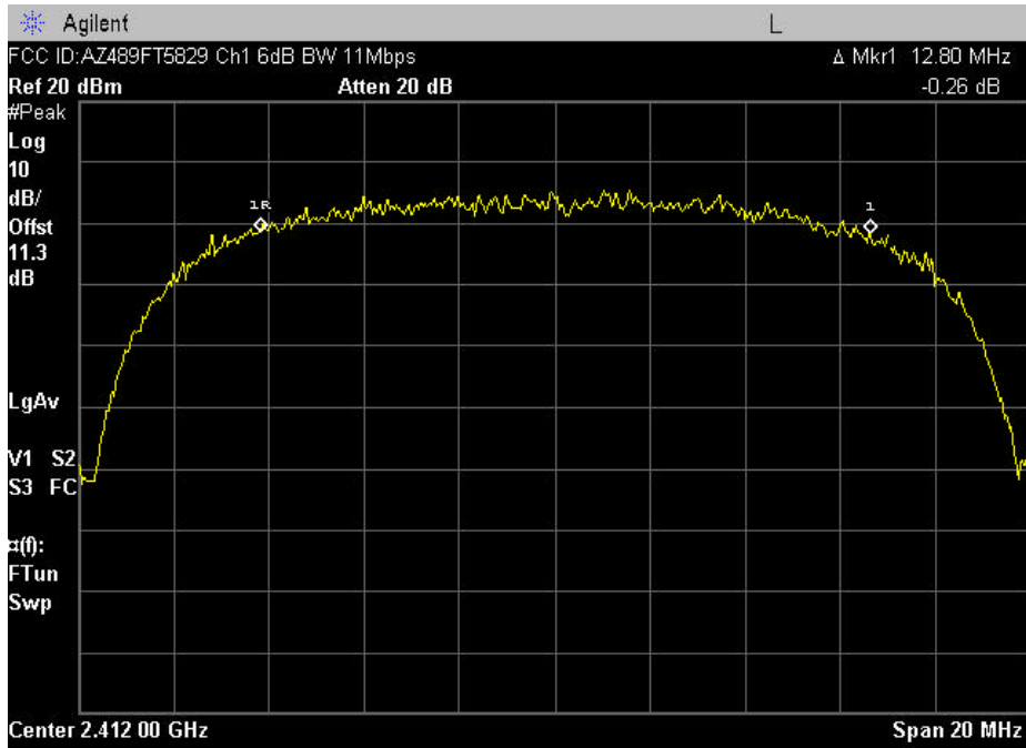
Plot A-1. 6dB Bandwidth Plot – Ch. 01
