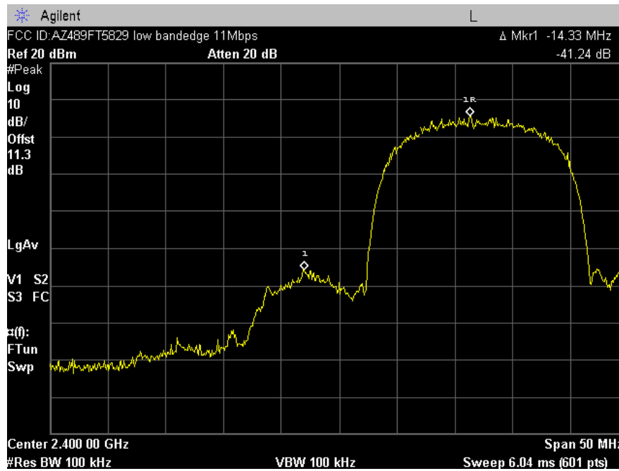
Plot A-13. Occupied Band Edge Plot – Ch. 01 – 11 Mbps
