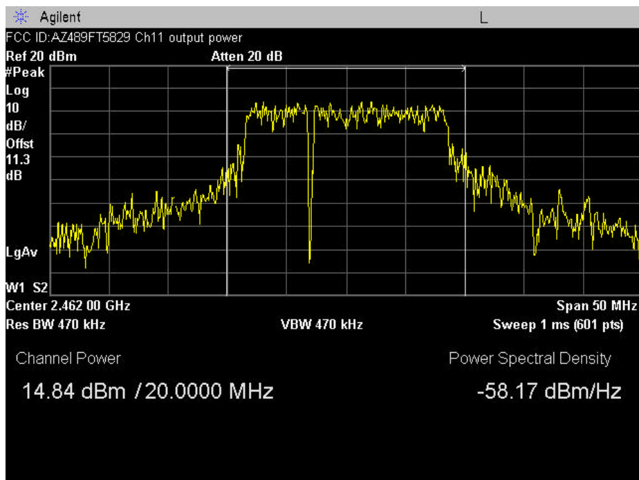
Plot A-9. Max. Output Power Plot – Ch. 11 – 36 Mbps
