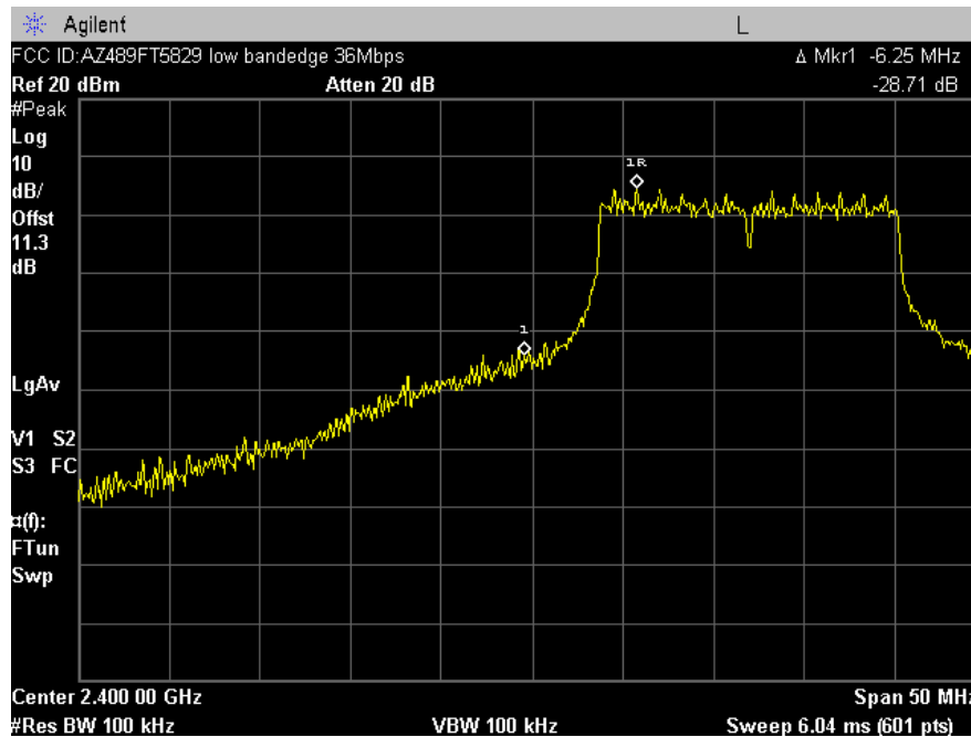
Plot A-15. Occupied Band Edge Plot – Ch. 01 – 36 Mbps
