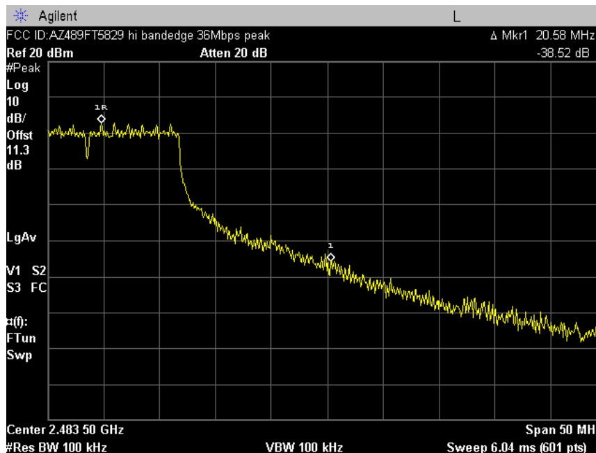
Plot A-16. Occupied Band Edge Plot – Ch. 11 – 36 Mbps
