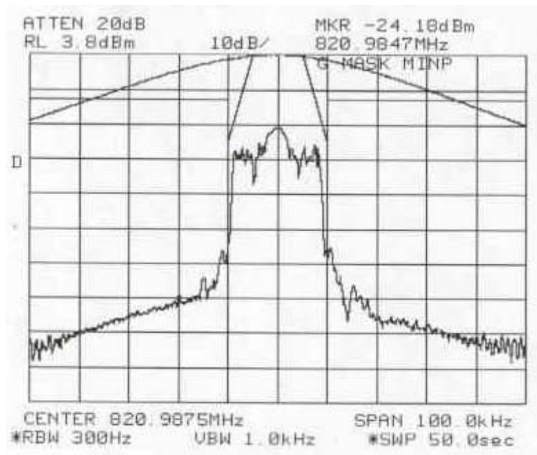
Figure 6-10b: Quad-16QAM Modulation performance relative to mask 47 CFR 90.210(g) (MINIMUM POWER SETTING) (Split 3:1 Interleaving)
