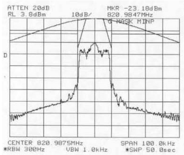
Figure 6-10a: Quad-16QAM Modulation performance relative to mask 47 CFR 90.210(g) (MINIMUM POWER SETTING)
