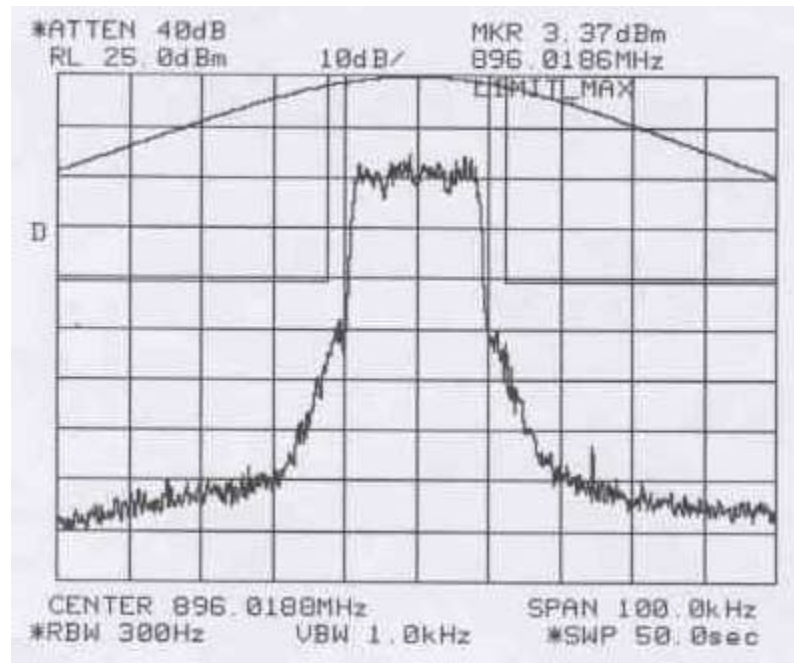
Figure 6-19b: Quad-16QAM Modulation performance relative to mask 47 CFR 90.669(a)
