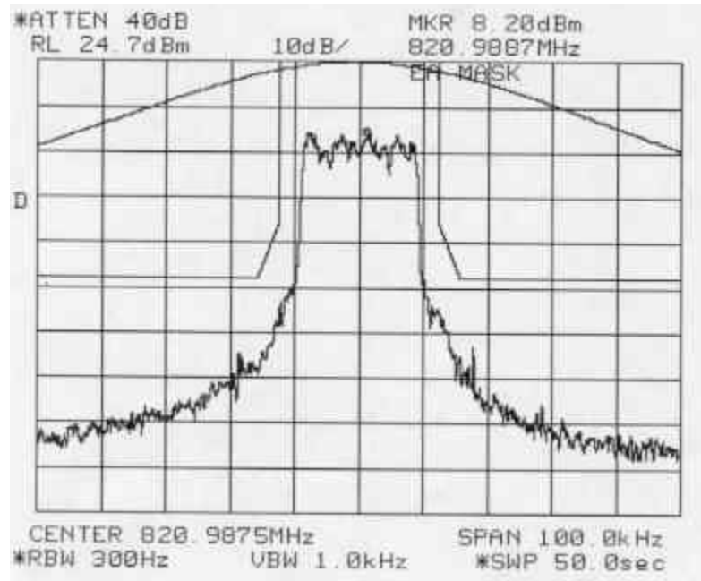
Figure 6-7: Quad-QPSK Modulation performance relative to mask 47 CFR 90.691. (MAXIMUM POWER SETTING)
