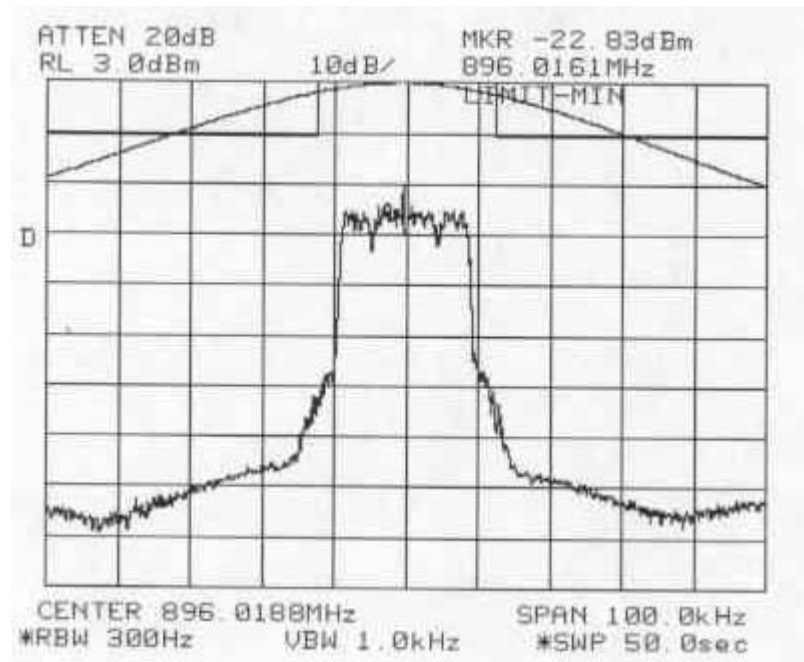
Figure 6-20a: Quad-16QAM Modulation performance relative to mask 47 CFR 90.669(a) (MINIMUM POWER SETTING)
