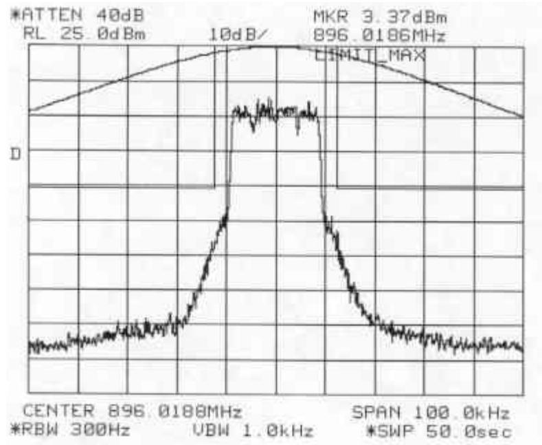
Figure 6-19a: Quad-16QAM Modulation performance relative to mask 47 CFR 90.669(a)
