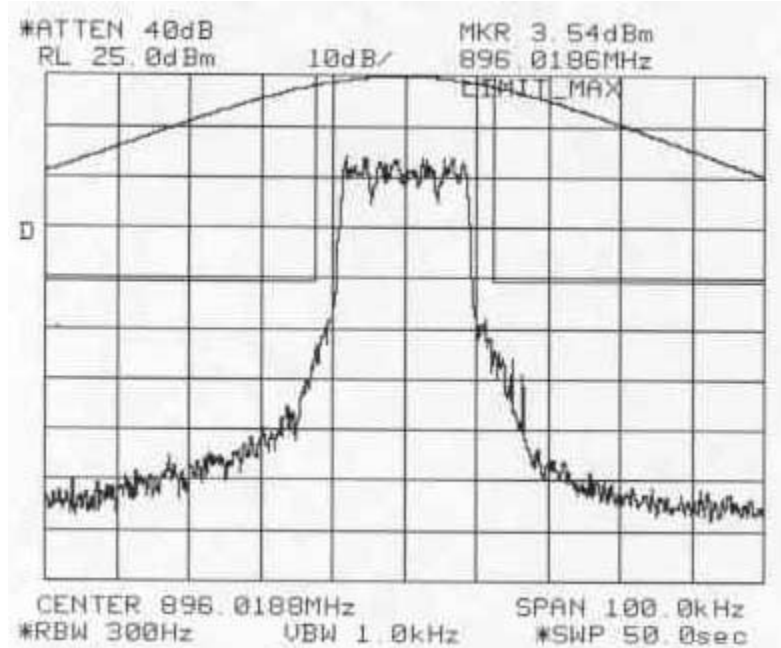
Figure 6-21: Quad-64QAM Modulation performance relative to mask 47 CFR 90.669(a) (MAXIMUM POWER SETTING)
