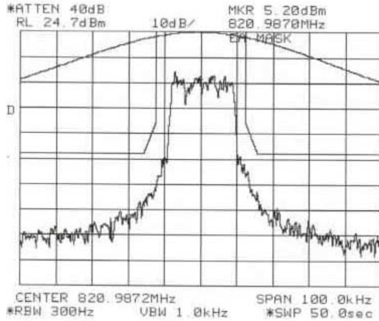
Figure 6-11a: Quad-16QAM Modulation performance relative to mask 47 CFR 90.691. (MAXIMUM POWER SETTING)
