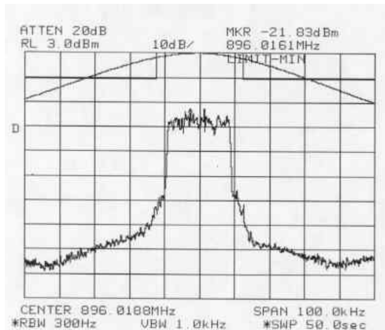
Figure 6-22: Quad-64QAM Modulation performance relative to mask 47 CFR 90.669(a) (MINIMUM POWER SETTING)
