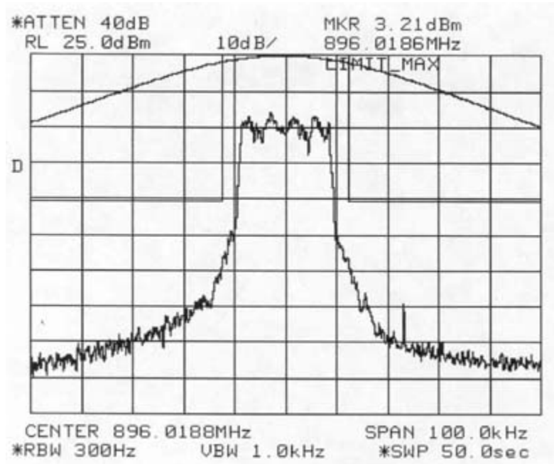
Figure 6-17: Quad-QPSK Modulation performance relative to mask 47 CFR 90.669(a) (MAXIMUM POWER SETTING)
