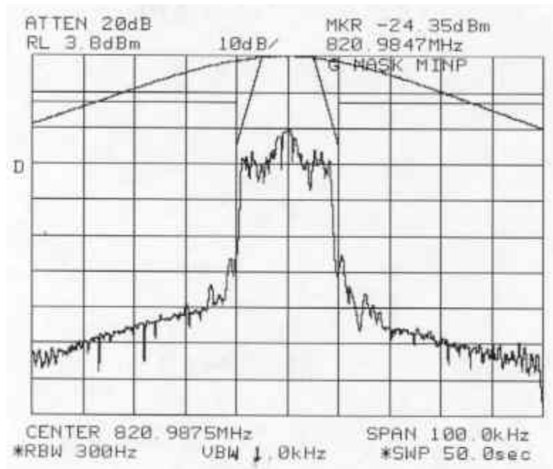
Figure 6-6: Quad-QPSK Modulation performance relative to mask 47 CFR 90.210(g) (MINIMUM POWER SETTING)
