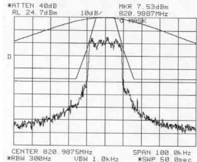
Figure 6-5: Quad-QPSK Modulation performance relative to mask 47 CFR 90.210(g) (MAXIMUM POWER SETTING)
