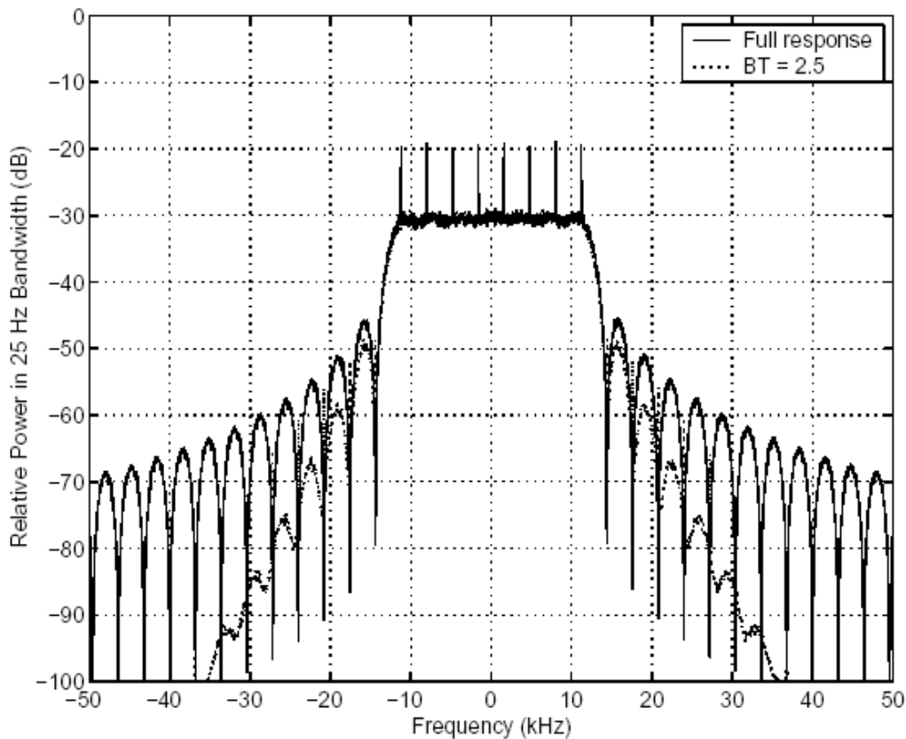
Figure 6-24. Compares the full response of the 8FSK Spectrum vs. the filtered version.
