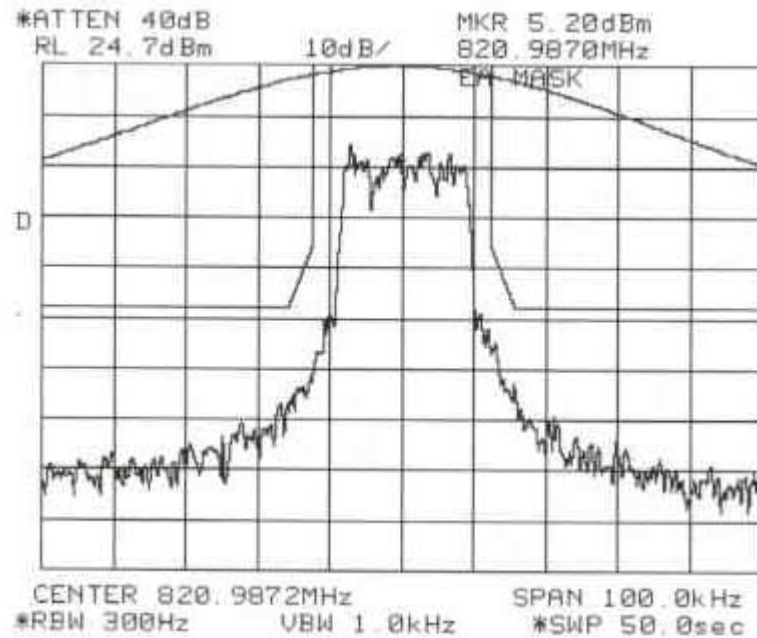
Figure 6-11b: Quad-16QAM Modulation performance relative to mask 47 CFR 90.691. (MAXIMUM POWER SETTING) (Split 3:1 Interleaving)
