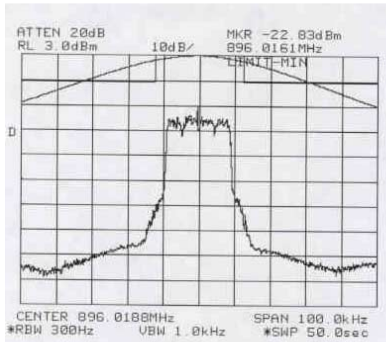
Figure 6-20b: Quad-16QAM Modulation performance relative to mask 47 CFR 90.669(a) (MINIMUM POWER SETTING) (Split 3:1 Interleaving)
