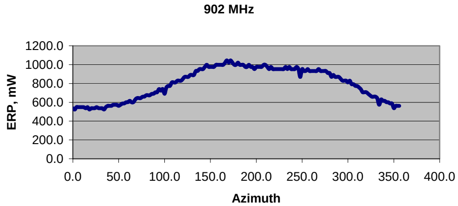
Figure 6-40. ISM Band: Scaled Maximum ERP vs. Azimuth Angle
