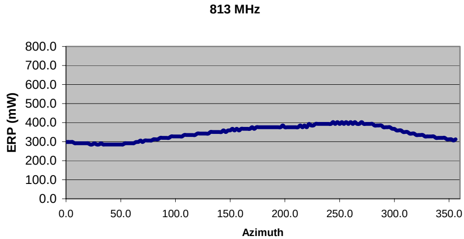
Figure 6-38: Land mobile Band: Scaled Maximum ERP vs. Azimuth Angle
