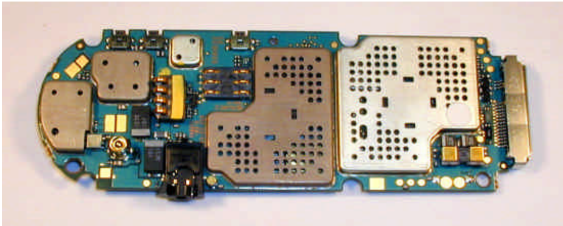
Figure 5-1. Internal photo with shields intact.
