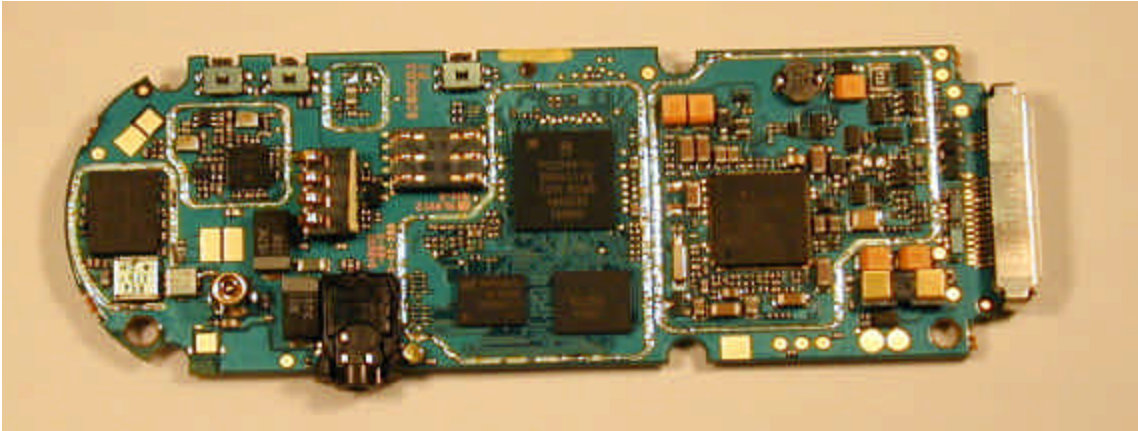
Figure 5-4. Internal photo of electronic assembly with shields removed.
