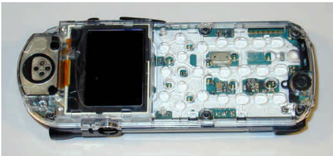
Figure 5-3. Internal photo showing the keypad and display.
