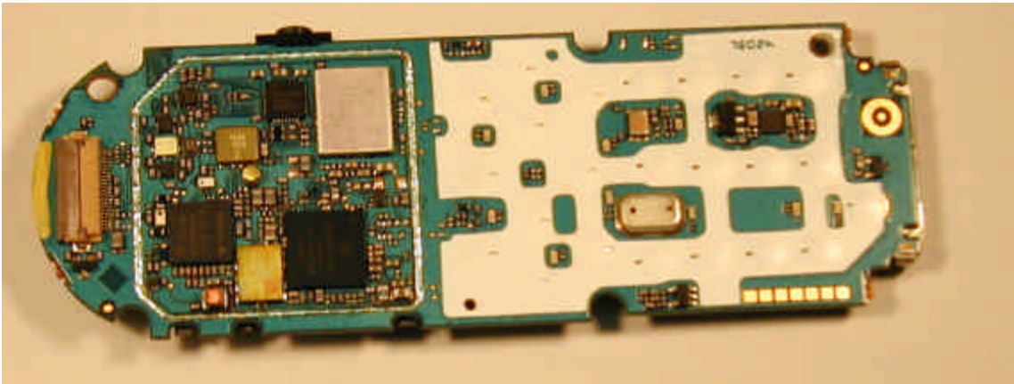
Figure 5-5. Internal photo of electronic assembly with shields removed.
