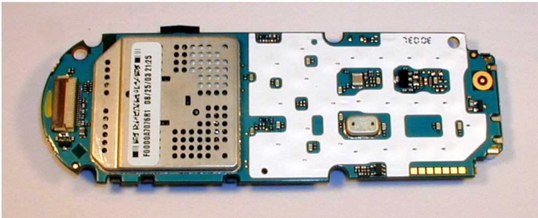
Figure 9-2. Internal photo with shields intact.
