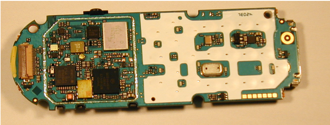
Figure 9-5. Internal photo of electronic assembly with shields removed.
