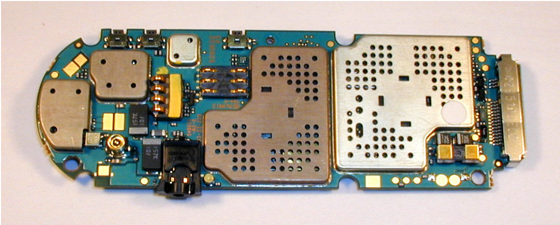
Figure 9-1. Internal photo with shields intact.
