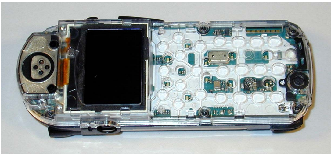
Figure 9-3. Internal photo showing the keypad and display.
