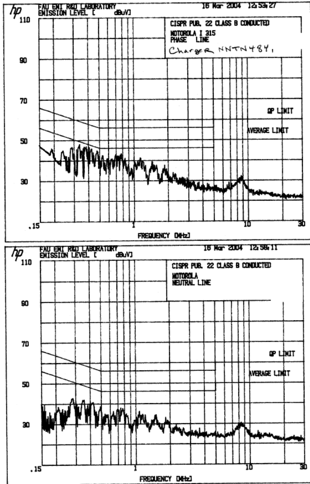
Figure 6-37: Phase and Neutral Line Voltage with a Peak and Average Detector (Radio in transmit mode at 806.0625 MHz)
