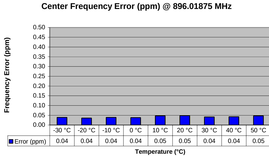
Figure 6-34: Transmitter Frequency Stability (900 MHz band) – Frequency Error vs. Temperature
