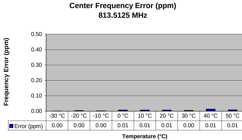
Figure 6-32: Transmitter Frequency Stability (800 MHz band) – Frequency Error vs. Temperature
