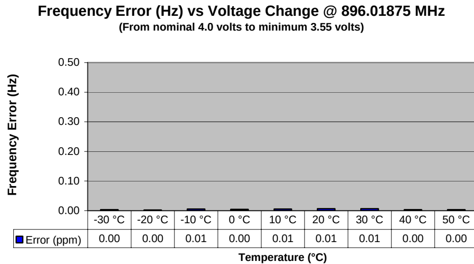
Figure 6-35: Transmitter Frequency Stability (900 MHz band) - Frequency Error vs. Voltage
