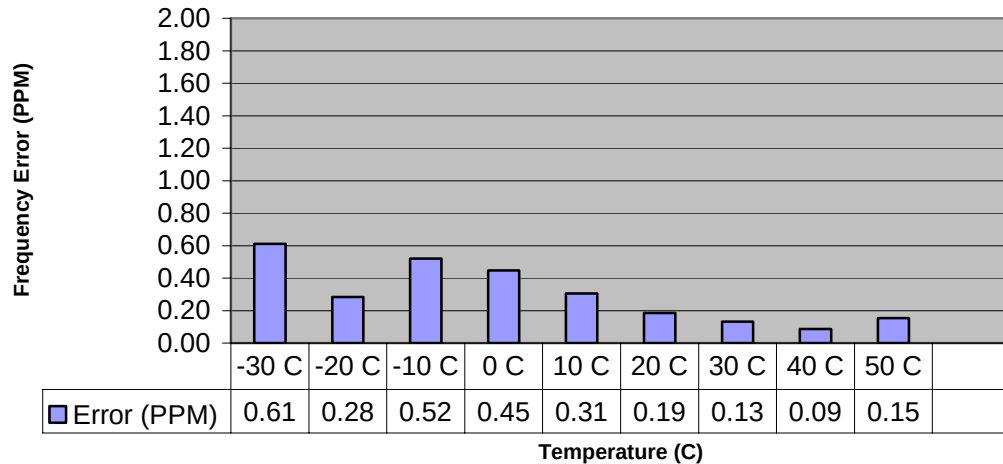
Figure 6-36: Transmitter Frequency Stability (900 MHz ISM band)- Frequency Error vs. Temperature and Voltage
